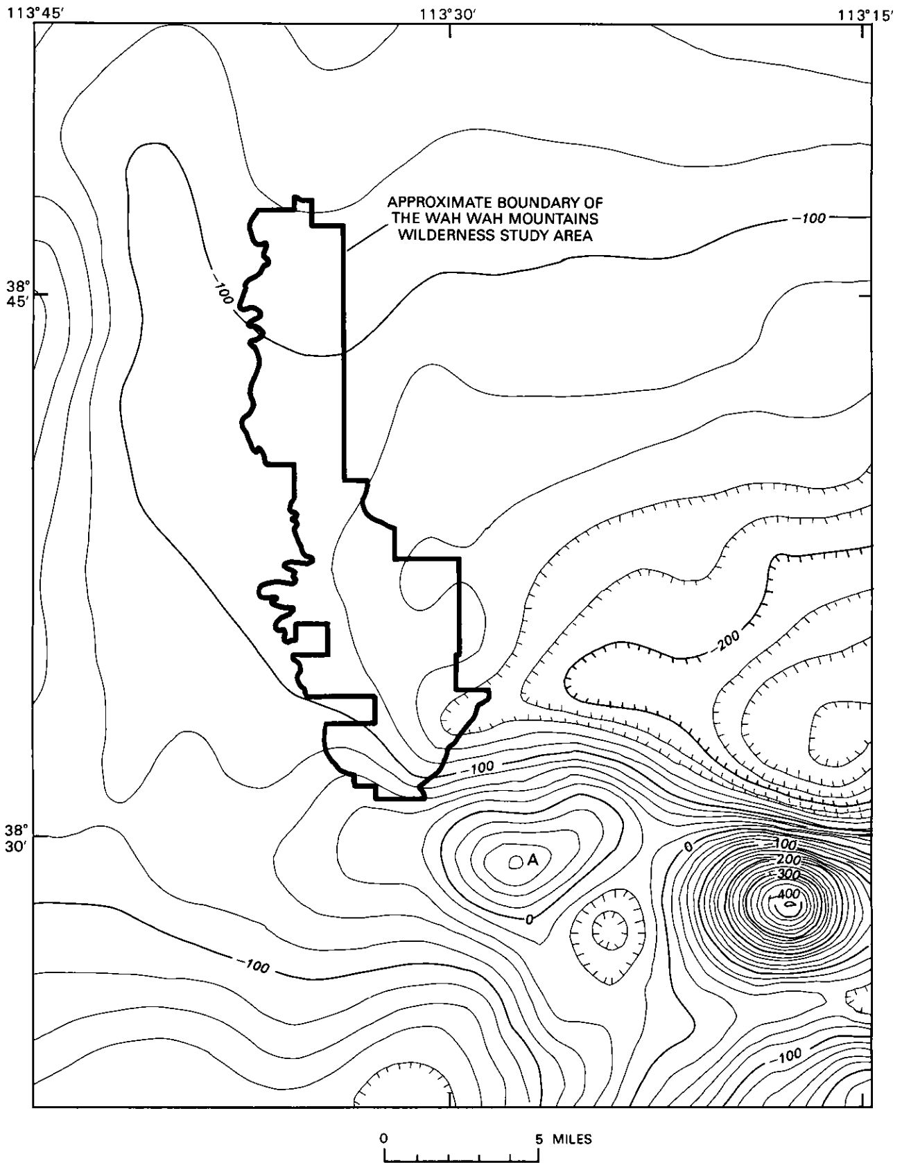
Figure 5. Aeromagnetic map of the Wah Wah Mountains Wilderness Study Area and vicinity, Utah. Contour interval, 20 nanoteslas. Hachures indicate closed areas of lower magnetic intensity. A, magnetic high discussed in text.
