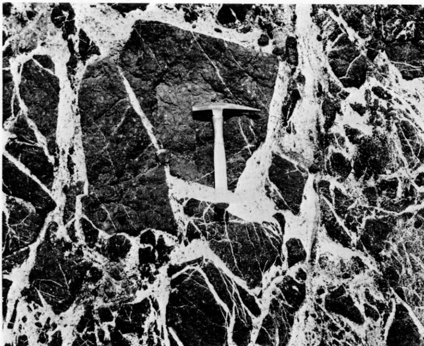
FIGURE 6.—Part of a brecciated amphibolite (agmatite) block included in migmatite, showing the intricate pattern of cementation by pegmatite. Photograph taken in sec. 32, T. 36 N., R. 106 W.
