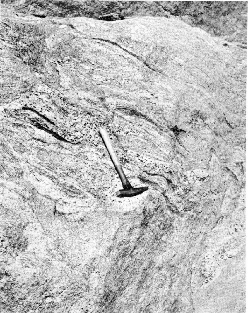
FIGURE 10.—Migmatite on Mount Quintet showing the speckled hornblende phase of the porphyritic granite injected into biotite-quartz-feldspar gneiss.
