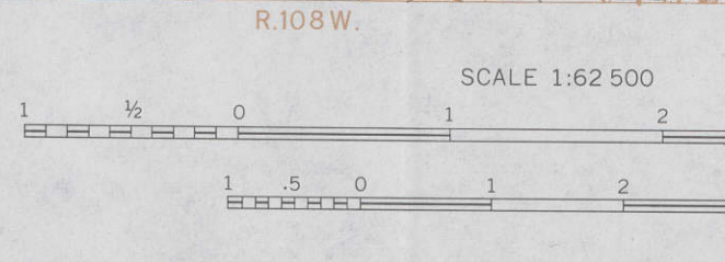
GEOLOGIC MAP OF THE GLACIER PRIMITIVE AREA, WYOMING
