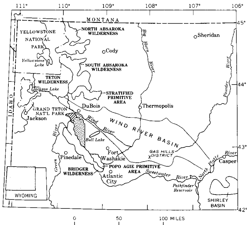
FIGURE 1.—Index map of Wyoming showing area studied: Glacier Primitive Area (stippled) and an adjacent area (hachured).
