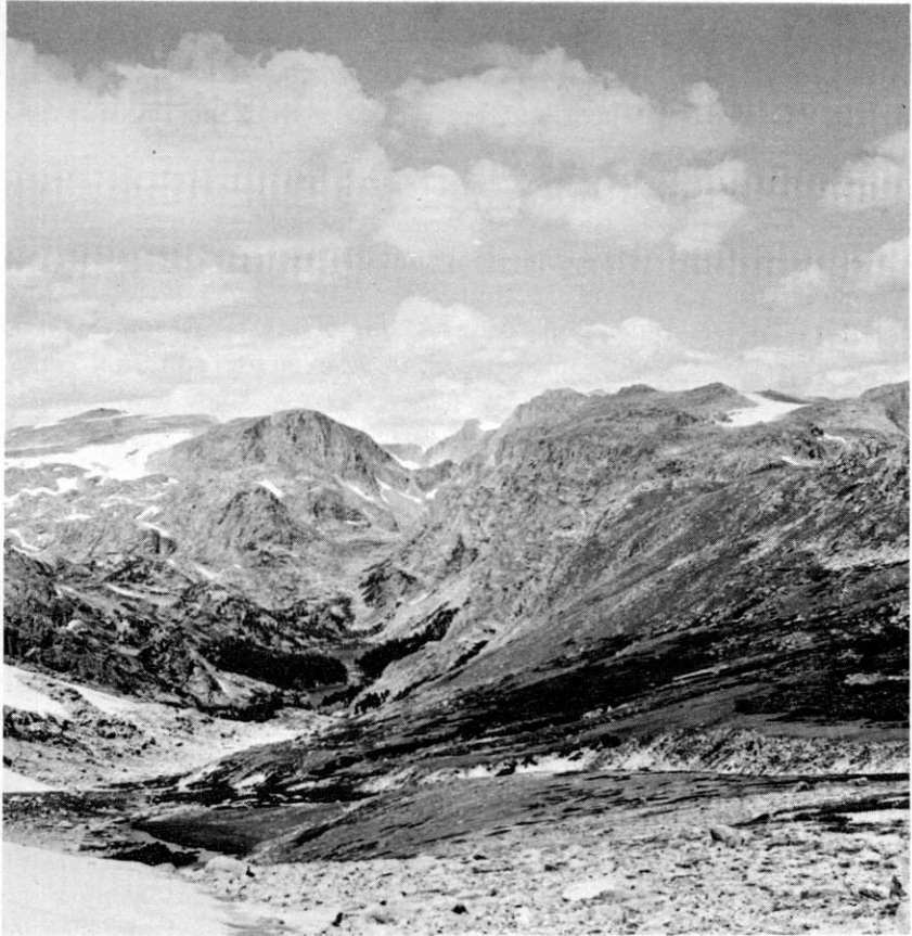
FIGURE 16.—Topographic lineament formed along the Alpine Lakes shear zone; view northwestward from the southern part of the area.
