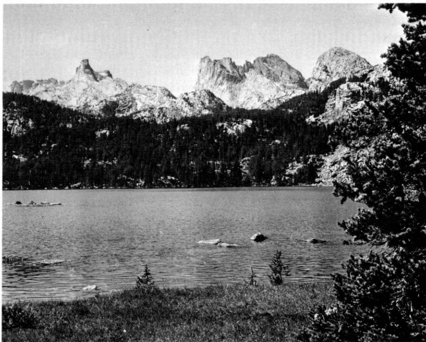
FIGURE 3.—Two prominent physiographic features: The Fortress on the left and the Brown Cliffs on the right center; view across unnamed lake in Bull Lake Creek drainage.
