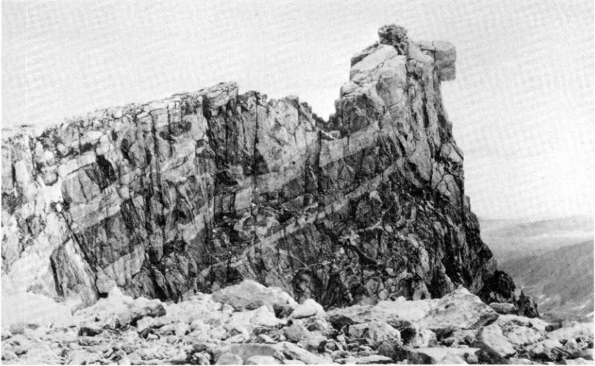
FIGURE 8.—Closeup of Chimney Rock from Horse Ridge. Light-colored gently dipping granitic dikes cut across the more steeply dipping gneissic foliation.
