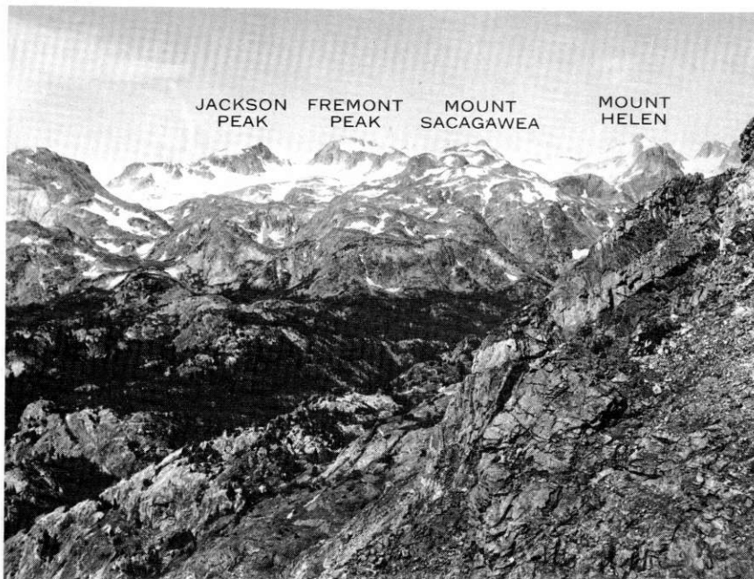
FIGURE 4.—Crest of the Wind River Range; view looking west from cliffs on the north side of Little Milky Lake. Although mapped as gneiss, the area in the foreground contains granitic and pegmatitic dikes cutting a gneissic sequence which consists principally of biotitic gneiss and includes amphibolite bodies.
