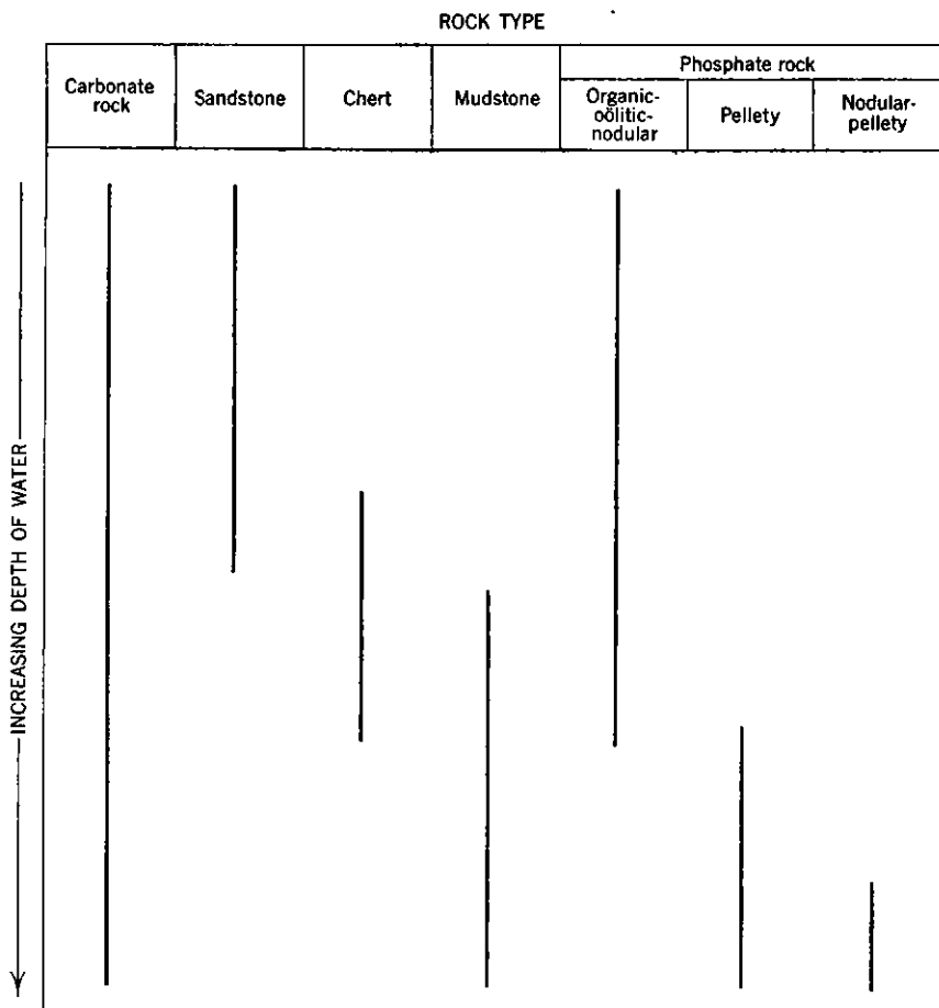
FIGURE 12.—Inferred relations between rock types in the Phosphoria formation in Montana and the relative depth of water in the depositional basin.
