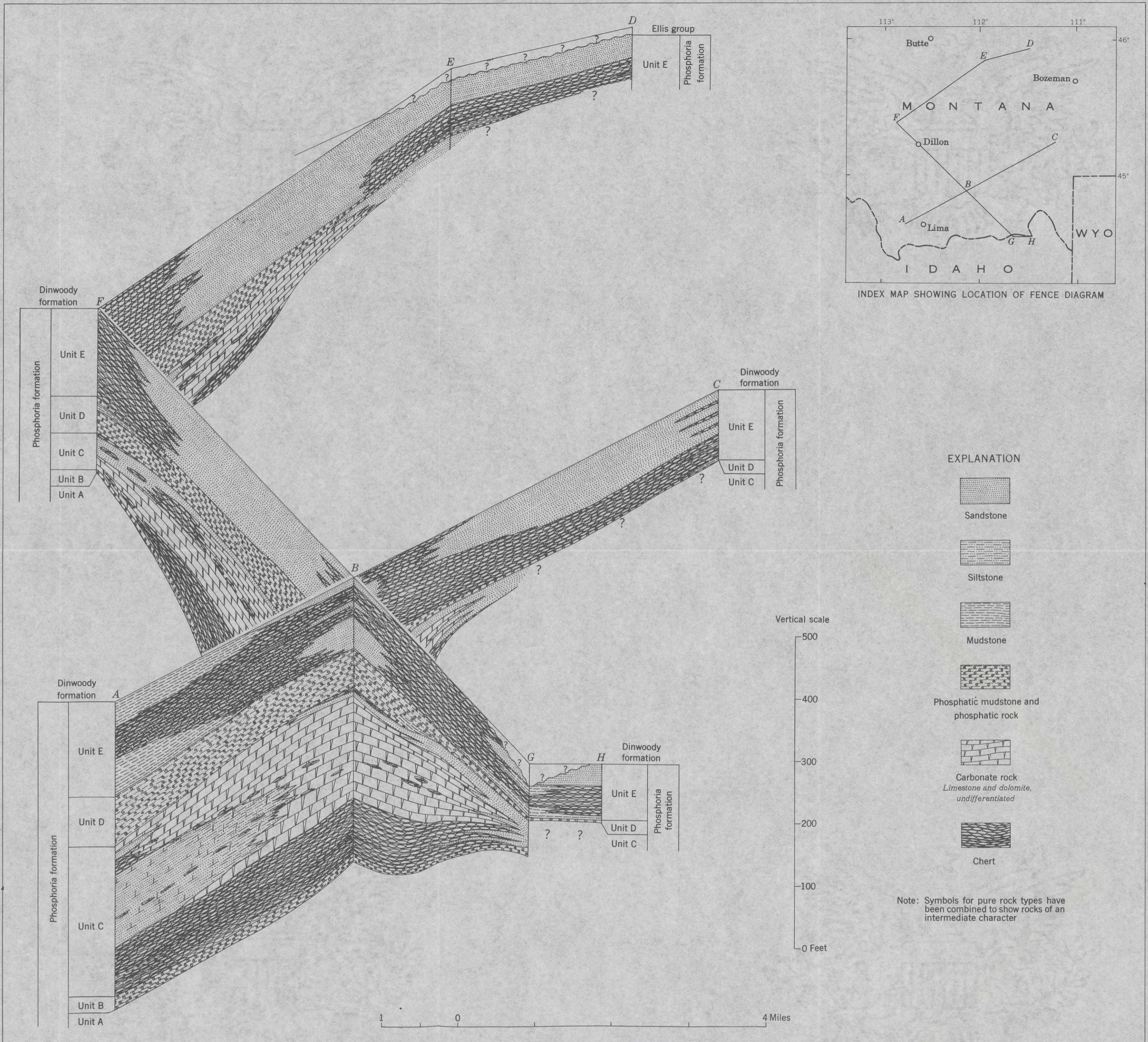
FENCE DIAGRAM SHOWING A LITHOLOGIC CORRELATION OF THE PHOSPHORIA FORMATION IN SOUTHWESTERN MONTANA
