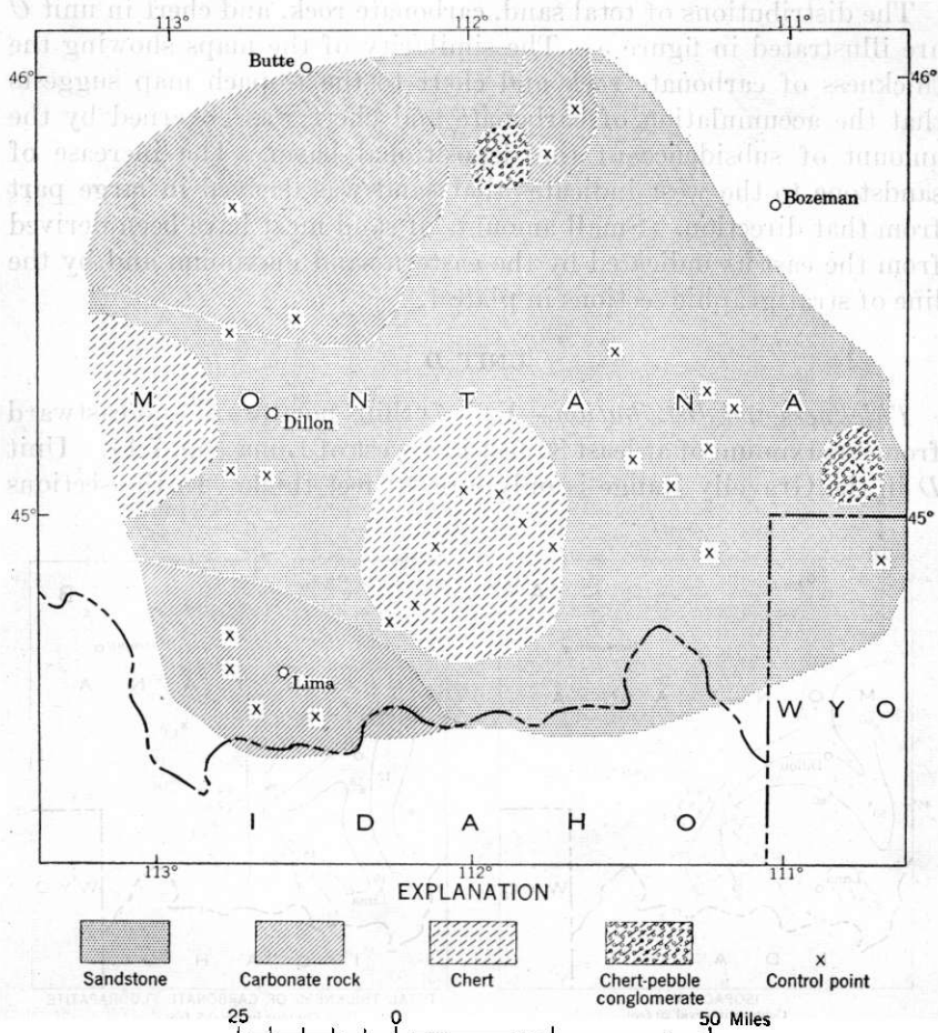
FIGURE 8.—Map showing lithologic constitution of the uppermost bed of unit C of the Phosphoria formation.
