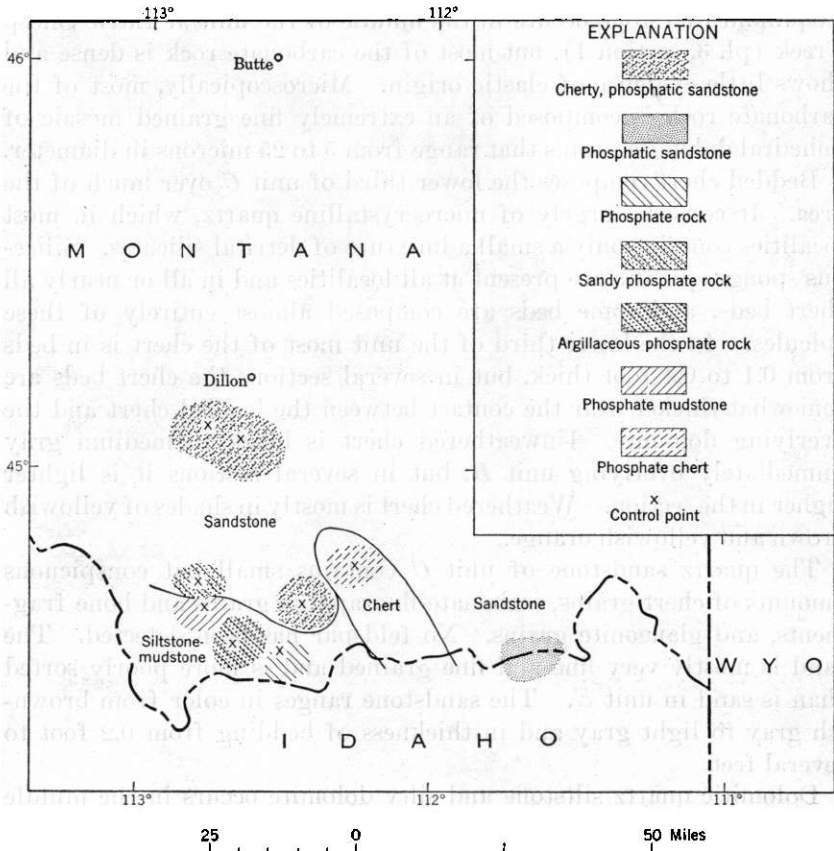
FIGURE 6.—Map showing lithologic constitution of the phosphatic bed in the lower third of unit C of the Phosphoria formation.
