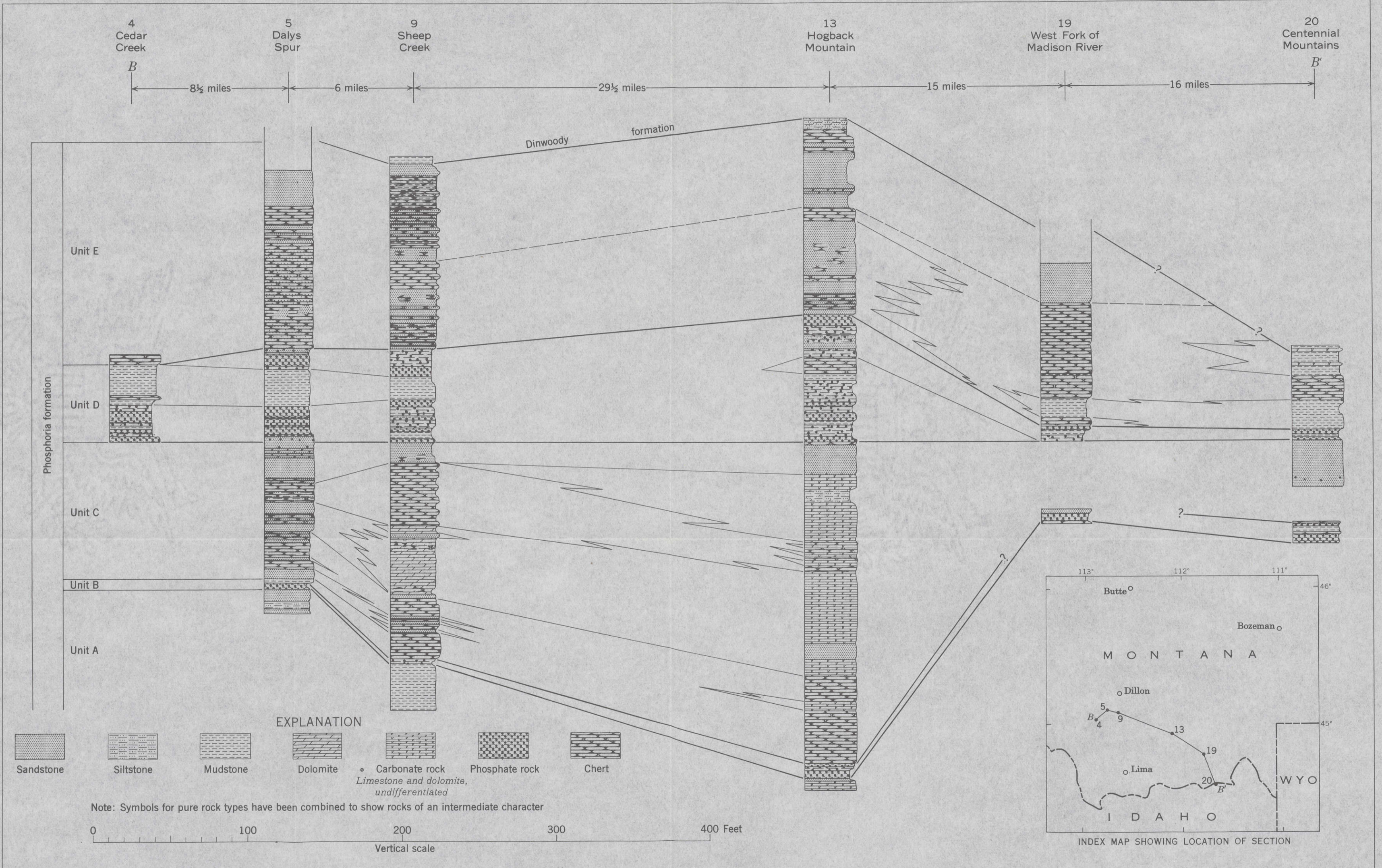
STRATIGRAPHIC SECTIONS SHOWING RELATIONS OF THE PHOSPHORIA FORMATION FROM CEDAR CREEK TO THE CENTENNIAL MOUNTAINS, MONTANA
