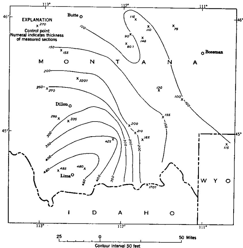
FIGURE 2.—Isopach map of the combined units B , C , D , and E of the Phosphoria formation.
