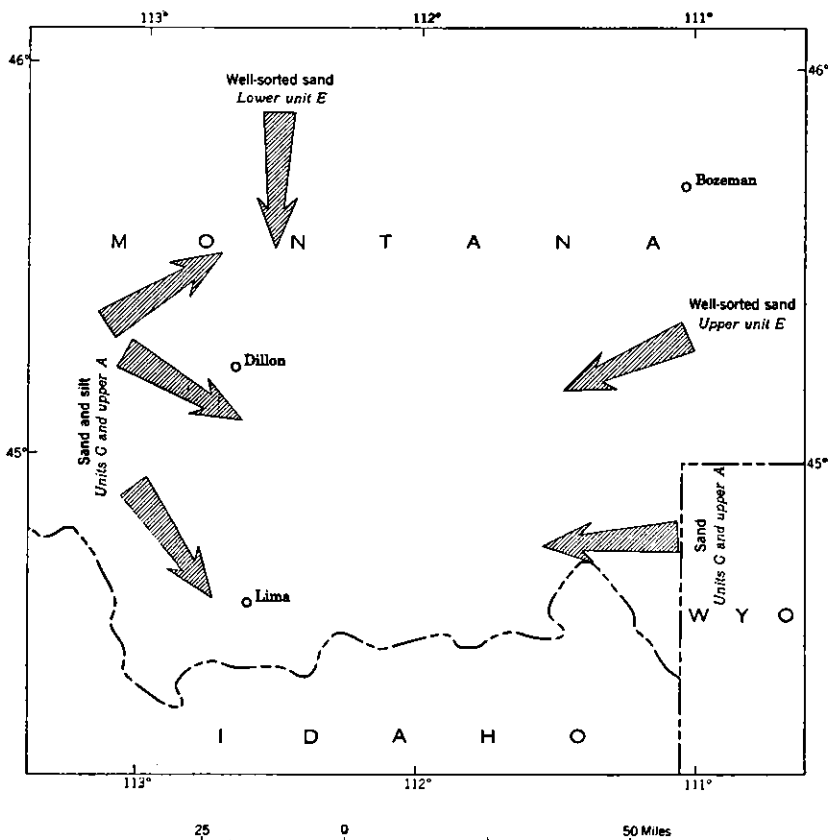
FIGURE 11.—Direction of transport of sand and silt in the Phosphoria formation.
