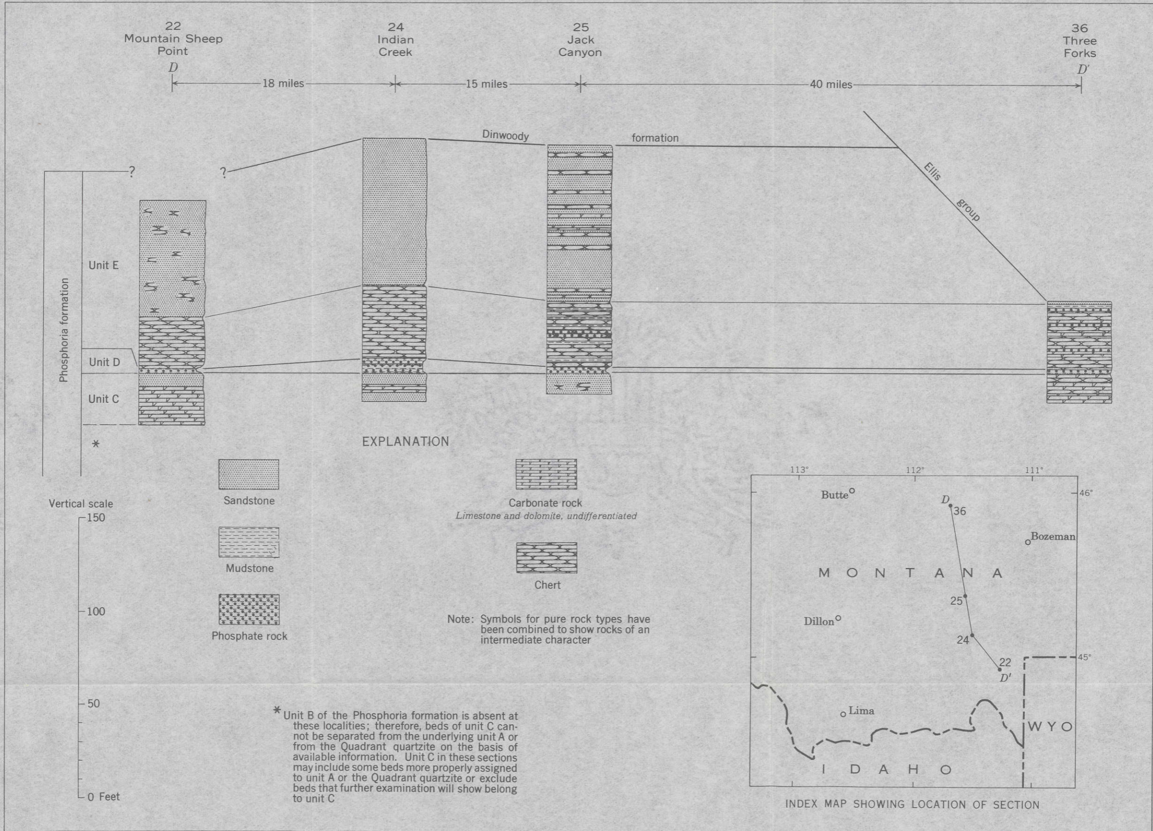
STRATIGRAPHIC SECTIONS SHOWING RELATIONS OF THE PHOSPHORIA FORMATION FROM MOUNTAIN SHEEP POINT TO THREE FORKS, MONTANA
