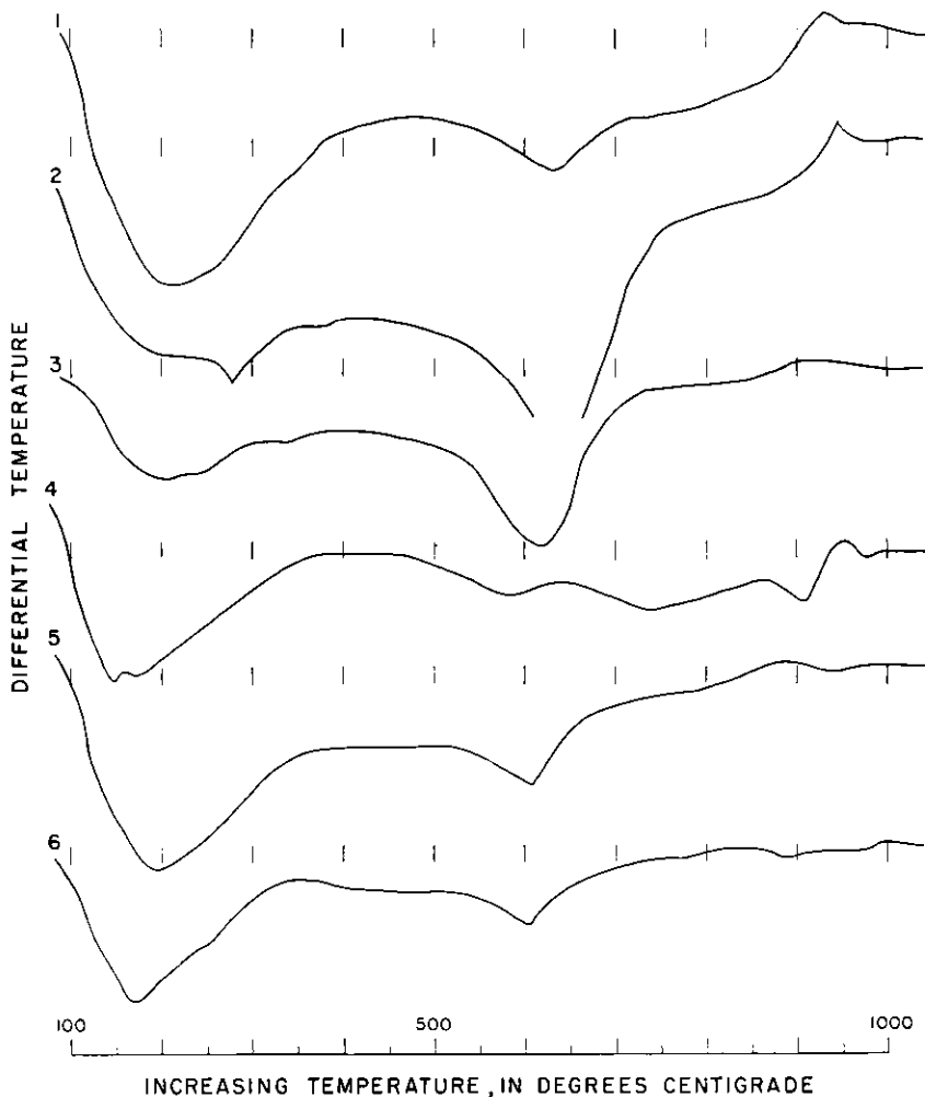
FIGURE 59.—Representative differential thermal curves of soil clays. (Thermal curve numbers correspond to soil clay numbers on facing page.)
