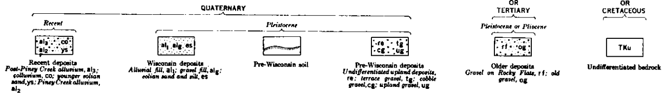
FIGURE 61.—Diagram showing stratigraphic and topographic relations of surficial deposits in the Louisville quadrangle. For full description of letter symbols see plate 7.
