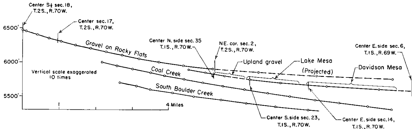
FIGURE 50.—Profiles of Rocky Flats, Davidson and Lake Mesas, Coal Creek, and South Boulder Creek. Horizontal plot was adjusted to make vertical separation correct. Altitude of projected Rocky Flats surface was computed.
