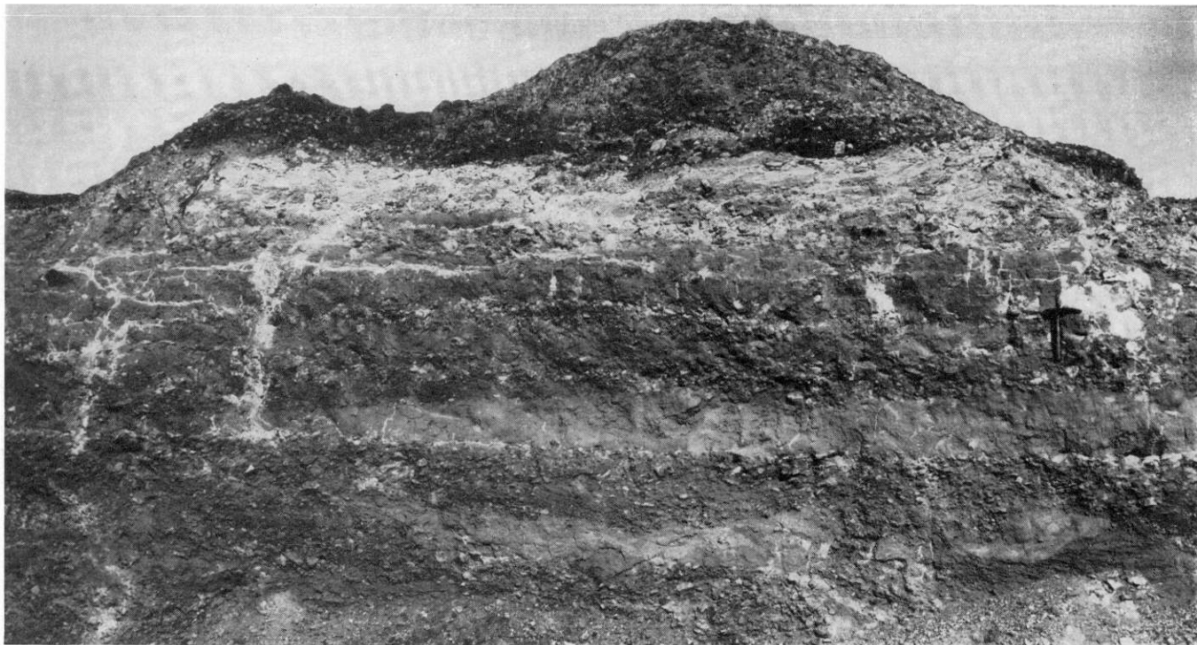
FIGURE 51.—Crossbedded gravel and sand in gravel pit on Rocky Flats in the NW \frac{1}{4} SW \frac{1}{4} sec. 23, T. 2 S., R. 70 W. (Golden quadrangle). Dark excavated material at top rests on truncated calcium carbonate layer. Nearby, a brown-red gravelly clay occurs above the carbonate layer. Calcium carbonate is most conspicuous at the top but also fills vertical joints below and is concentrated laterally at depth along contacts between gravel and sand lenses. The coarse prismatic structure and massive accumulation of carbonate near the hammer is typical of pre-Wisconsin soil development on fine-grained parent materials.
