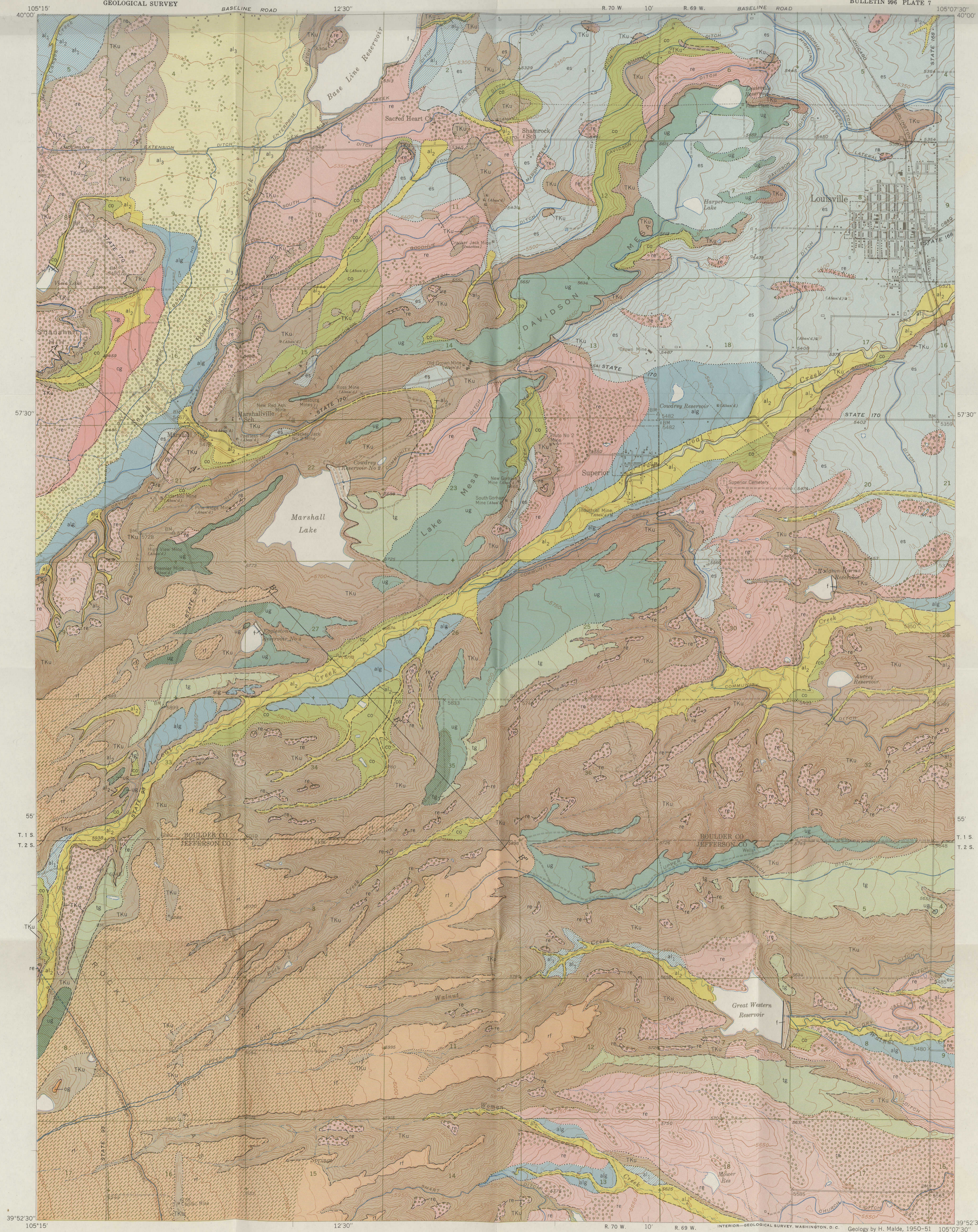
SURFICIAL GEOLOGIC MAP OF LOUISVILLE QUADRANGLE, COLORADO
