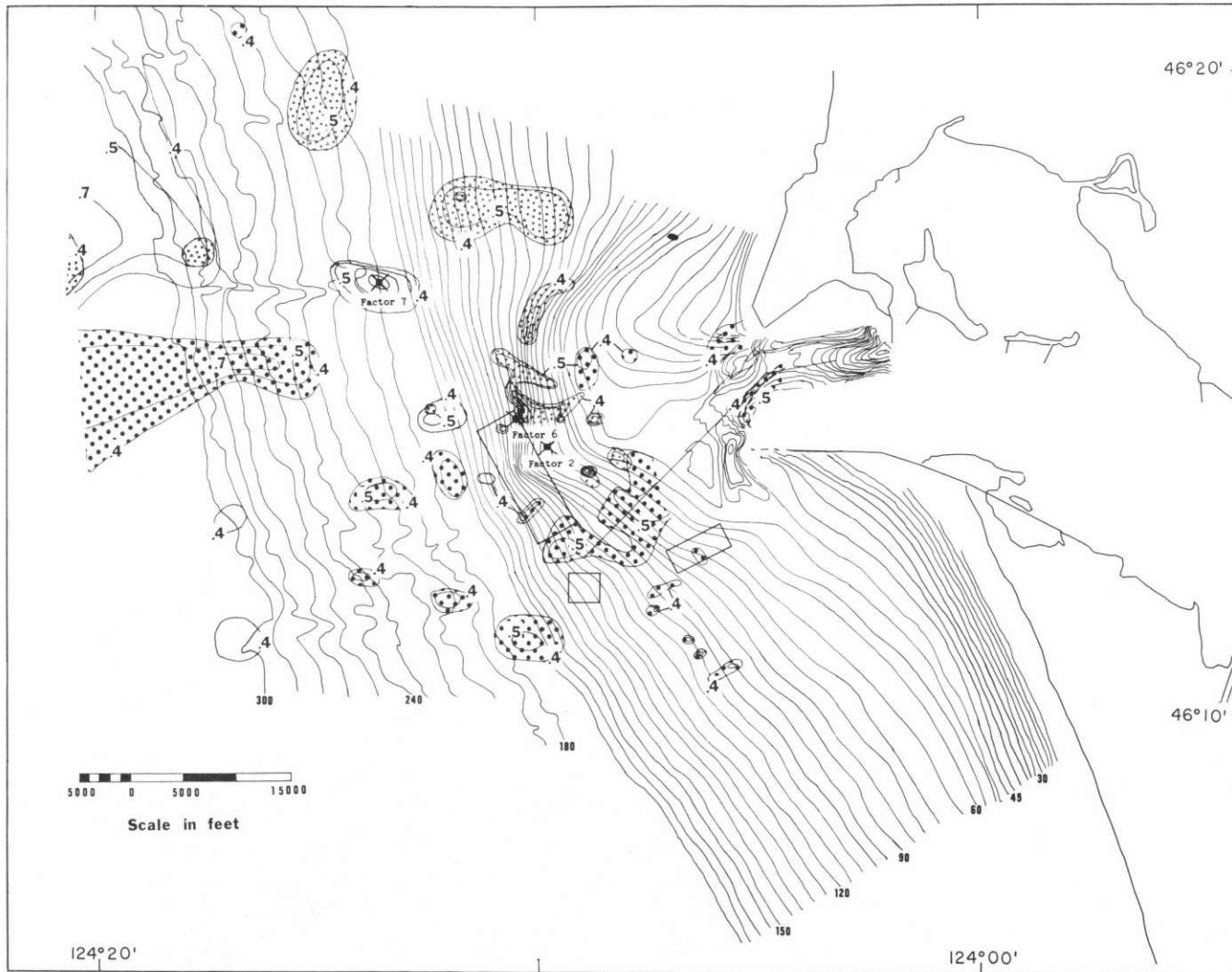
Figure A82. Areal distribution of Factor 2 (2.56 mode), Factor 6 (coarse silt, 4.56 mode), and Factor 7 (fine silt and clay, 12.0 mode) sediments. For distribution of Factors 2 and 6 in the vicinity of Disposal Site B refer to Figure A83. Locations of Factors 2, 6, and 7 extremal samples are shown (X). Disposal Sites A, B, and F and main channel entrance range line are shown for reference. Contours are in feet and the interval is variable. Key for factor loading shadings is shown in Figure A78.
