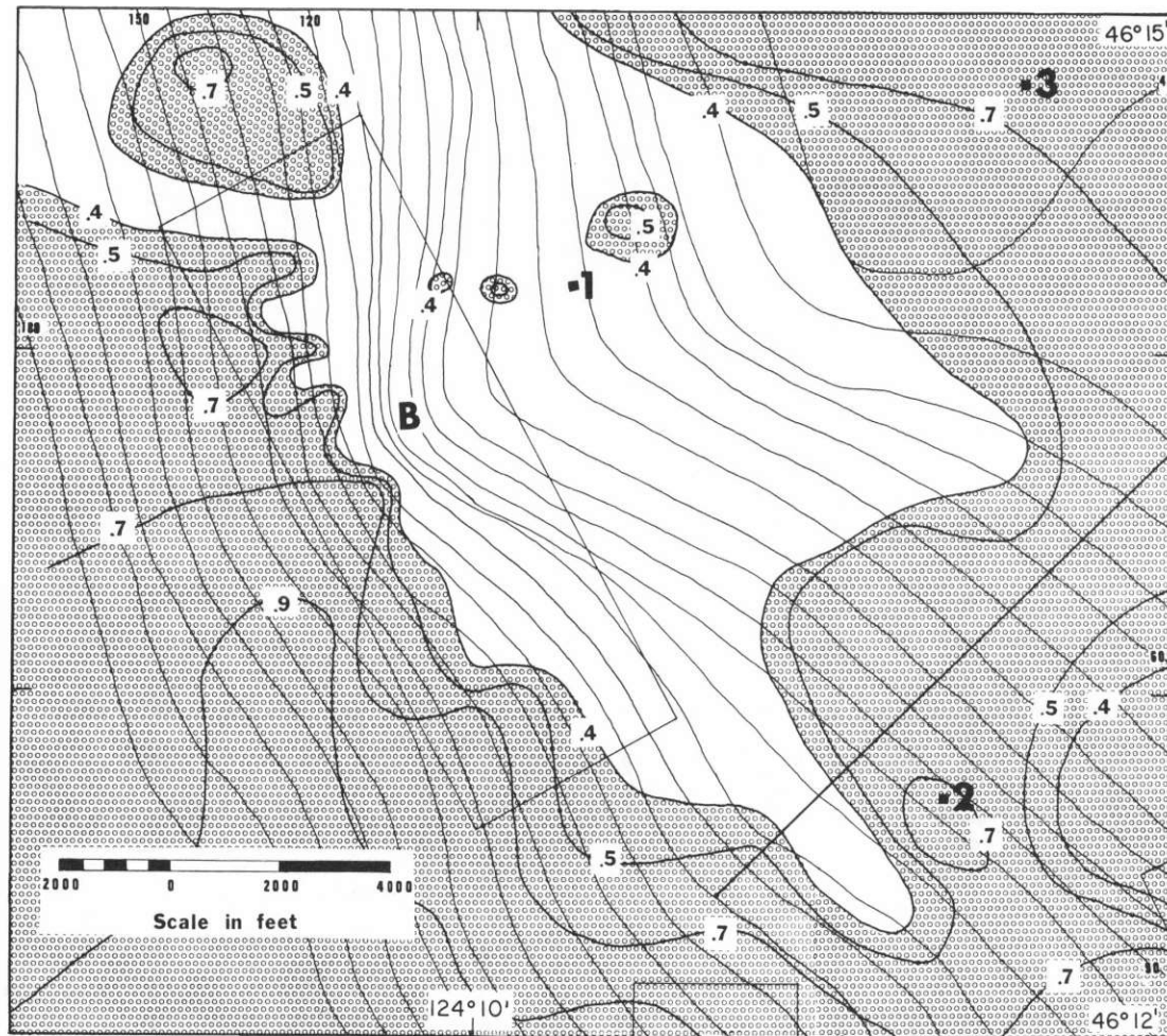
Figure A85. Areal distribution of Factor 3 (2.75 or 3.00 mode) sediments in the vicinity of Disposal Site B. Contours of loading values at 0.4, 0.5, 0.7, and 0.9. Disposal Sites A, B, and F, channel marker buoys (●), and the main channel entrance range line are shown for reference. Bathymetric contours are in feet
