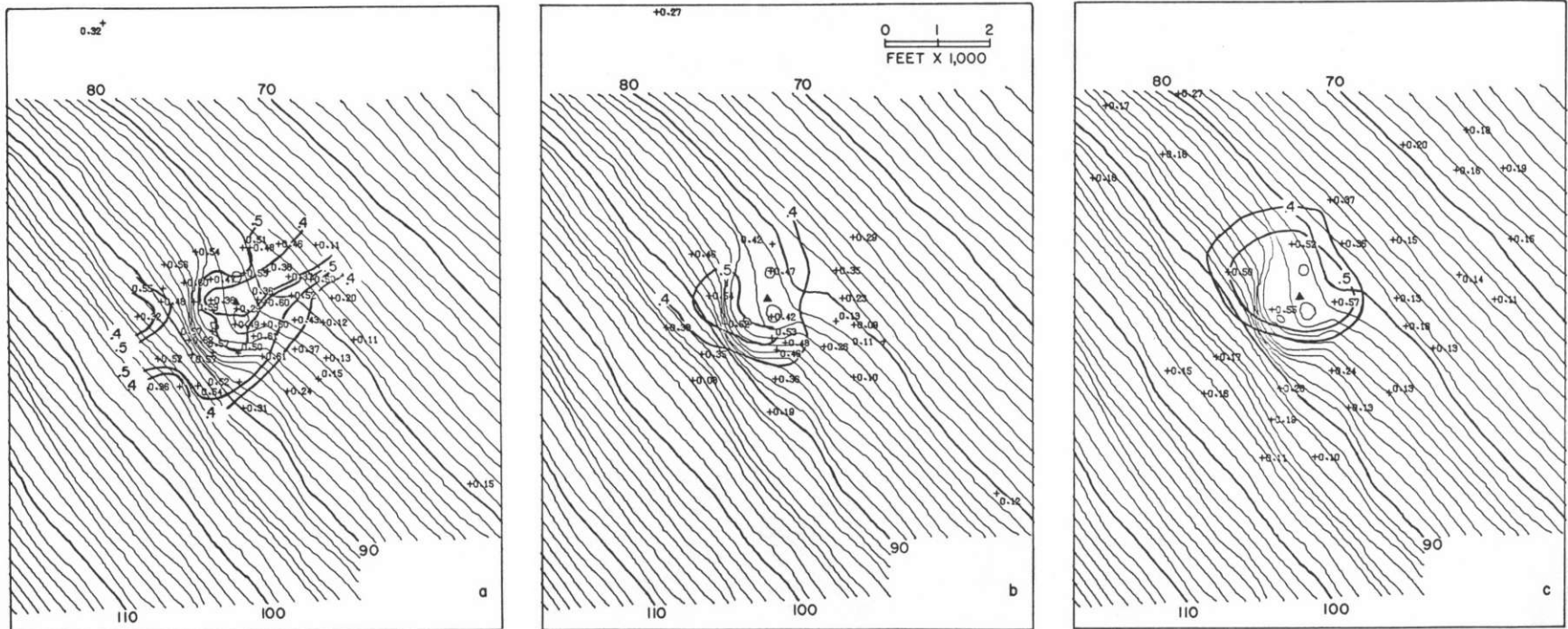
Figure A97a, b, and c. Areal distribution of Factor 2 (2.5% mode) sediment within experimental disposal Site G after the controlled disposal. Contours of loading values at 0.4, 0.5, 0.7, and 0.9. Bathymetric contours in feet. Disposal Buoy D is shown by \blacktriangle . Sample a - September 1975; b - October 1975; and c - December 1975.
