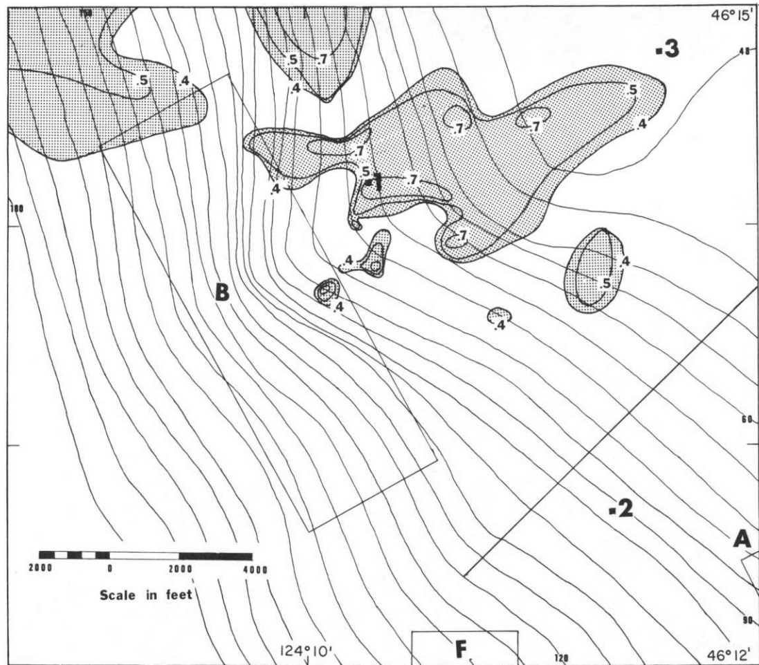
Figure A87. Areal distribution of Factor 4 (3.25 mode) sediments in the vicinity of Disposal Site B. Contours of loading values at 0.4, 0.5, 0.7, and 0.9. Disposal Sites A, B, and F, channel marker buoys (*), and main channel entrance range line are shown for reference. Bathymetric contours are in feet
