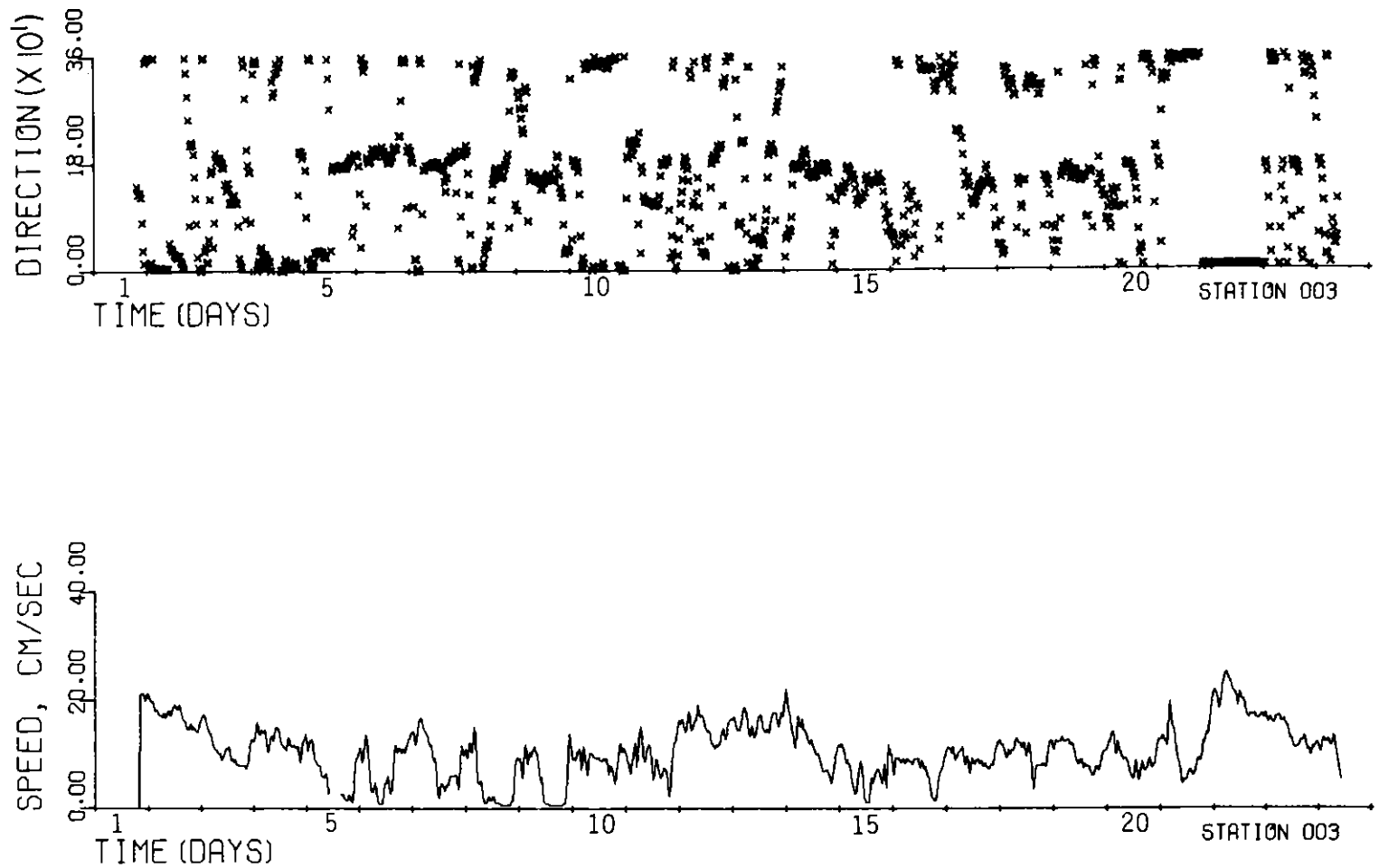
Figure A43. Bottom current speed ( \bar{U}_{100} ) and direction ( ^{\circ}T ) vs. time in days at Station 3 during the period 1930 15 00 June 75 to 1000 8 July 75. Current speed was measured 3.3 ft off the bed and all measurements were averaged over 30-min periods. These current data are summarized in Figure A44
