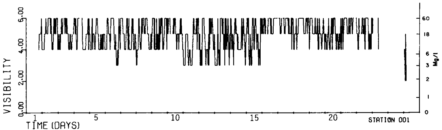
Figure A39. Photo visibility for Stations 1 and 2 during the period 1900 12 April 75 to 0800 6 May 75. The scale at the right represents concentration of suspended sediment (mg/l) 4.3 ft above the seabed (see Figure A21)
