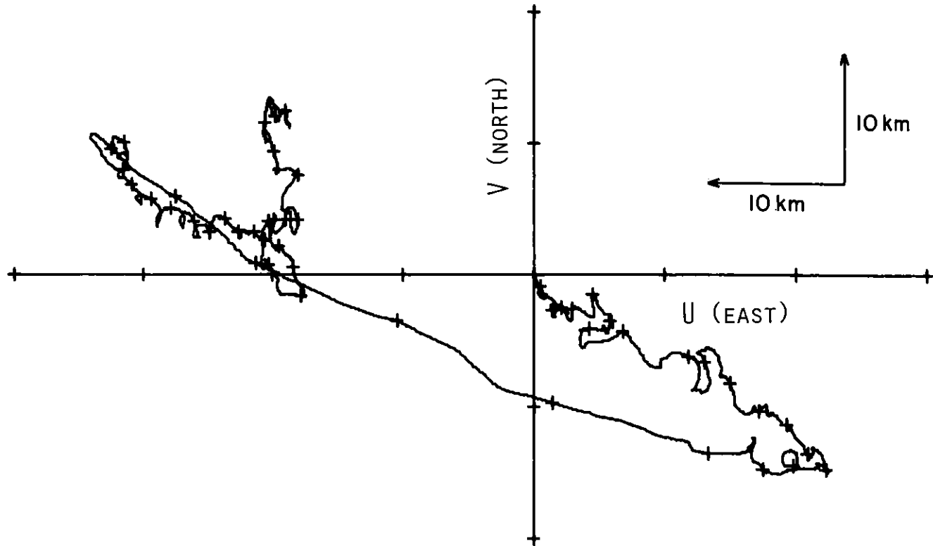
Figure A67. Progressive vector diagram (PVD) for Station 5 during the period 1300 19 August 75 to 0800 12 September 75. The positive vertical scale represents true north
