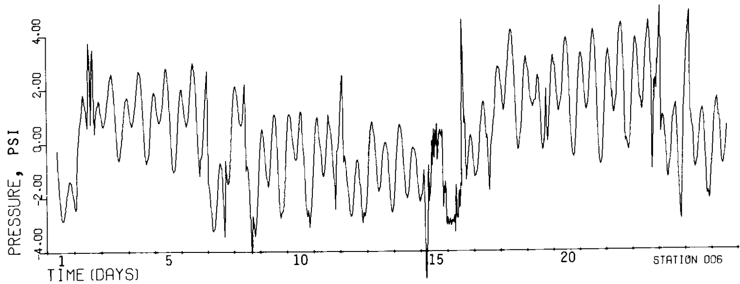
Figure A72. Tide height vs. time in days at Station 6 during the period 0900 12 December 75 to 1400 6 January 76. Mean sea level could not be established due to heavy wave activity during most of the station (see Figure A19) (1 psi ~ 2.2 ft)
