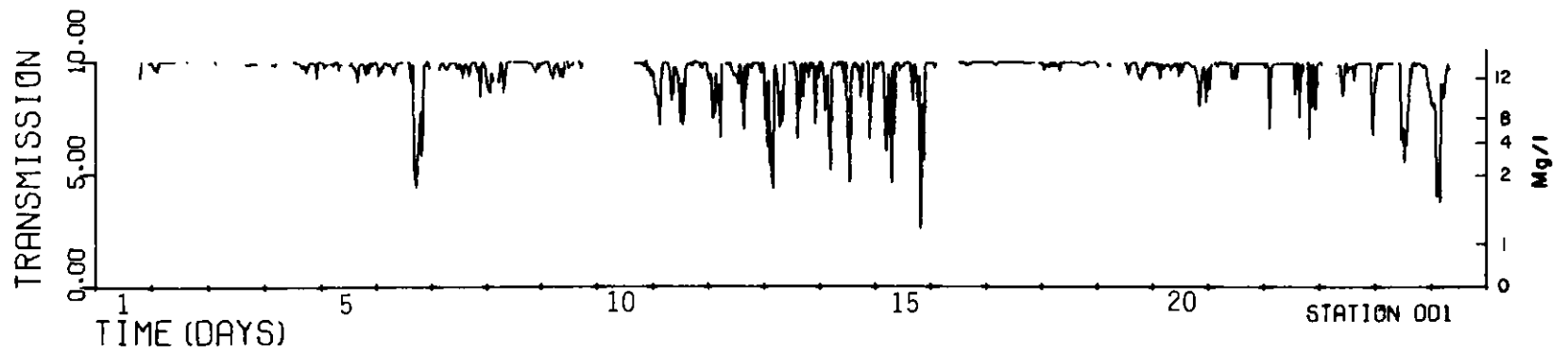
Figure A38. Transmission (in arbitrary recorder units) at Station 1 during the period 1900 12 April 75 to 0800 6 May 75. The scale at the right represents concentration of suspended sediment (mg/l) 4.3 ft above the seabed (see Figure A21)
