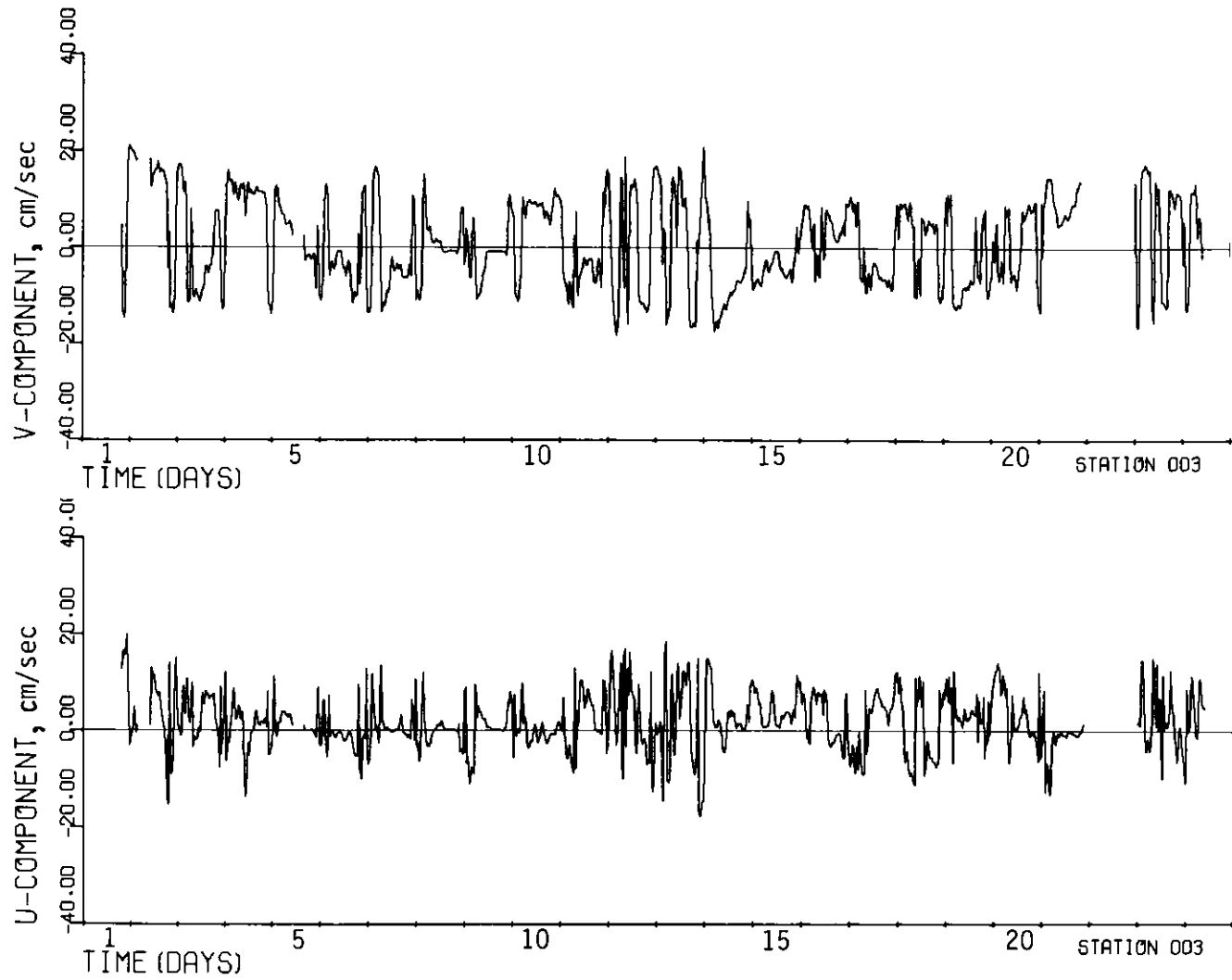
Figure A45. Northward (V) and eastward (U) components of current velocity 3.3 ft above the bed at Station 3 during the period 1930 15 June 75 to 1000 8 July 75
