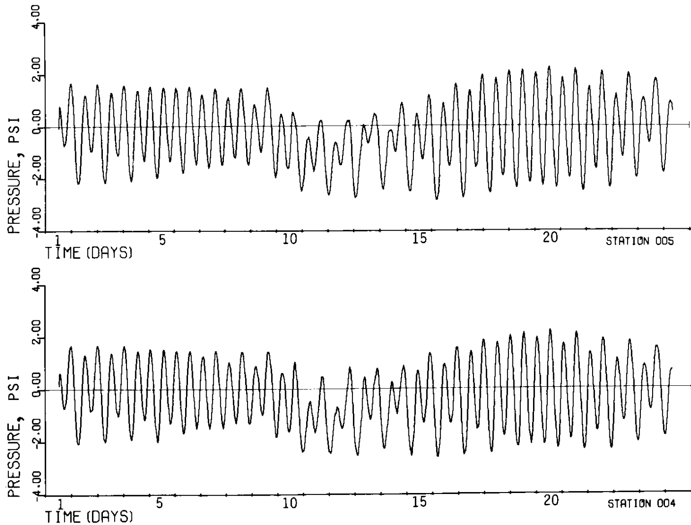
Figure A59. Tide height vs. time in days at Stations 4 and 5 during the period 1300 19 August 75 to 0800 12 September 75. The vertical scale is in psi referenced to mean sea level (1 psi ~ 2.2 ft)
