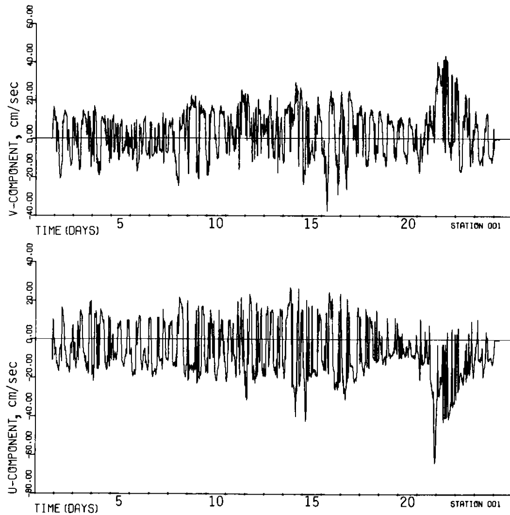
Figure A34. Northward (V) and eastward (U) components of current velocity 3.3 ft above the bed at Station I during the period 1900 12 April 75 to 0800 6 May 75
