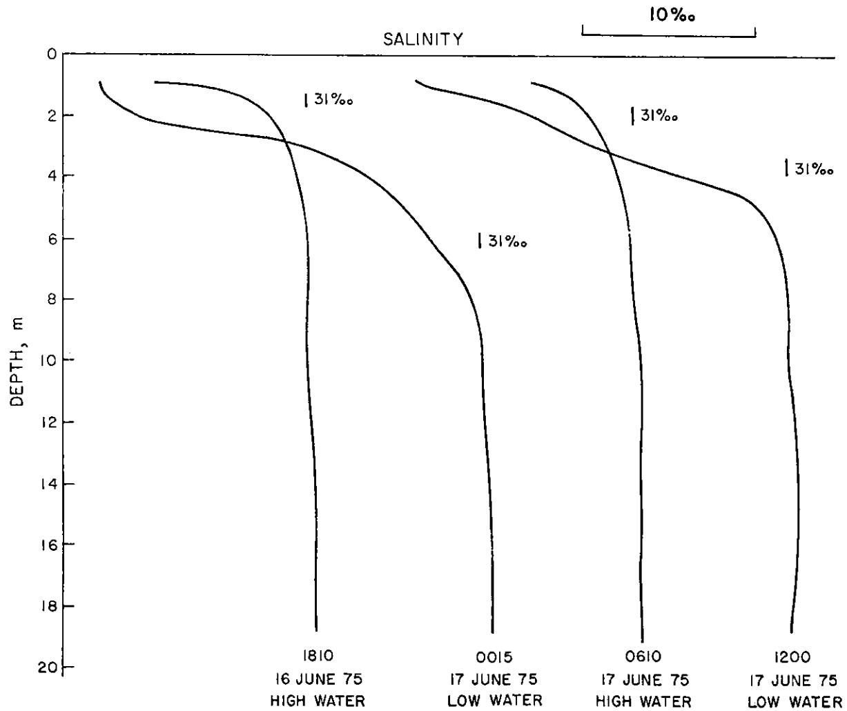
Figure A55. Salinity profiles at station Kay-3 (Site B) representing typical flood and ebb characteristics. Data were collected from 25-hr anchor stations
