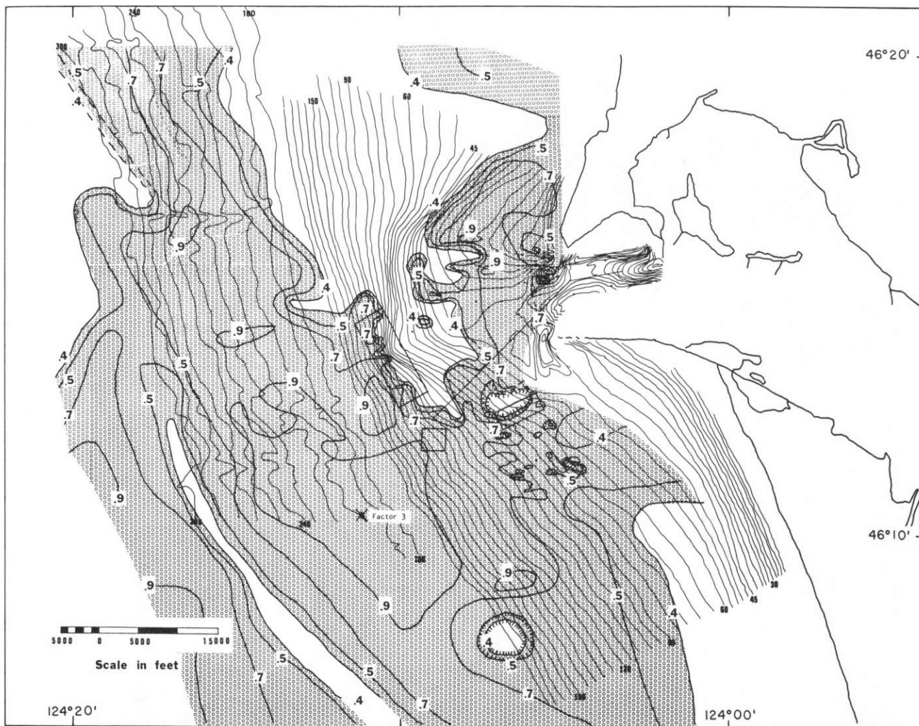
Figure A84. Areal distribution of Factor 3 (2.75 or 3.0% mode) sediment. Contours of loading values at 0.4, 0.5, 0.7, and 0.9. Location of Factor 3 extremal samples is shown (X). Disposal Sites A, B, and F and the main channel entrance range line are shown for reference. Bathymetric contours are in feet and the interval is variable. Detail in the vicinity of Disposal Site B is shown in Figure A85.
