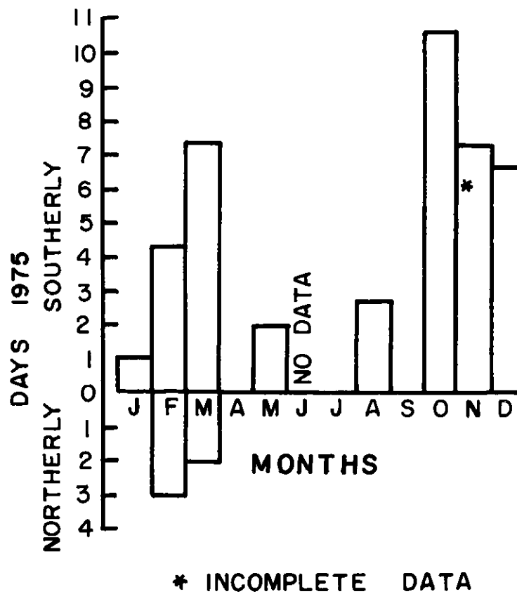
Figure A129. Frequency of time in days during each month of 1975 that mean wind speeds exceeded 10 m/sec blowing from the north or the south. Winds were measured at the Columbia River Lightship and all data were averaged for 25-hr periods prior to analysis
