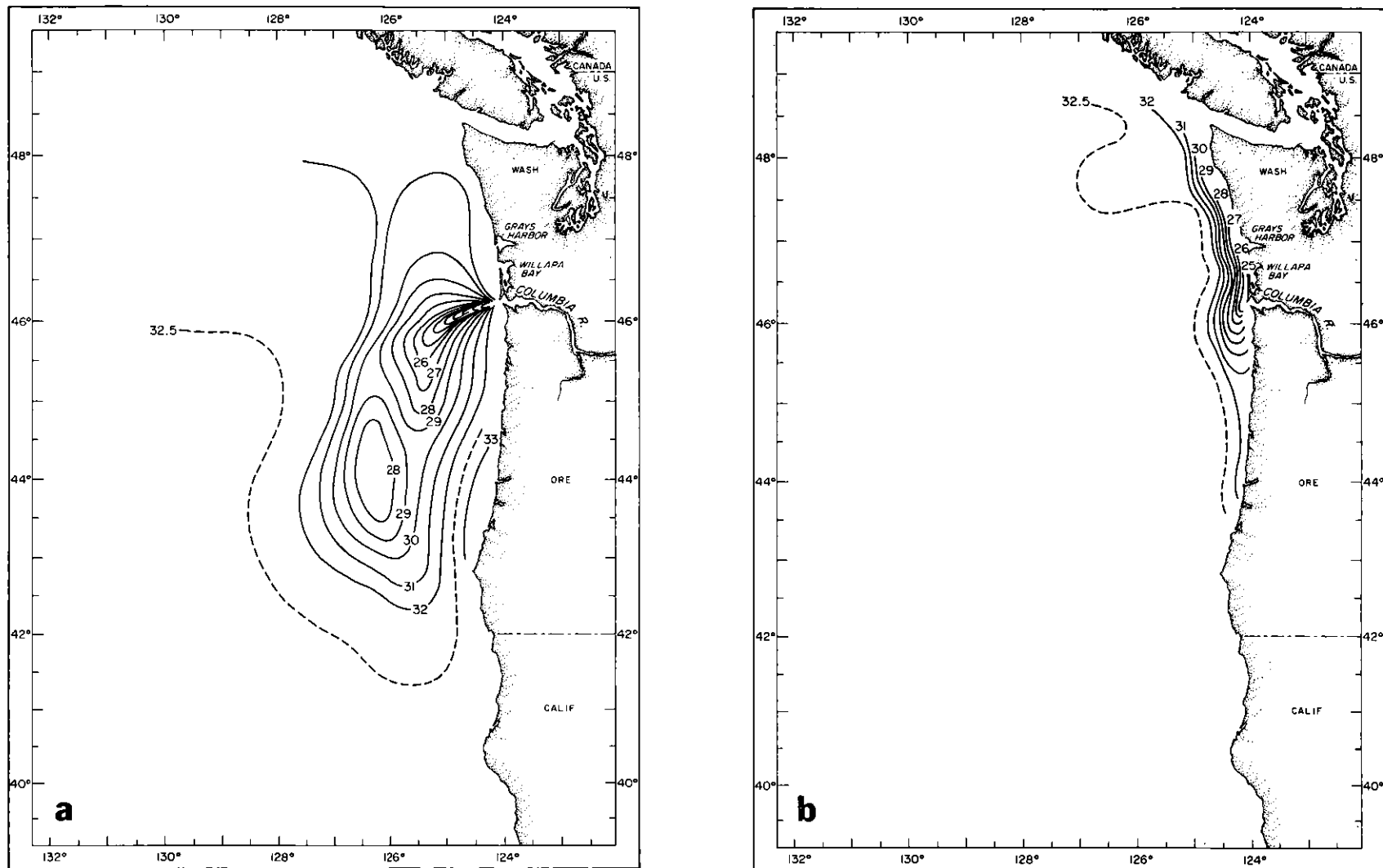
Figure A14. General surface salinity ( ^{\circ}/_{\infty} ) distribution during summer (a) and winter (b) seasons (from Duxbury, Morse and McGary 1966)
