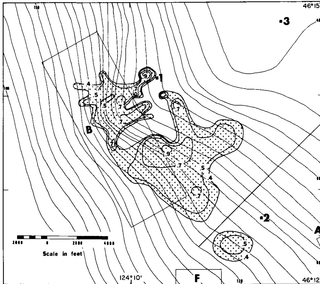
Figure A80. Areal distribution of Factor 1 (1.75, 2.0, or 2.25 modes) sediment in the vicinity of Disposal Site B. Contours of loading values at 0.4, 0.5, 0.7, and 0.9. Disposal Sites B and F, channel marker buoys (•), and the main channel entrance range line are shown for reference. Bathymetric contours are in feet
