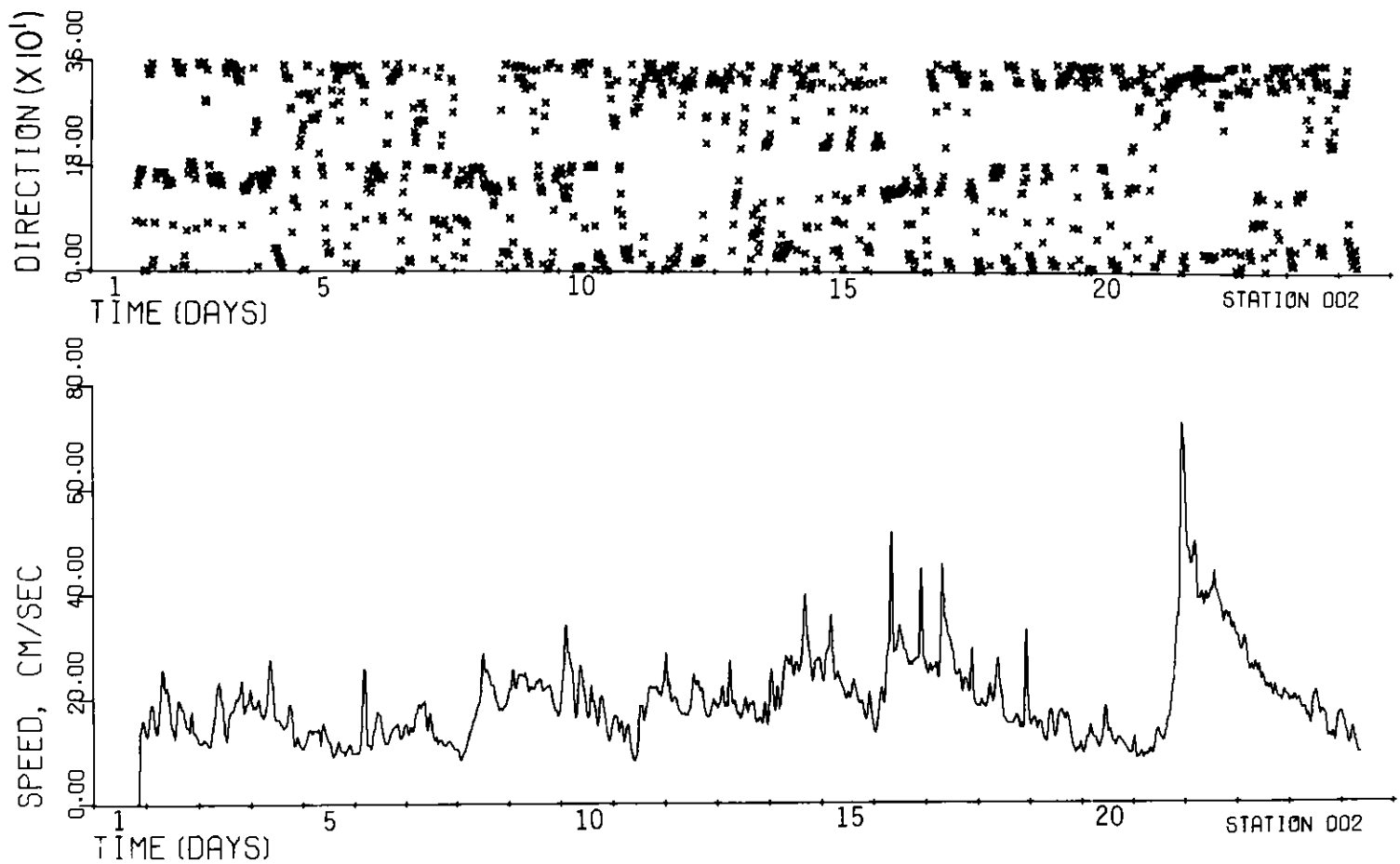
Figure A31. Bottom current speed ( \bar{U}_{100} ) and direction ( ^{\circ}T ) vs. time in days at Station 2 during the period 1900 12 April 75 to 0800 6 May 75. Current speed was measured 3.3 ft off the bed and all measurements were averaged over 30-min periods. These current data are summarized in Figure A33
