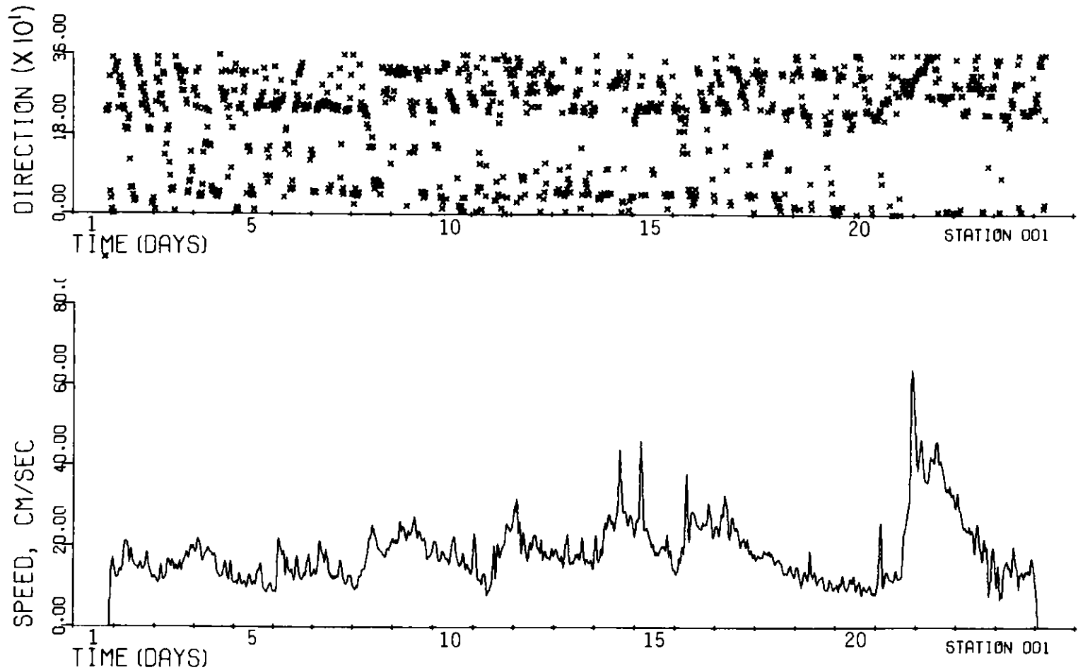
Figure A30. Bottom current speed ( \bar{U}_{100} ) and direction ( ^{\circ}T ) vs. time in days at Station 1 during the period 1900 12 April 75 to 0800 6 May 75. Current speed was measured 3.3 ft off the bed and all measurements were averaged over 30-min periods. These current data are summarized in Figure A32
