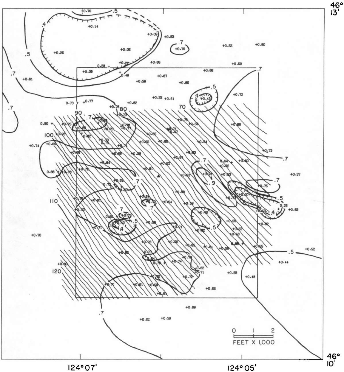
Figure A98. Areal distribution of Factor 3 (2.75 or 3.0 mode) sediment within experimental Disposal Site G before the controlled disposal. Contours of loading values at 0.4, 0.5, 0.7, and 0.9. Bathymetric contours are in feet. Disposal Buoy D is shown as ▲. (Figures 99a, b, and c are enlargements of the inner rectangular area)
