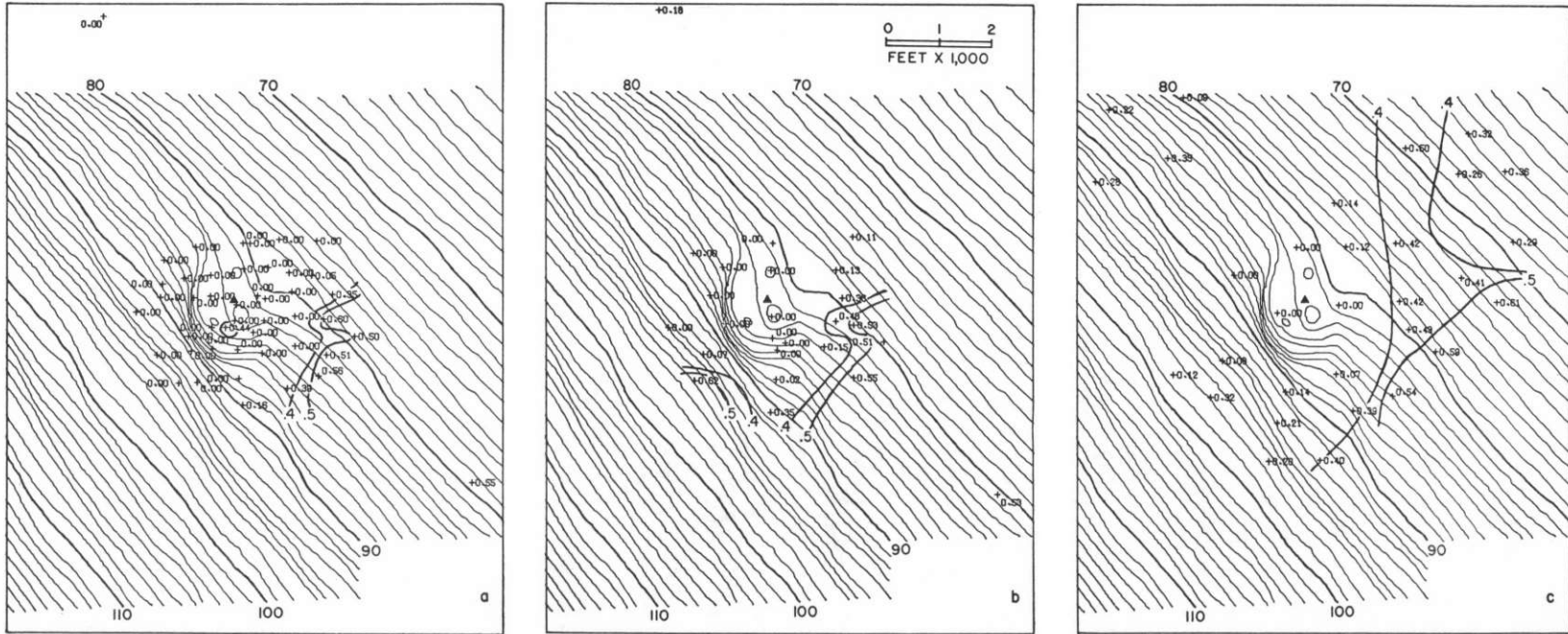
Figure A101a, b, and c. Areal distribution of Factor 4 (3.25% mode) sediment within experimental disposal Site G after the controlled disposal. Contours of loading values at 0.4, 0.5, 0.7, and 0.9. Bathymetric contours in feet. Disposal Buoy 0 is shown by ▲. Sample a - September 1975; b - October 1975; and c - December 1975.
