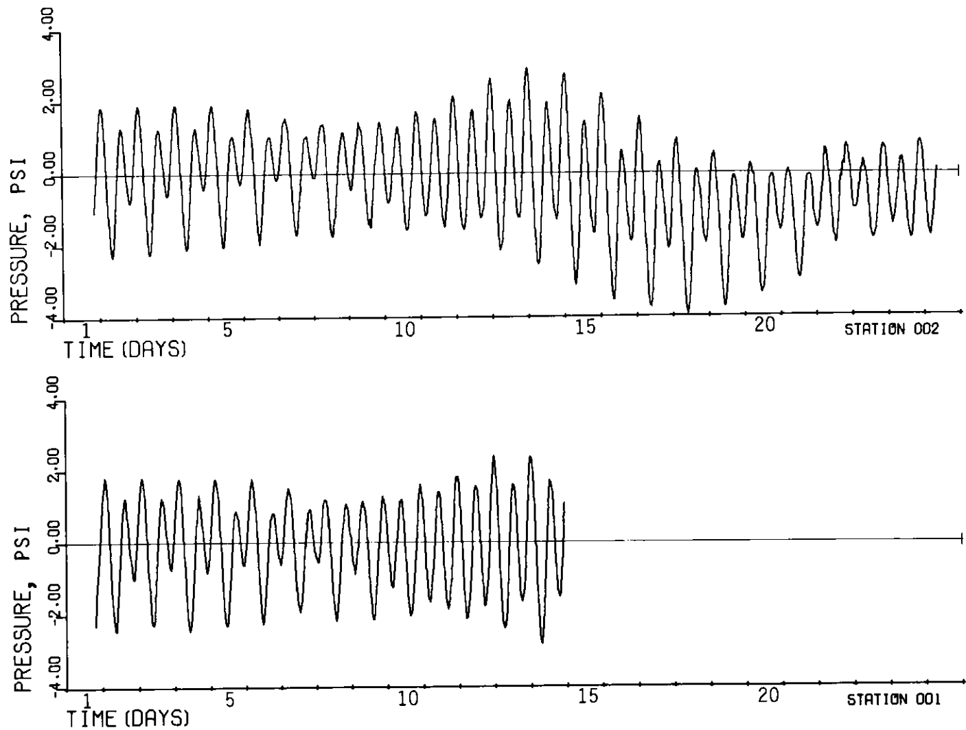
Figure A29. Tide height vs. time in days at Stations 1 and 2 during the period 1900 12 April 75 to 0800 12 May 75. The vertical scale is in psi referenced to mean sea level (1 psi ~ 2.2 ft)
