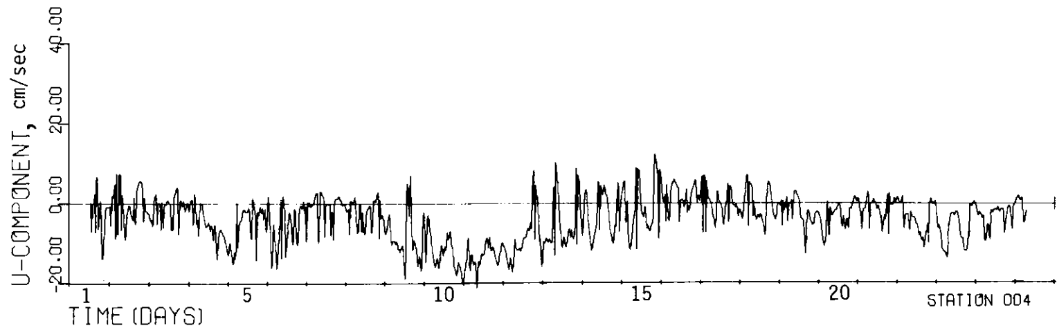
Figure A64. Northward (V) and eastward (U) components of current velocity 3.3 ft above the seabed at Station 4 during the period 1300 19 August 75 to 0800 12 September 75
