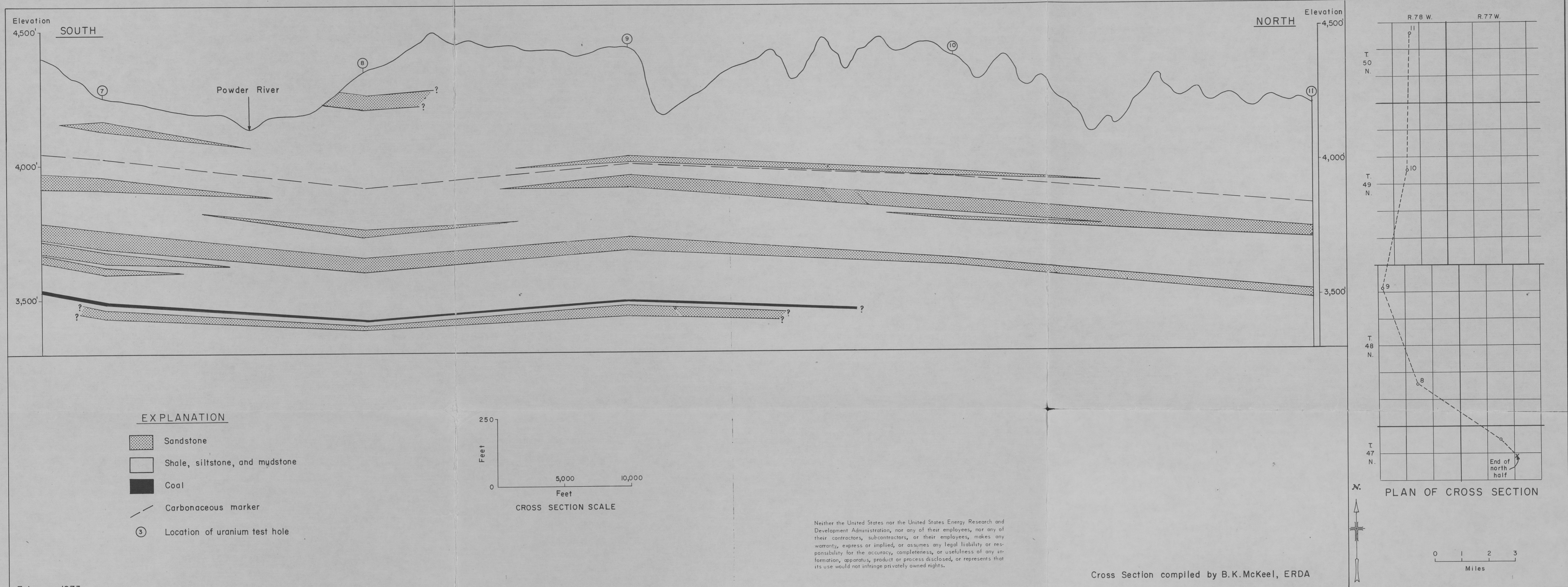
North-South Cross Section (North Half) Northern Powder River Basin, Wyoming
