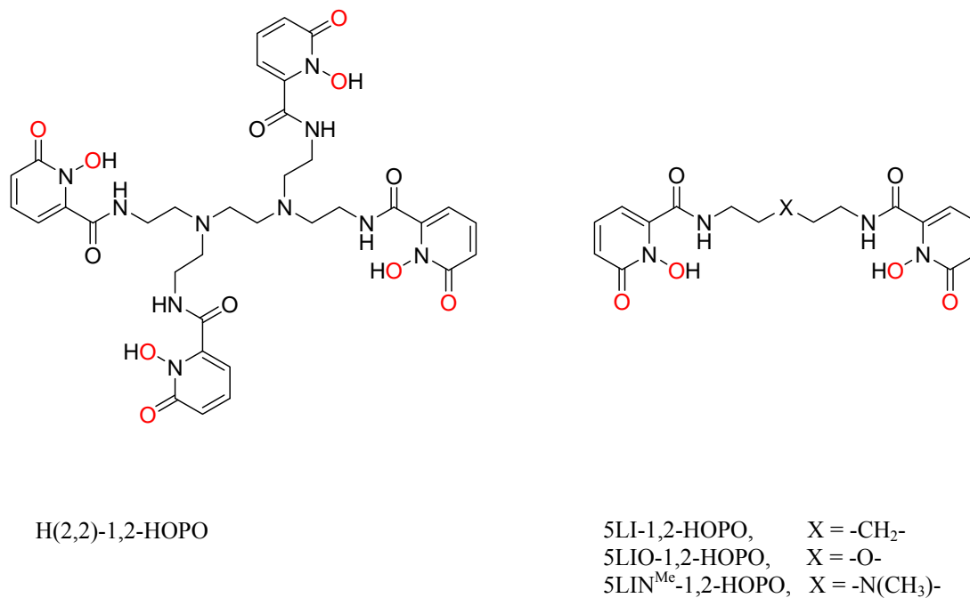
Figure 9. Chemical structures of ligands based on the 2-hydroxyisophthalamide (IAM) and 1-hydroxypyridin-2-one (1,2-HOPO) chelates.
