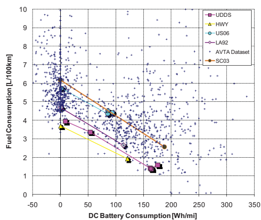
Figure 17: Electricity Consumption Space for AVTA Fleet and Dynamometer Drive Cycles
