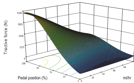
Figure 3: Response Surface Model of Tractive Force Based on Speed and Pedal Position
