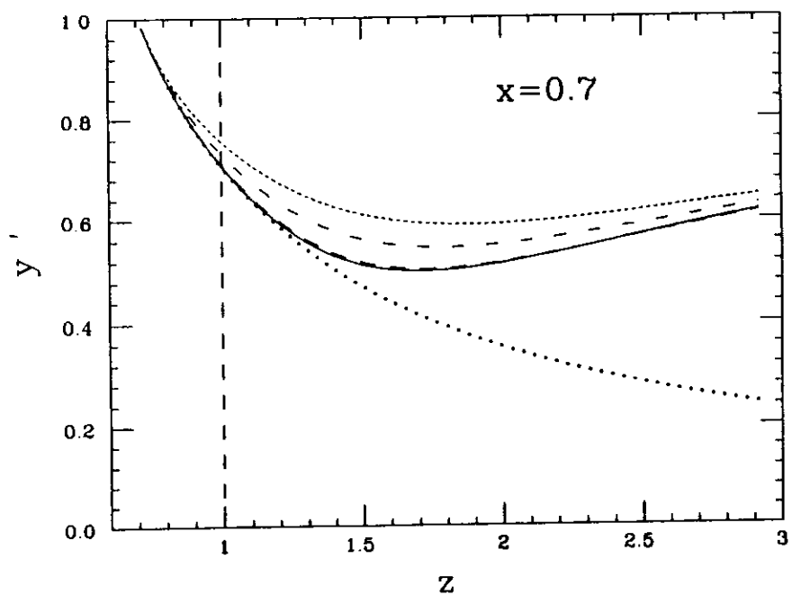
FIG. 2 The variable y' plotted as a function of the nucleon momentum fraction z for x = 0.7 , m_X = M and different values of k_1 = 0 (solid), 1 (dashed), 3 (dash-dot), and 4.5 (short dashed) \text{fm}^{-1} . The dotted line is y' = y , shown for comparison.
