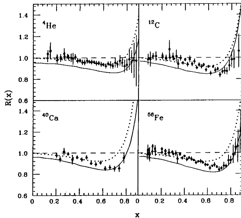
FIG. 5. The ratio R of F_2^A divided by A/2 \times F_2^D for ^4\text{He} , ^{12}\text{C} , ^{40}\text{Ca} , and ^{56}\text{Fe} . The dotted lines are the calculations of [7, 8], given for comparison, and the solid lines are the best results of this calculation (with the phase space formula for the valence quarks and no EMC effect for the sea quarks). The two curves for ^{12}\text{C} are identical to the corresponding cases shown in Fig. 4. The data are from Ref. [24] (diamonds) and Ref. [26] (boxes)
