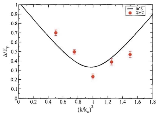
Figure 4: Neutron matter quasi-particle dispersion in BCS (line) and GFMC (points) at k_F a = -10 .
