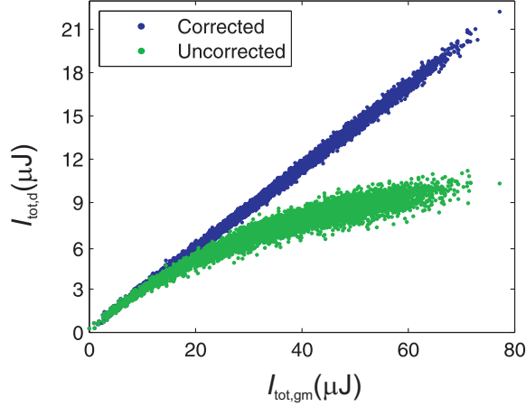
FIG. 2: Linearization of the detector: The integrated photon energy on the detector for 2000 pulses is shown as a function of the photon energy measured by the gas monitor detector of FLASH. The green dots show the raw detector data whereas the blue curve shows the data after correction for nonlinearities.
