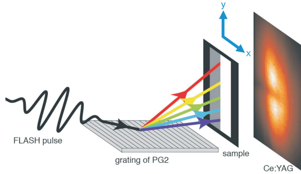
FIG. 1: Cartoon of NEXAFS in single shot spectrograph detection at FLASH. Femtosecond X-ray pulses from the SASE undulator disperse on the monochromator grating and pass through the sample. The sample is two-parted for simultaneous measurement of the absorption in the thin-film sample and the unmodified reference spectral distribution for single shot normalization. The transmitted x-rays are converted into visible light on a Ce:YAG crystal and imaged with an intensified CCD.
