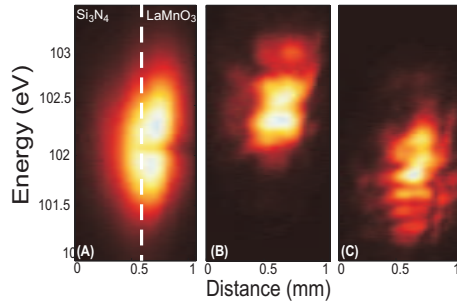
FIG. 3: (A) Sum over all the pulses of the experiment with the sample in the beam. The La absorption peak is visible at 102.17 eV. (B, C) Examples of FLASH pulses with no sample in the beamline. The energy as well as mode profile fluctuates on a pulse by pulse basis, requiring the detection of a reference spectrum for each pulse.
