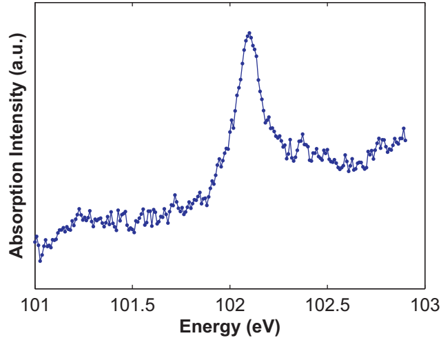
FIG. 4: The {}^3D_1 absorption resonance at the N_{4,5} -edge of the \text{La}^{3+} -ions in \text{LaMnO}_3 from all accumulated FLASH pulses.
