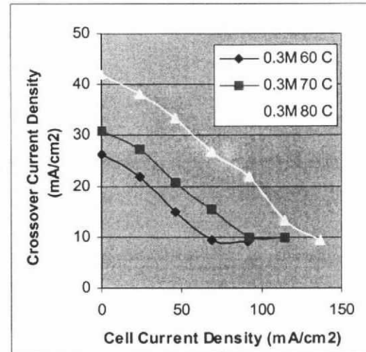
Figure 1: Crossover current density versus cell current density as a function of temperature.
