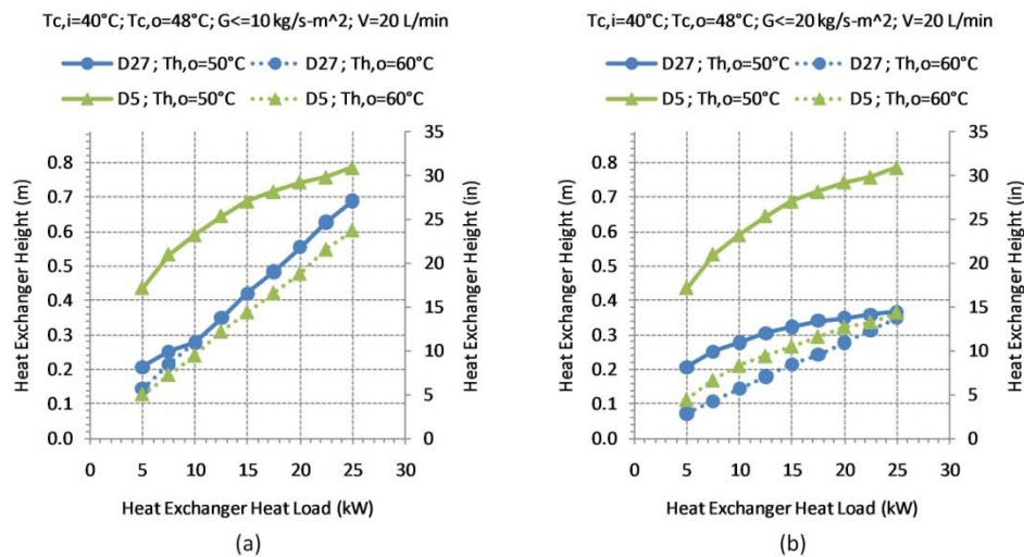
Figure 8: Louver fin heat exchanger height vs. heat load for a fixed 0.711 m (28 in.) width; (a) G_{max}=10 \text{ kg/s-m}^2 and V_h=20 \text{ L/min} ; (b) G_{max}=20 \text{ kg/s-m}^2 and V_h=20 \text{ L/min} .
