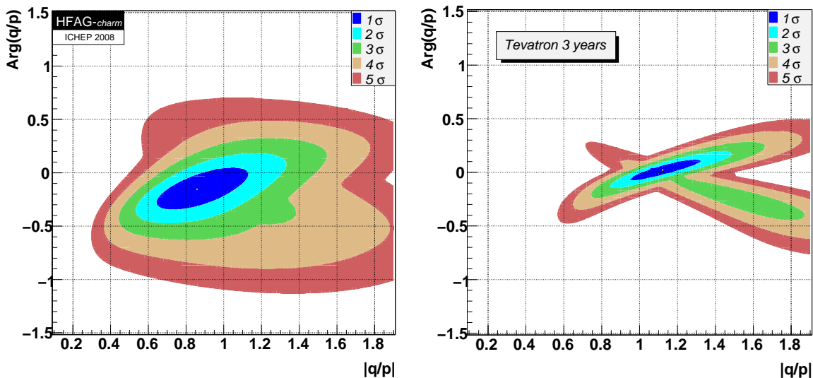
Figure 2: |q/p| versus \phi likelihood contours resulting from a global fit to measured observables (see text). Left: data after ICHEP 2008, from the HFAG [26]. Right: after three years of running of a Tevatron charm experiment.
