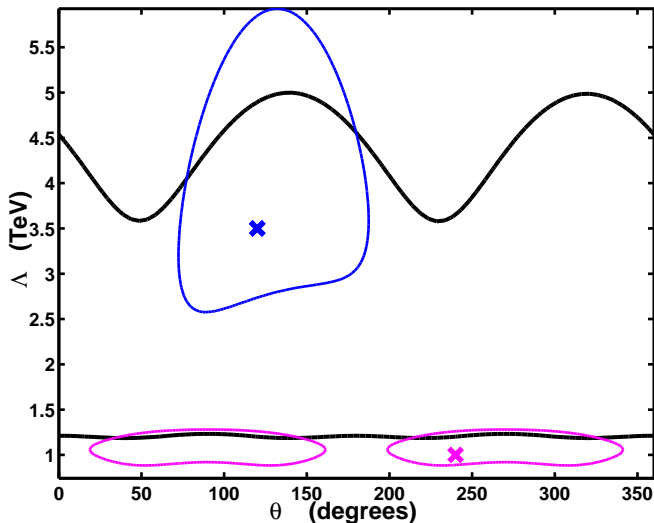
Figure 4: Dark Lines: 95% confidence level sensitivity of NuSOng to new heavy physics described by Eq. (1) when \nu_\alpha = \nu_\mu (higher curve) and \nu_\alpha \neq \nu_\mu (lower curve). Closed Contours: NuSOng measurement of \Lambda and \theta , at the 95% level, assuming \nu_\alpha = \nu_\mu , \Lambda = 3.5 TeV and \theta = 2\pi/3 (higher, solid contour) and \nu_\alpha \neq \nu_\mu , \Lambda = 1 TeV and \theta = 4\pi/3 (lower, dashed contour). Note that in the pseudoelastic scattering case ( \nu_\alpha \neq \nu_\mu ), \theta and \pi + \theta are physically indistinguishable. From [3].
