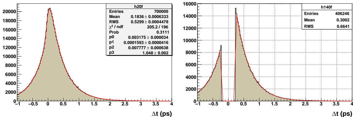
Figure 1: Monte Carlo D^0 \rightarrow K^+\pi^- decay time distributions (left) without and (right) with a minimum decay time cut. Superimposed is the result of a fit. The ratio of signal to background after the t_{\min} ( =\tau_D/2 ) cut is 0.40, and the decay time resolution \sigma_t is 75 fs.
