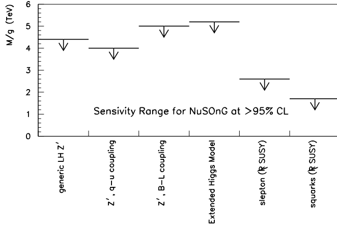
Figure 5: Some examples of NuSOng’s 2\sigma sensitivity to new high-mass particles commonly considered in the literature. For explanation of these ranges, and further examples, see [3].
