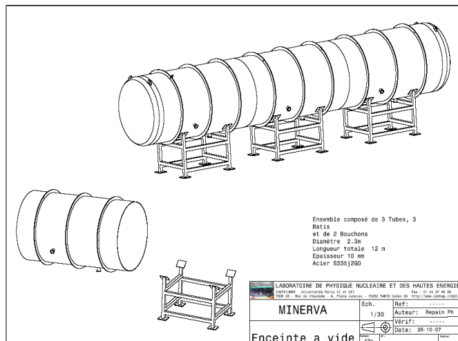
Figure 10: A 12 m long tank for the evacuated decay volume.
