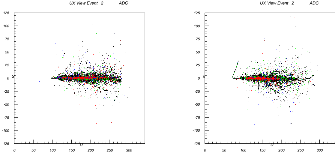
Figure 3: A 60 GeV \nu - e neutral current scatter in an LAr detector (left) and a typical 60 GeV \nu_e + n background event (right).
