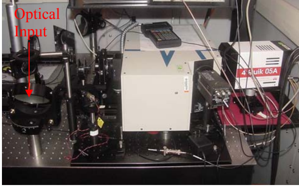
Figure 1: Photograph of the transport optics, Oriel Spectrometer, and two readout cameras for Sta-5.
