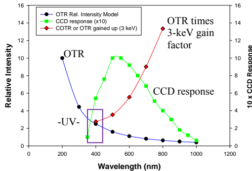
Figure 5: Analytical representations of the OTR dependence on 1/\lambda^2 and OTR times the 3-keV gain factor, or COTR. The CCD camera response is also shown.
