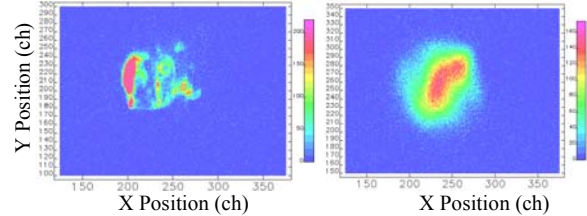
Figure 6: Beam Images via COTR from an Al mirror (left) and the 400-nm bandpass filtered LSO:Ce crystal emissions plus Al mirror COTR (right).
