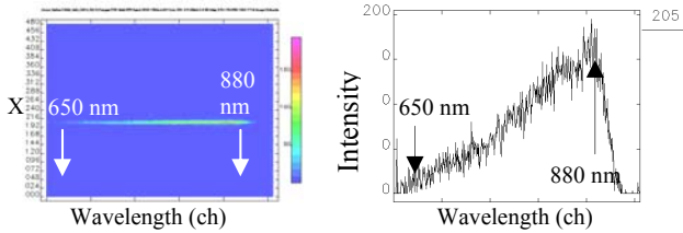
Figure 4: Imaging spectrometer results using the GaAs PC MCP-ICCD in x-\lambda space for COTR from an Al mirror (left) and the COTR spectral profile (right). The localized x extent of the COTR streak in wavelength is evident.
