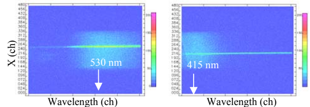
Figure 3: Imaging spectrometer results using the CCD camera readout in x-\lambda space for YAG:Ce crystal plus an
