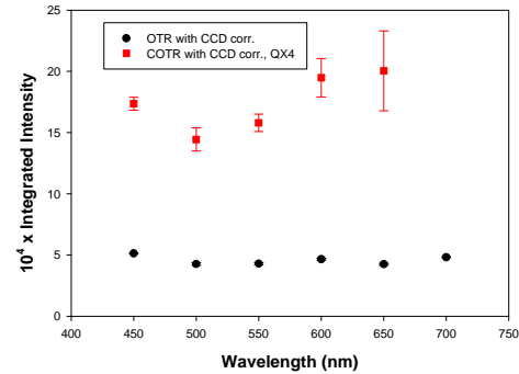
Figure 2: Evaluation of the OTR/COTR image intensities versus the bandpass filter center wavelength for the PC rf gun beam (red) and TC rf gun beam (black). The COTR has a stronger red component than the incoherent OTR.
