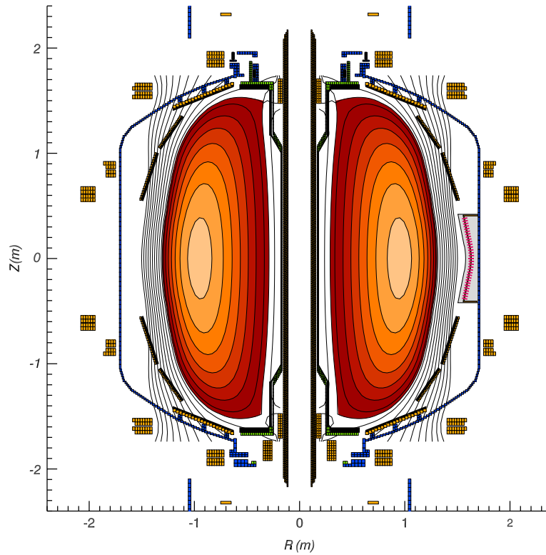
Figure 3. Flux plot of the record elongation ( \kappa = 3 ) plasma equilibrium.
