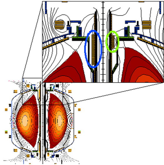
Figure 1. Detail view of the change made to the PF1A coil. The old coil is shown circled on the left, the new coil on the right.
