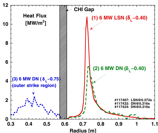
Figure 9. The peak heat flux versus major radius for three divertor configurations: (1) low \delta lower single null, (2) low \delta double null and (3) high \delta double null. All three configurations had identical heating power. The peak heat flux reduces by a factor of \sim 5 .
