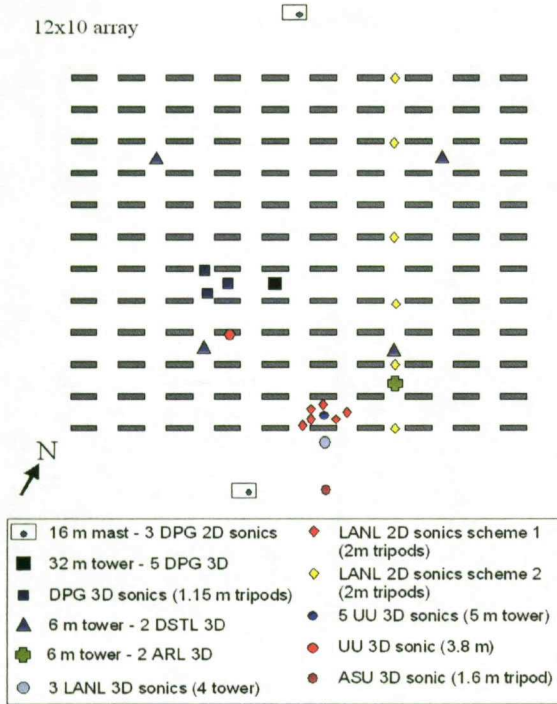
Figure 2. Schematic showing the relative locations of the sonic anemometers employed in MUST. Not to scale. Organizations: ARL (Army Research Laboratory); ASU (Arizona State University); DPG (Dugway Proving Grounds); DSTL (Defense Science Technology Laboratory); UU (University of Utah).
