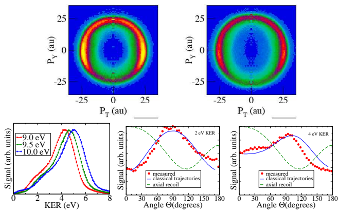
FIG. 2: (Color online) Top: Scatter plots for \text{H}^- production from {}^2\text{A}_1 resonance at 9.0 and 10 eV. Bottom: angular integrated experimental KER distributions (left); comparison of measured and calculated angular distributions at 2 eV (middle) and 4 eV (right) at 9.5 eV.
