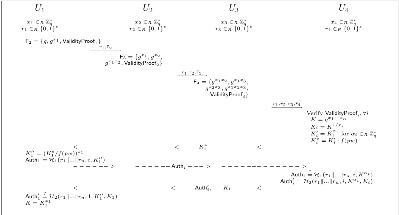
Figure 2: An honest execution of the password-authenticated Diffie-Hellman Group Open Key Exchange (GOKE) protocol with four players \mathcal{U} = \{U_1, U_2, U_3, U_4\} . The session key is sk_i = \mathcal{H}_0(r_1 \| \dots \| r_n, K) .
