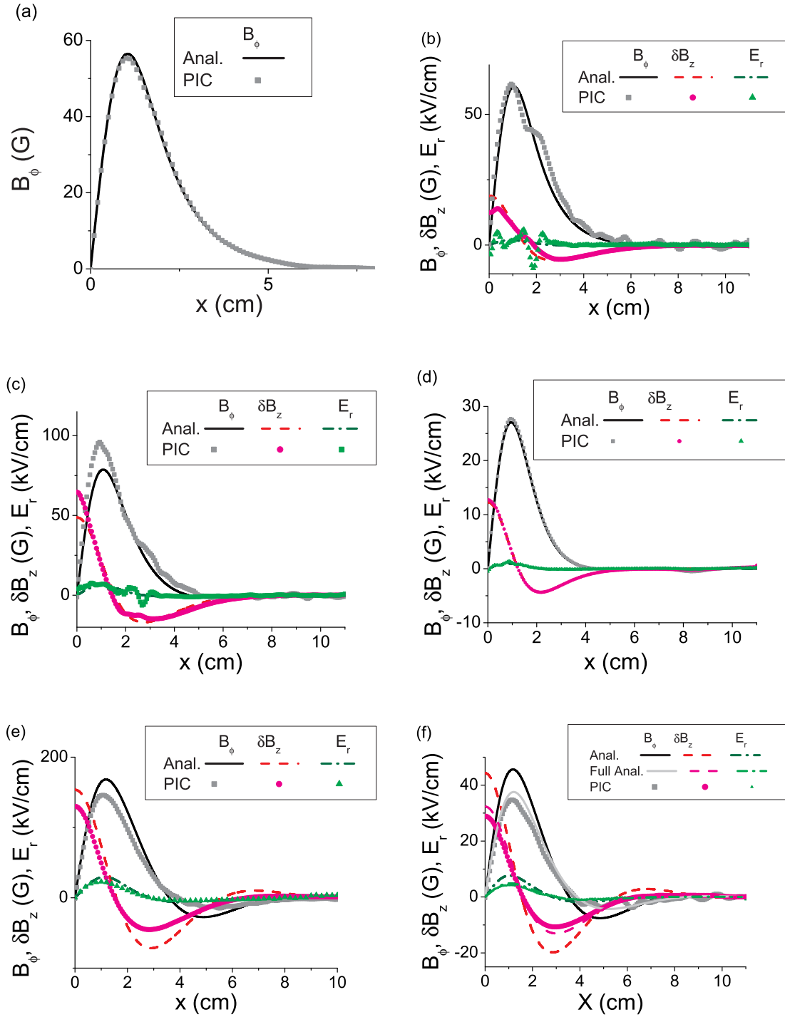
FIG. 6: (Color online) Comparison of analytic theory and LSP particle-in-cell simulation results for the self-magnetic field, perturbation in the solenoidal magnetic field, and the radial electric field in a perpendicular slice of the beam pulse. The beam parameters are the same as in Fig.5 with n_{b0} = n_p/2 = 1.2 \times 10^{11} \text{cm}^{-3} , except for (d), where n_{b0} = n_p/8 = 0.6 \times 10^{11} \text{cm}^{-3} , and (f), where n_{b0} = n_p/8 = 0.3 \times 10^{11} \text{cm}^{-3} . The values of the applied solenoidal magnetic field, B_{z0} are: (a) B_{z0} = 0\text{G} ; (b) B_{z0} = 300\text{G} ; (c) and (d) B_{z0} = 600\text{G} ; (e) and (f) B_{z0} = 900\text{G} .
