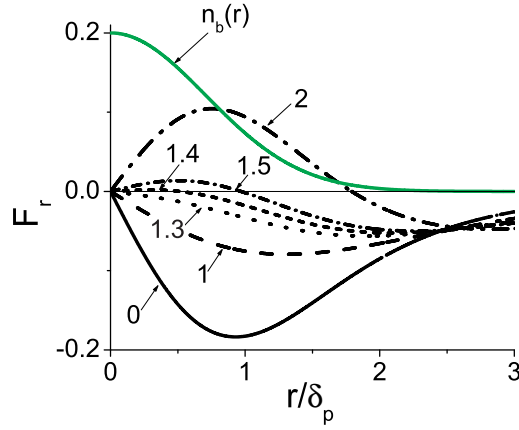
FIG. 9: (Color online) The normalized radial force F_r/(Z_b^2 n_{b0} m V_{bz}^2/n_p \delta_p) acting on the beam particles for different values of the parameter \omega_{ce}^2/\omega_{pe}^2 \beta_b^2 . The green line shows the gaussian density profile multiplied by 0.2 in order to fit the profile into the plot. The beam radius is equal to the skin depth, r_b = \delta_p .
