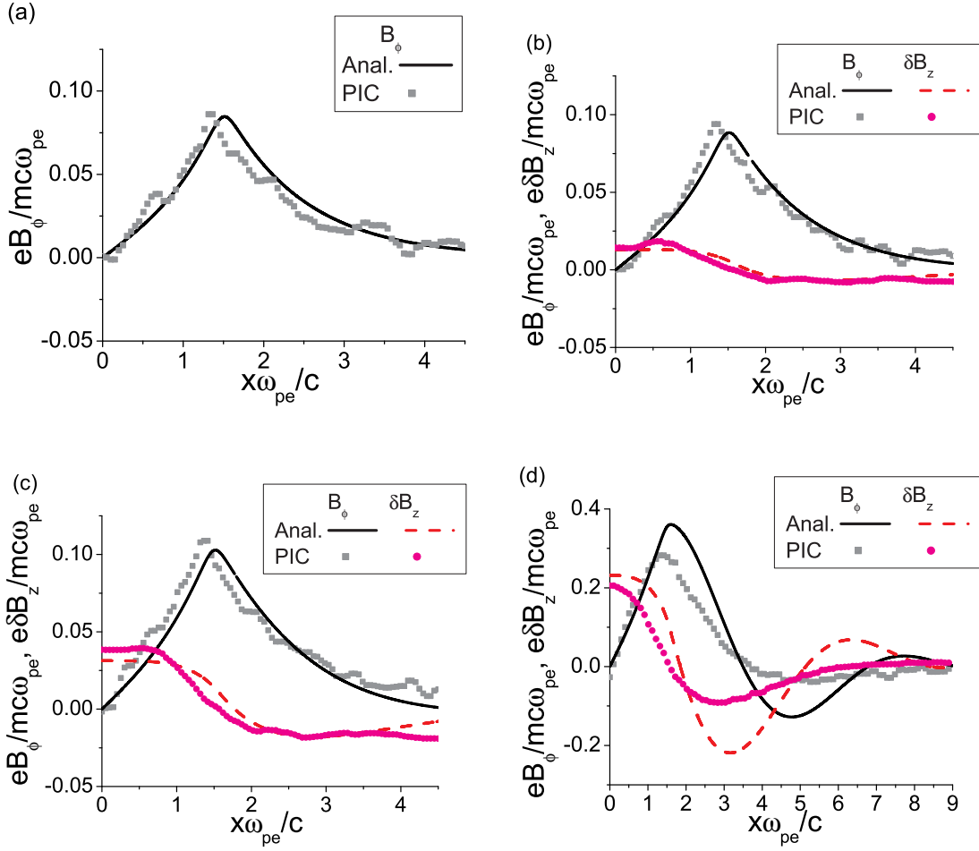
FIG. 4: (Color online) Comparison of analytic theory and EdPIC particle-in-cell simulation results for the self-magnetic field and the perturbations in the solenoidal magnetic field in the center slice of the beam pulse. The beam parameters are the same as in Fig.3. The beam velocity V_b = 0.5c . The values of applied solenoidal magnetic field correspond to the ratio of cyclotron to plasma frequency \omega_{ce}/\omega_{pe} : (a) 0; (b) 0.25; (c) 0.5; and (d) 1.
