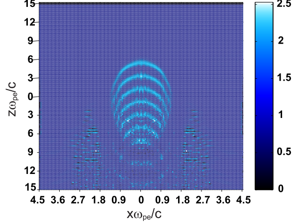
FIG. 3: (Color online) The electron density perturbation caused by an ion beam pulse moving with velocity V_b = 0.5c along the z -axis. The beam density is one-half of the background plasma density; the beam profile is flat-top with smooth edges; the beam radius is r_b = 1.5c/\omega_{pe} ; and the beam half length is l_b = 7.5c/\omega_{pe} .
