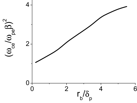
FIG. 10: (Color online) The parameter \omega_{ce}^2/\omega_{pe}^2\beta_b^2|_{op} plotted as a function of r_b/\delta_p corresponding to the minimum radial force for effective beam transport over long distances. The beams have gaussian density profiles with different values of r_b/\delta_p .
