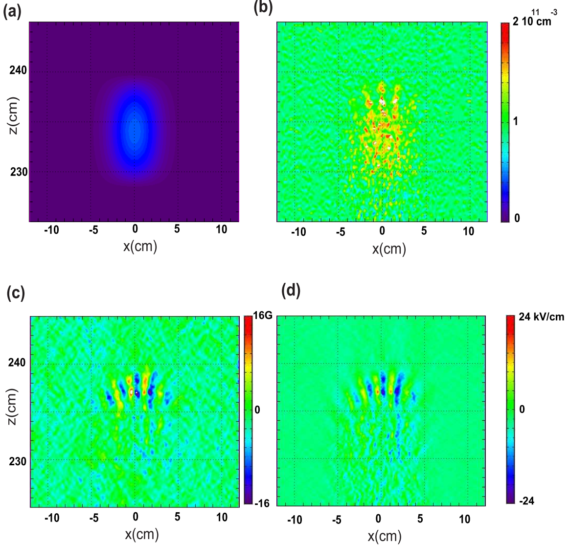
FIG. 11: (Color online) LSP particle-in-cell simulation results for the perturbations in electron density, self-magnetic field and self-electric radial field. The beam velocity is V_b = 0.2c . The plasma and beam parameters are n_p = 10^{11} \text{cm}^{-3} , and n_{b0} = 0.5 \times 10^{11} \text{cm}^{-3} . The beam density profile is gaussian, n_{b0} \exp(-z^2/l_b^2 - r^2/r_b^2) , where r_b = 2.8 \text{cm} , and l_b = 5.7 \text{cm} . The value of the applied solenoidal magnetic field is, B_{z0} = 2839 \text{G} . Figure 11 (a) shows the beam density; (b) the electron density; (c) the self-magnetic field B_y ; and (d) the self-electric field E_x .
