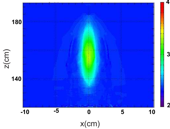
FIG. 5: (Color online) The electron density perturbation caused by an ion beam pulse moving with velocity V_b = 0.33c along the z -axis. The beam density profile is gaussian with r_b = 1cm , l_b = 17cm , and n_{b0} = n_p/2 = 1.2 \times 10^{11}cm^{-3} .
