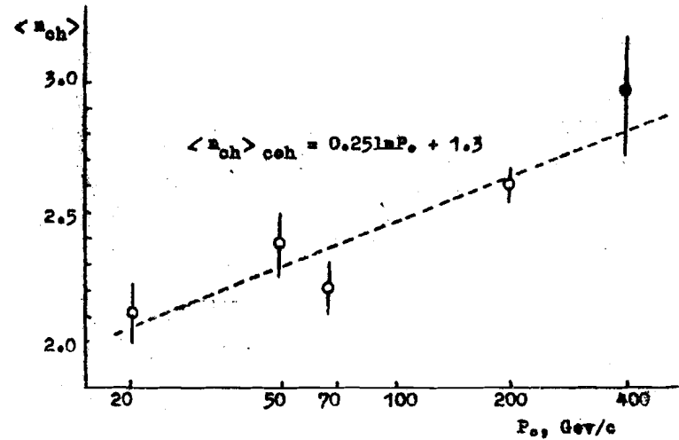
Fig.4. The energy dependence of the mean multiplicity of charged particles in reactions ( 1 ). The data at P_0 = 20 - 200 Gev/c from the review 4/
