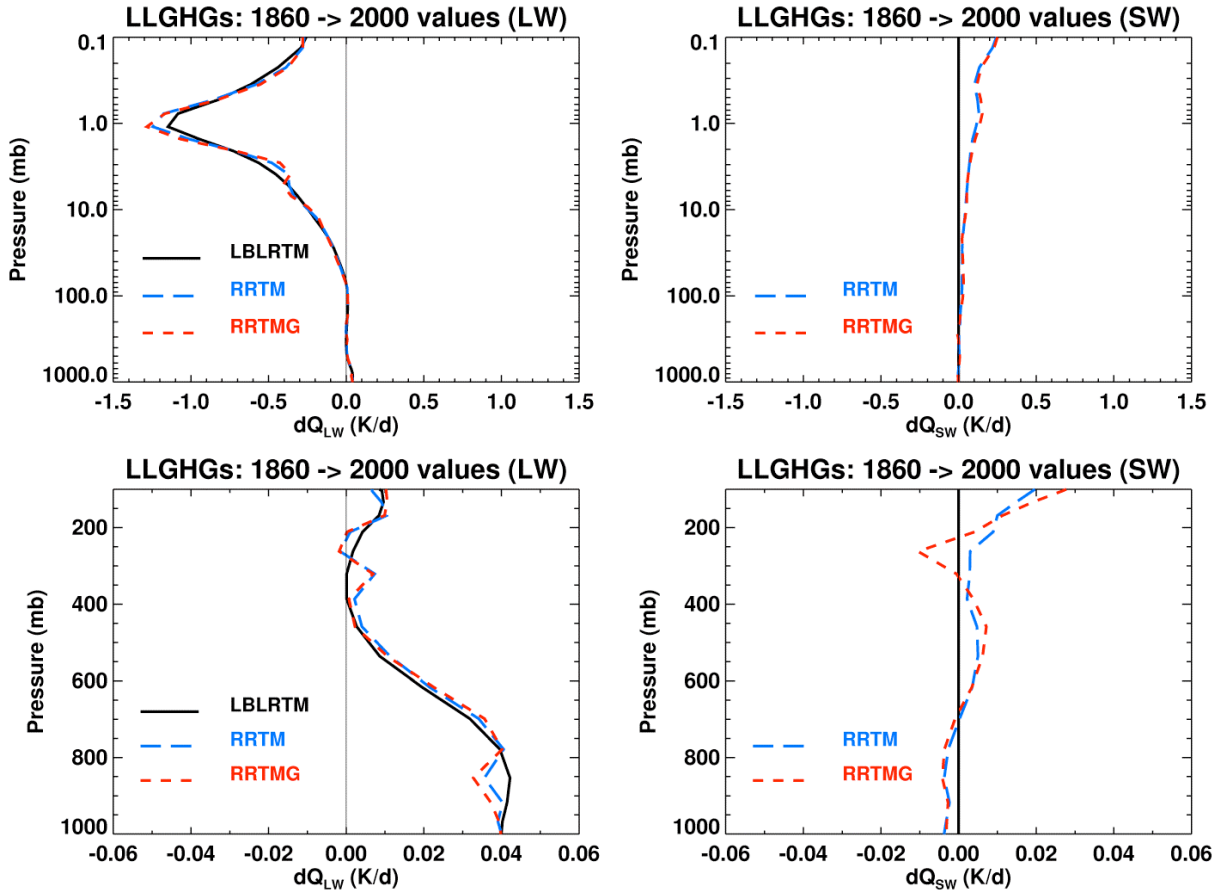
Figure 2. Heating rate profile differences from increasing the concentrations of \text{CO}_2 , \text{CH}_4 , \text{N}_2\text{O} , CFC-11 and CFC-12 from 1860 to 2000 values using the standard mid-latitude summer profile for the longwave (left) and shortwave (right) as calculated by the AER radiation models.
