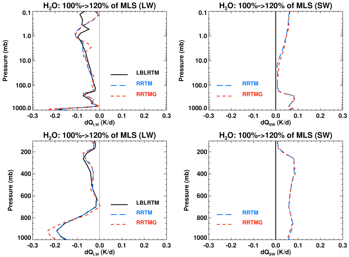
Figure 3. Heating rate profile differences from increasing the water vapor concentration in the standard mid-latitude summer profile in all layers by 20 percent with doubled \text{CO}_2 (574 ppmv) in all calculations for the longwave (left) and shortwave (right) as calculated by the AER radiation models.
