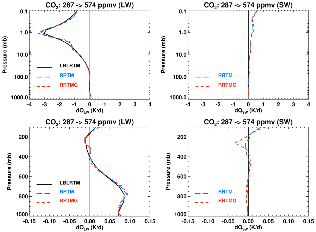
Figure 1. Heating rate profile differences from doubling the CO 2 concentration from 287 to 574 ppmv using the standard mid-latitude summer profile for the longwave (left) and shortwave (right) as calculated by the AER radiation models.
