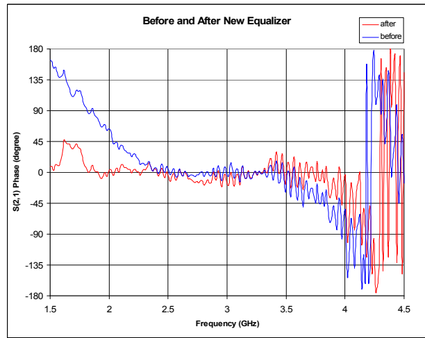
Figure 8: Phase of transfer function before and after installation of an equalizer.
