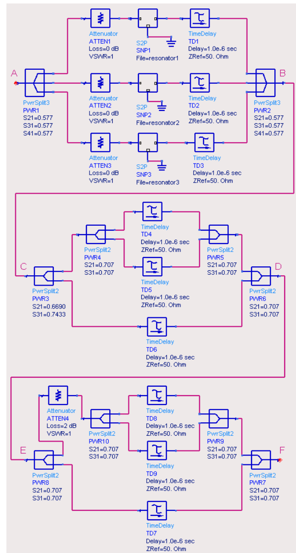
Figure 1: Schematic of a new equalizer.
