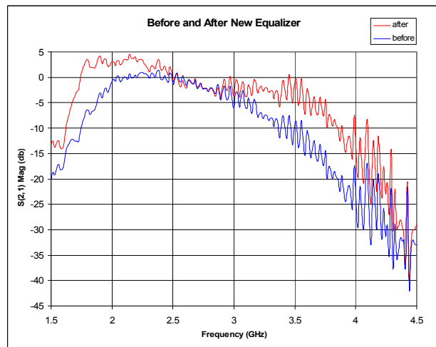
Figure 9: Amplitude of transfer function before and after installation of an equalizer.
