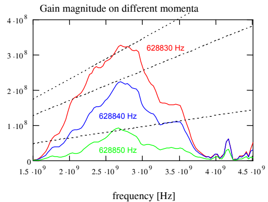
Figure 10: Stacktail gain before installation of an equalizer.
