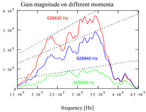
Figure 11: Stacktail gain after installation of an equalizer.
