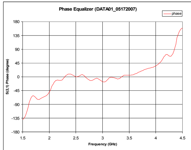
Figure 3: Phase of a phase equalizer part.
