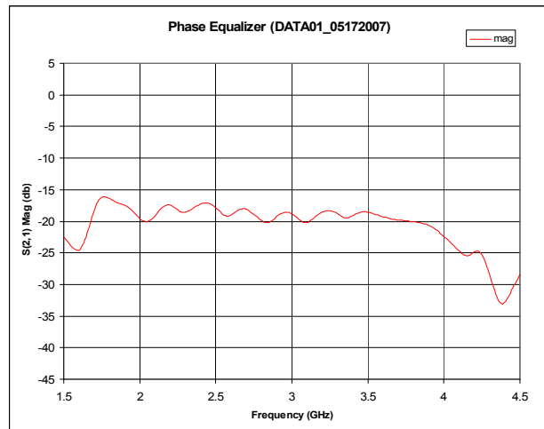
Figure 4: Amplitude of a phase equalizer part.
