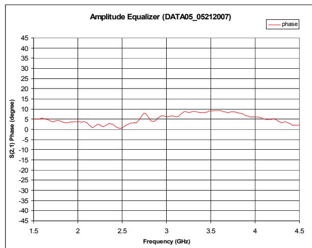
Figure 5: Phase of an amplitude equalizer part.
