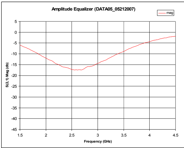
Figure 6: Amplitude of an amplitude equalizer part.
