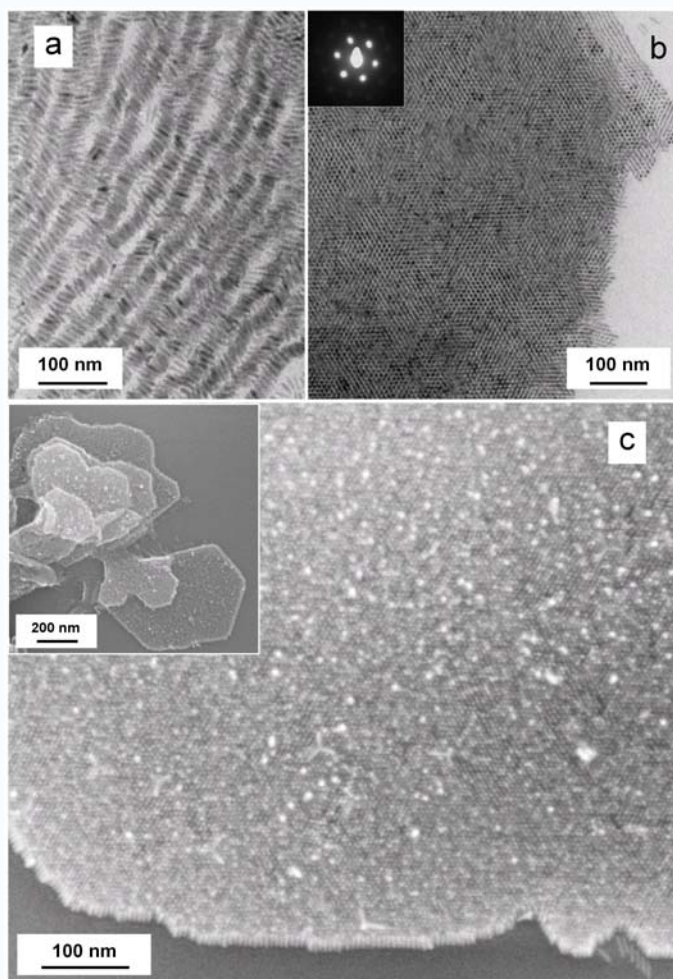
Figure 4. Self-assembly of CdSe/CdS nanorods with length 24 nm and diameter 5.2 nm. (a) TEM image of a superstructure with smectic-A ordering. (b) TEM image of a nanorod superlattice with simple hexagonal packing of nanorods assembled perpendicular to the substrate. Inset shows electron diffraction from a superlattice domain. (c) HRSEM image of CdSe/CdS nanorods assembled perpendicular to the substrate (silicon wafer). Inset shows layer-by-layer growth of a nanorod superlattice.
