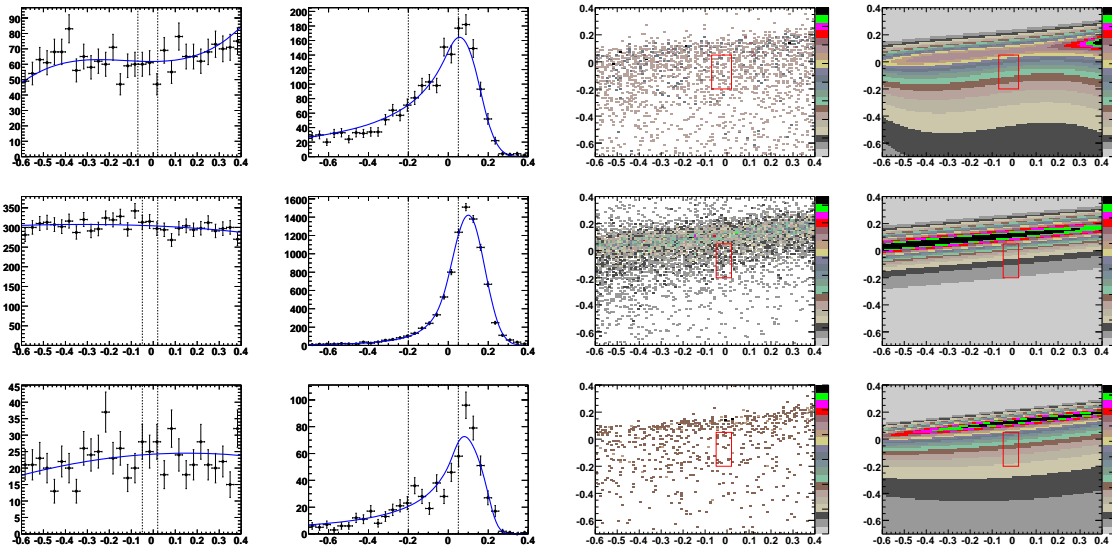
Figure C.15: Bhabha and di-muon backgrounds: Fit of the Bhabha and di-muon ( \Delta M, \Delta E ) MC distributions with PDF described in the text. column 1) \Delta M projection of the control sample distribution (points) and the PDF (curve); column 2) \Delta E projection of the control sample distribution (points) and the PDF (curve); column 3) control sample ( \Delta M, \Delta E ) distribution; column 4) PDF ( \Delta M, \Delta E ) distribution; row 1) e^-e^+e^- ; row 2) \mu^-e^+e^- ; row 3) e^-\mu^+\mu^- . \Delta M is plotted in ( \text{GeV}/c^2 ) and \Delta E is plotted in ( \text{GeV} ). Only channels with significant QED contributions in the LB are shown.
