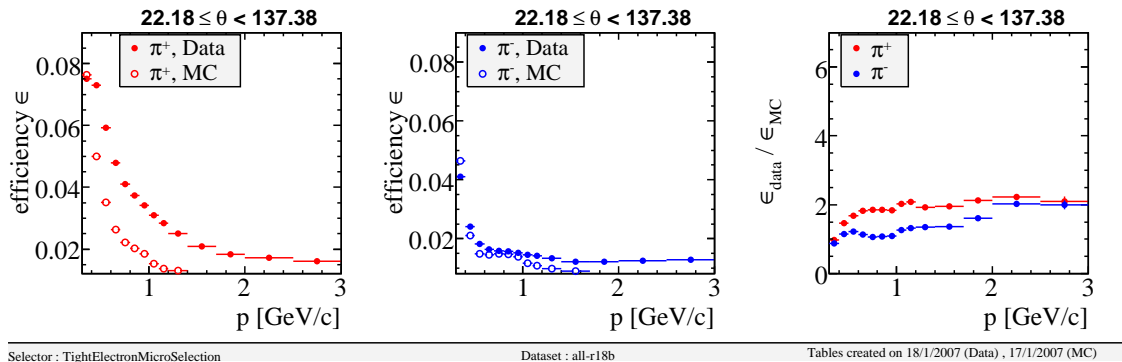
Figure III.3: The mis-ID rate for pions in data and MC by the eMicroTight selector, as a function of particle momentum for (a) positively charged pions, and (b) negatively charged pions. Plot (c) shows the ratio of the data mis-ID rate to the MC mis-ID rate.
