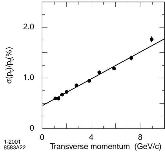
Figure II.15: Transverse momentum resolution, as determined from cosmic ray muons traversing the DCH and SVT.
