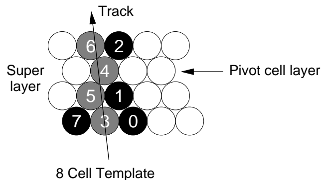
Figure II.24: Track Segment Finder pivot group.
