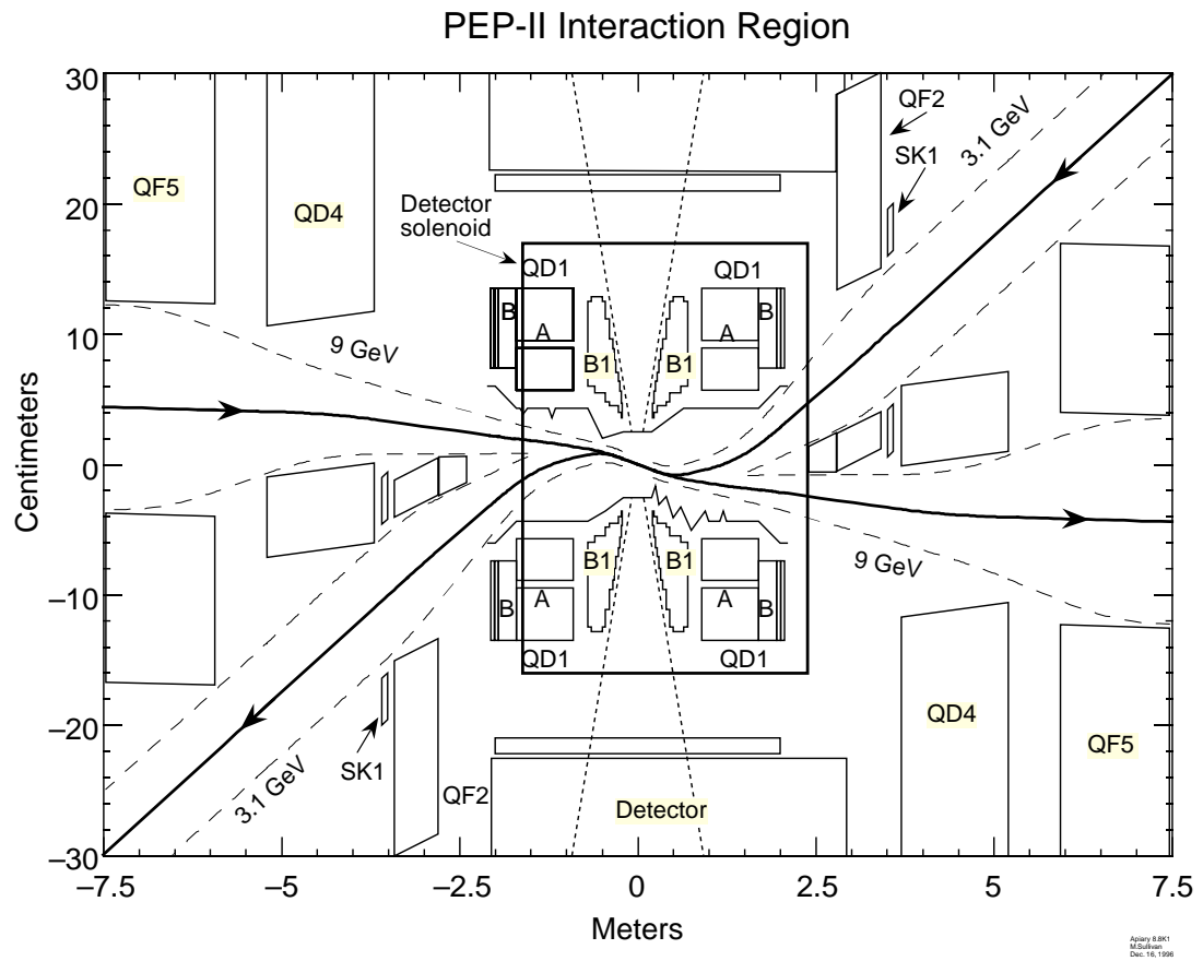
Figure II.1: The PEP-II interaction region around the BABAR detector.
