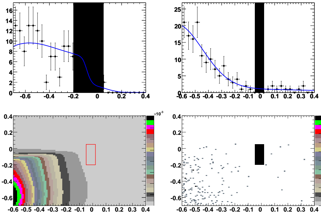
Figure III.12: \tau^- \rightarrow e^+ \mu^- \mu^- channel: PDFs with MC-fitted shapes are scaled to data; a) \Delta E projection of the data (points) and the sum of the background PDFs (curve); b) \Delta M projection of the data (points) and the sum of the background PDFs (curve); c) PDF ( \Delta M, \Delta E ) distribution; d) data ( \Delta M, \Delta E ) distribution. The filled black boxes and open red box show the signal region (blinded for data).
