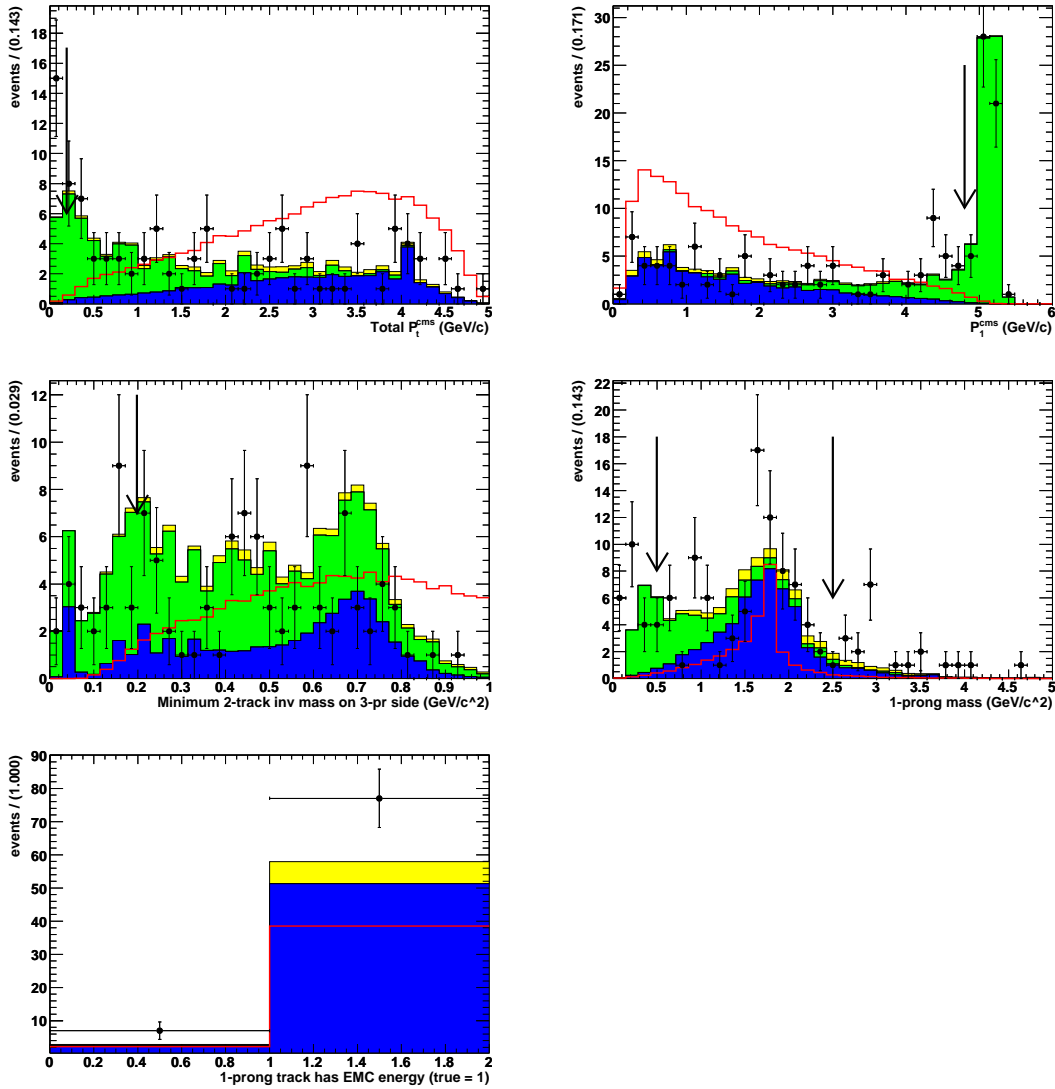
Figure C.8: \tau^- \rightarrow \mu^- e^+ e^- channel a) total transverse momentum; b) 1-prong momentum; c) min 2-track mass; d) 1-prong mass; e) (bool) one-prong track has EMC energy. The points show the data distributions for events in the grand sideband region with all other cuts applied. The blue histogram shows the expected \tau^+ \tau^- background level, the green histogram shows the expected dimuon background level, and the yellow histogram shows the expected uds background level, all normalized by the background fits with all selection cuts applied. Arrow(s) indicate the chosen cut value(s). For comparison, the red curve shows the MC signal distribution for the large box with arbitrary normalization.
