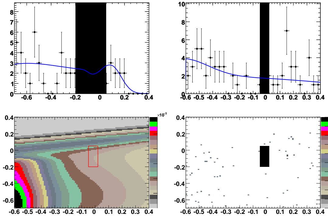
Figure III.10: \tau^- \rightarrow \mu^- e^+ e^- channel: PDFs with MC-fitted shapes are scaled to data; a) \Delta E projection of the data (points) and the sum of the background PDFs (curve); b) \Delta M projection of the data (points) and the sum of the background PDFs (curve); c) PDF (\Delta M, \Delta E) distribution; d) data (\Delta M, \Delta E) distribution. The filled black boxes and open red box show the signal region (blinded for data).
