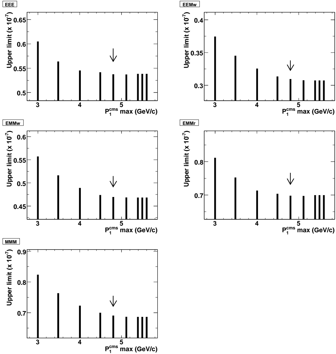
Figure C.1: Expected upper limit on branching fraction as a function of p_1^{cms} . \mu^- e^+ e^- channel is excluded because the dimuon control sample does not have a requirement on the maximum value of p_1^{cms} (see section 7). Arrows indicate optimized value for the selection cut.
