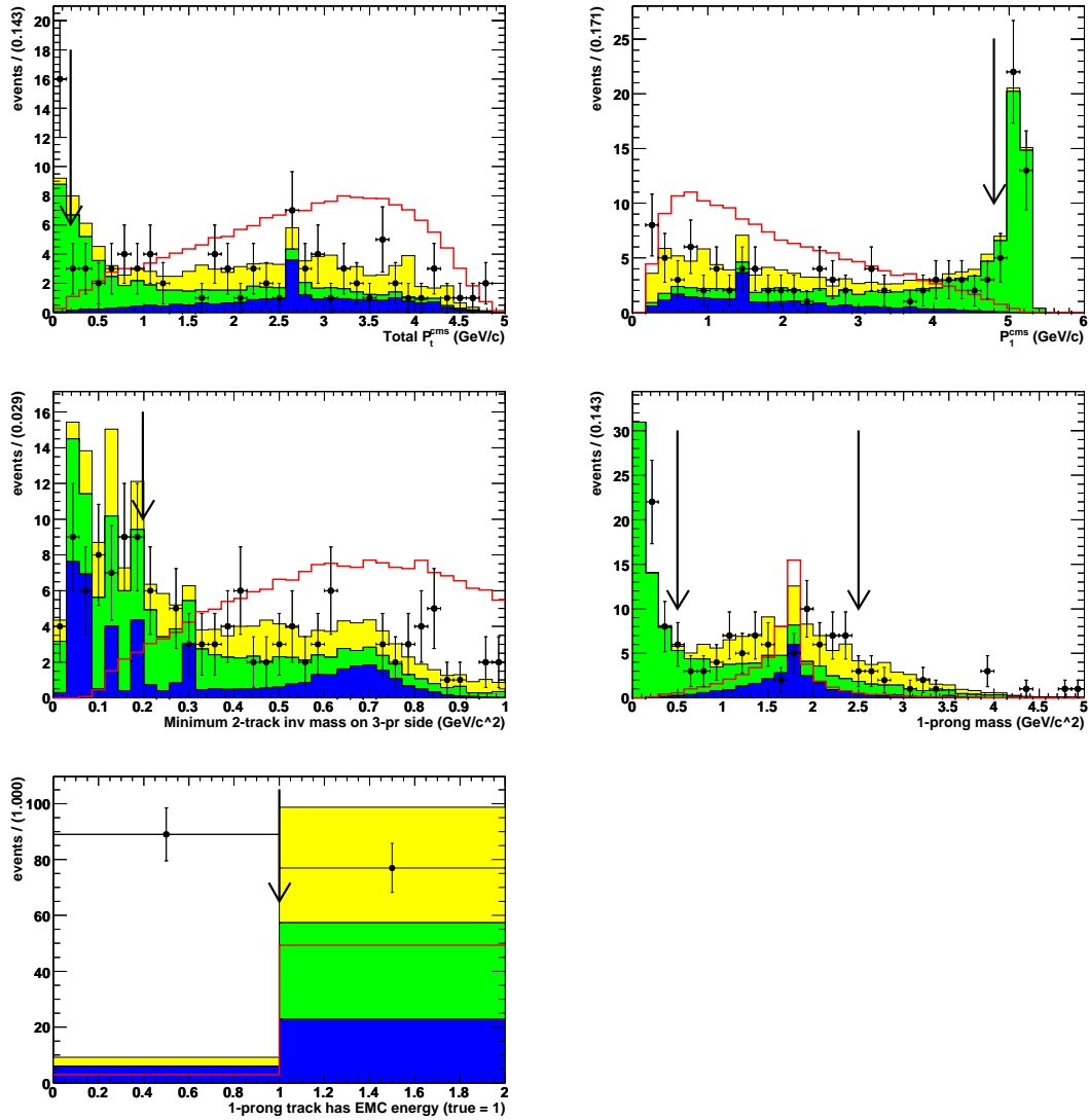
Figure C.7: \tau^- \rightarrow e^-e^+e^- channel a) total transverse momentum; b) 1-prong momentum; c) min 2-track mass; d) 1-prong mass; e) (bool) one-prong track has EMC energy. The points show the data distributions for events in the grand sideband region with all other cuts applied. The blue histogram shows the expected \tau^+\tau^- background level, the green histogram shows the expected Bhabha background level, and the yellow histogram shows the expected uds background level, all normalized by the background fits with all selection cuts applied. Arrow(s) indicate the chosen cut value(s). For comparison, the red curve shows the MC signal distribution for the large box with arbitrary normalization.
