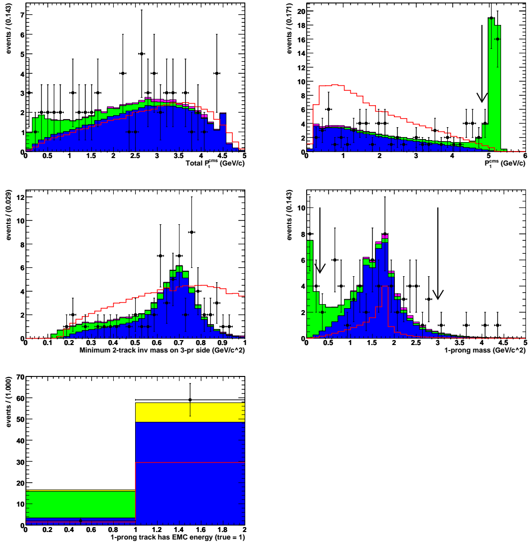
Figure C.9: \tau^- \rightarrow \mu^+ e^- e^- channel a) total transverse momentum; b) 1-prong momentum; c) min2-track mass; d) 1-prong mass; e) (bool) one-prong track has EMC energy. The points show the data distributions for events in the grand sideband region with all other cuts applied. The blue histogram shows the expected \tau^+ \tau^- background level, the green histogram shows the expected Bhabha background level, and the yellow histogram shows the expected uds background level, all normalized by the background fits with all selection cuts applied. Arrow(s) indicate the chosen cut value(s). For comparison, the red curve shows the MC signal distribution for the large box with arbitrary normalization.
