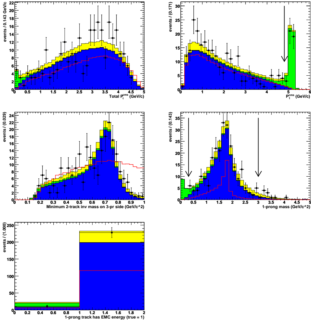
Figure C.10: \tau^- \rightarrow e^+\mu^-\mu^- channel a) total transverse momentum; b) 1-prong momentum; c) min 2-track mass; d) 1-prong mass; e) (bool) one-prong track has EMC energy. The points show the data distributions for events in the grand sideband region with all other cuts applied. The blue histogram shows the expected \tau^+\tau^- background level, the green histogram shows the expected Bhabha background level, and the yellow histogram shows the expected uds background level, all normalized by the background fits with all selection cuts applied. Arrow(s) indicate the chosen cut value(s). For comparison, the red curve shows the MC signal distribution for the large box with arbitrary normalization.
