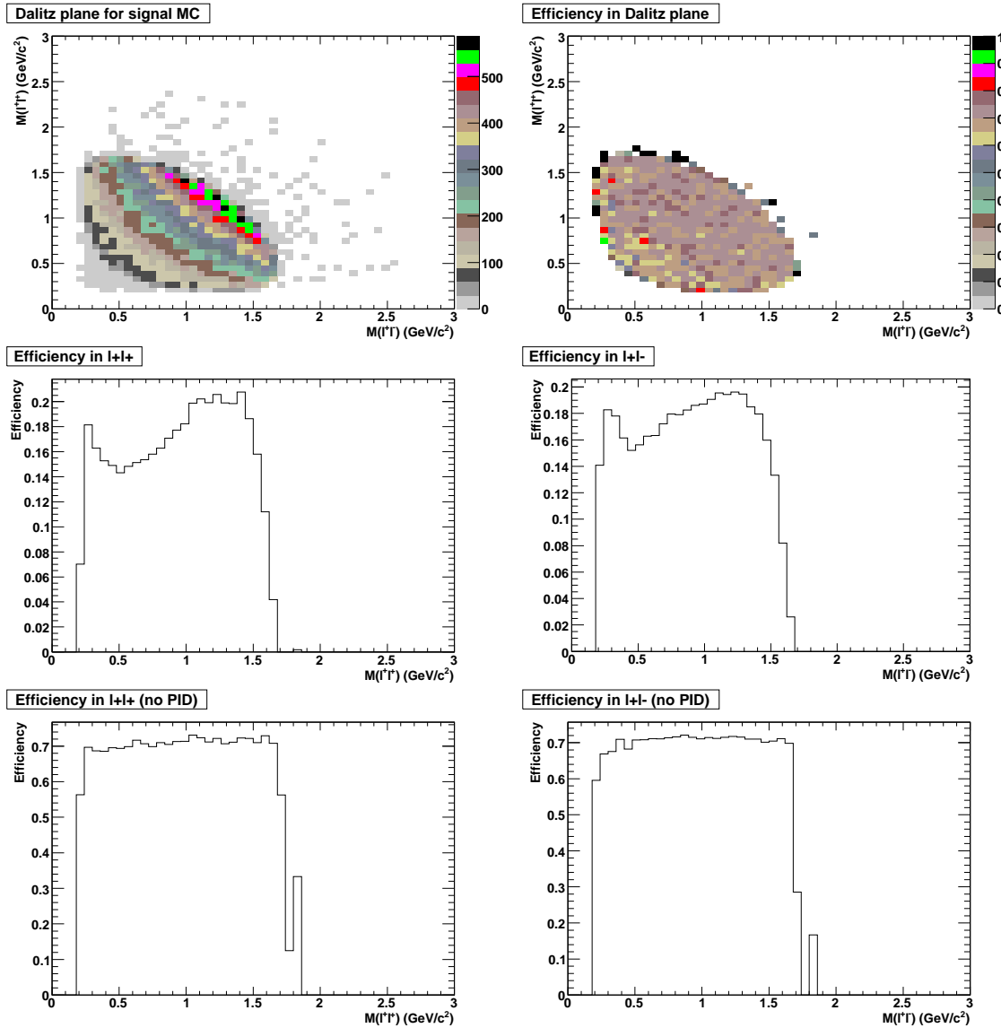
Figure III.15: \tau^- \rightarrow \mu^- \mu^+ \mu^- a) generated MC Dalitz distribution after preselection; b) efficiency to pass all selection except SB as function of Dalitz distribution; c) selection efficiency as a function of invariant mass squared of the pair of same-sign leptons; d) selection efficiency as a function of invariant mass squared of the pair of opposite-sign leptons; e) efficiency for all selection cuts except PID as a function of invariant mass squared of the pair of same-sign leptons; e) efficiency for all selection cuts except PID as a function of invariant mass squared of the pair of opposite-sign leptons;
