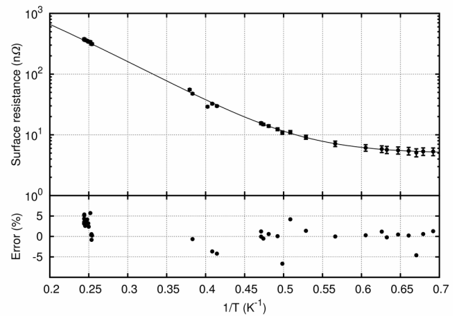
Fig. 3. The measurement of the residual resistance of the Accel-6 cavity. Only the data below T_\lambda ( 1/T=0.46 \text{ K}^{-1} ) were used in the fit.
