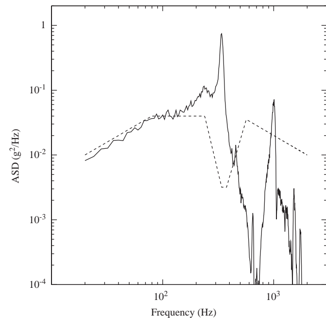
Fig. 10. Z-axis random vibration test on the TKR ID 6. Dashed line: notched input ASD spectrum. Solid line: response of the accelerometer #3.
