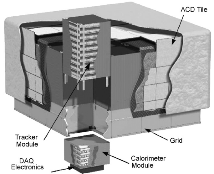
Fig. 1. Cutaway view of the LAT detector. Each tower in the 4 \times 4 array includes a TKR and a CAL.
