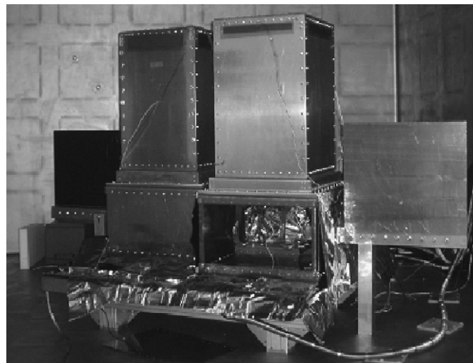
Fig. 12. Thermal-vacuum test set-up.
