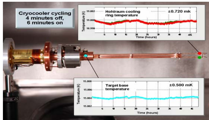
Figure 6. The required \pm 1\text{mK} temperature stability has been demonstrated in the lab. The surrogate target is shown with its thermal shroud removed.
