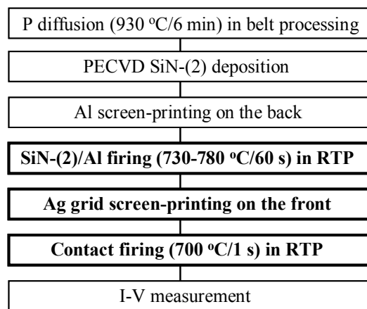
Figure 1-13. A process sequence for record high efficiency screen-printed EFG Si cells, involving two-step RTP for defect passivation and good contacts.
