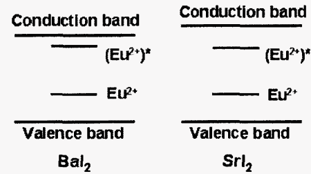
FIG. 3. (Color online) Postulated energy level diagram for the \text{BaI}_2(\text{Eu}) and \text{SrI}_2(\text{Eu}) systems.
