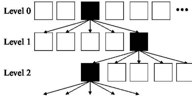
Fig. 1. Hierarchical partitioning of the Biot-Savart matrix. The highest level of partitioning is based on the number of processors. Some of the the interactions at any Level l will be full rank (black boxes), and these interactions are sub-partitioned by decomposing the corresponding sub-volume and sub-surface to create Level l+1 .
