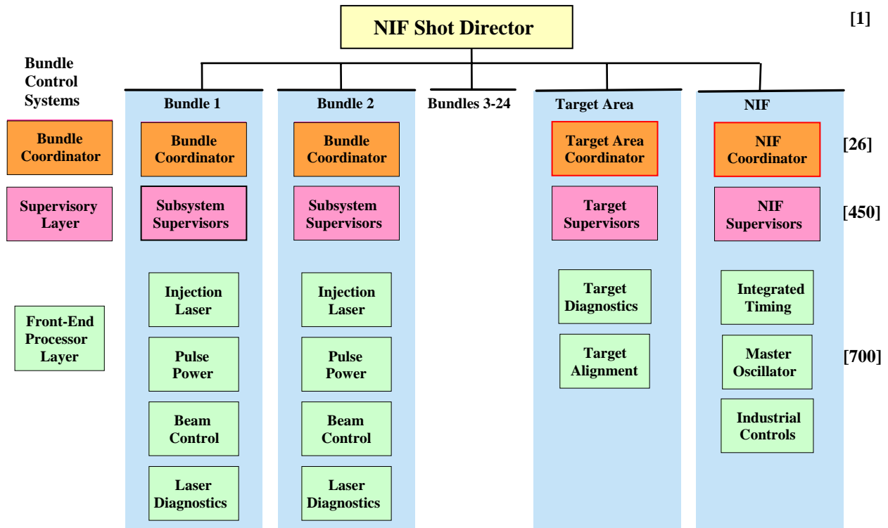
Figure 2: Shot Management Layers
