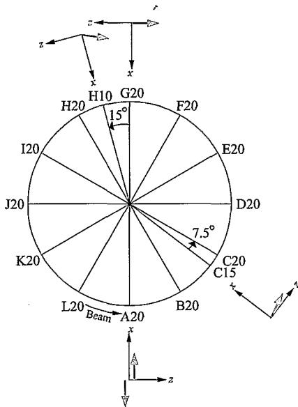
Figure 2: Basic geometry of the AGS spin precession with a 15% partial snake in the A20 straight section at extraction energy ( G\gamma = 46.5 ). For the superconducting helical snake, the snake's rotation axis is longitudinal as in a solenoid. is a left-handed rotation of 27^\circ about the longitudinal axis from a tilt of 13.5^\circ radially outward to 13.5^\circ radially inward if the spin is predominantly vertical. Opposite the snake at G20, the horizontal component of spin points backwards to the direction of motion. At the H10 extraction point, the stable spin direction is predominantly vertical with a horizontal component 22.5^\circ away from the backwards direction as indicated in the figure.
