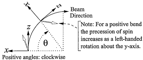
Figure 1: For the local coordinate system traveling with the beam, the z -axis points along the direction of the beam, y -axis points vertically (out of the page), and the x -axis points to the left thus forming a right-handed system. Clockwise bends (to the right) have a positive bend angle. The projection of the polarization in the horizontal plane is measured relative to the local z -axis.
