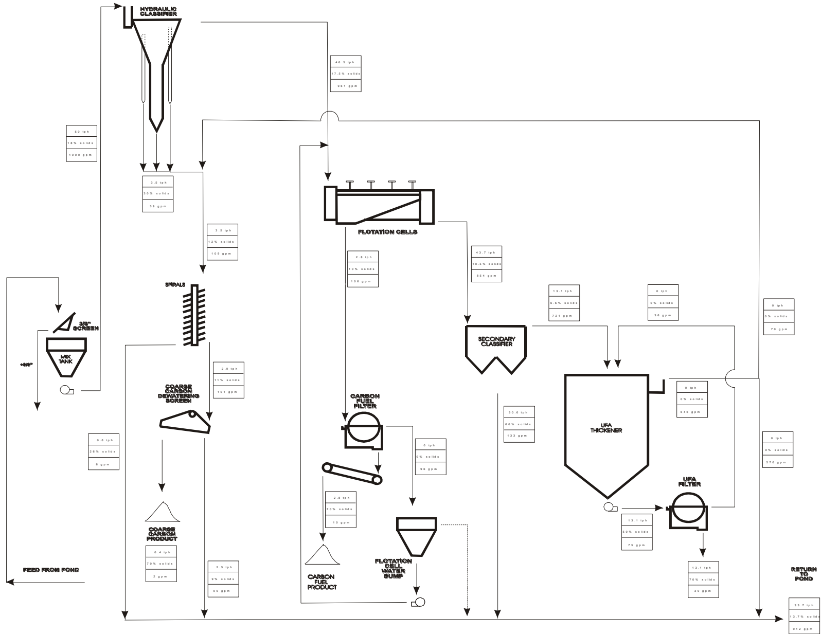
Figure 4. Process Flowsheet 4.
