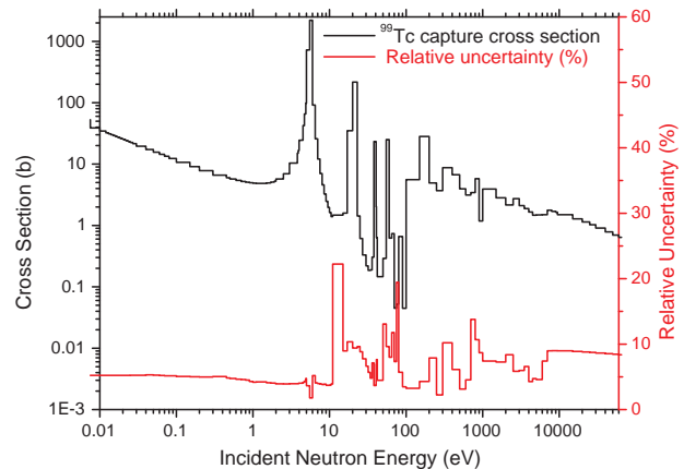
FIG. 64: Uncertainties of capture cross sections on ^{99}\text{Tc} obtained by the Atlas-KALMAN method in ENDF/B-VII.0 compared with the ^{99}\text{Tc}(n,\gamma) cross section. The left scale is for the cross section (black curve) and the right scale is for the relative uncertainty (red curve).
