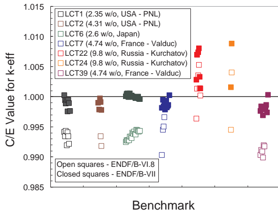
FIG. 98: LEU-COMP-THERM benchmark C/E values for k_{\text{eff}} for the ENDF/B-VI.8 and ENDF/B-VII.0 cross sections.
