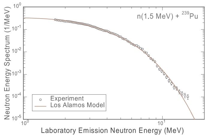
FIG. 32: Prompt fission neutron spectrum for 1.5 MeV neutrons incident on ^{239}\text{Pu} . The data of Staples [95] are shown together with the least-squares adjustment to the Los Alamos model.
