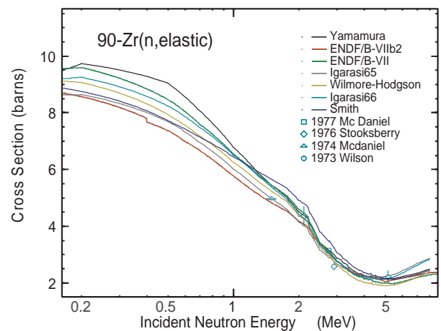
FIG. 59: Comparison of elastic cross sections on ^{90}\text{Zr} calculated with various optical model potentials. The preliminary ENDF/B-VII evaluation (denoted ENDF/B-VIIb2) yields the lowest cross sections. The final ENDF/B-VII evaluation is considerably higher, as suggested by the integral experiments.
