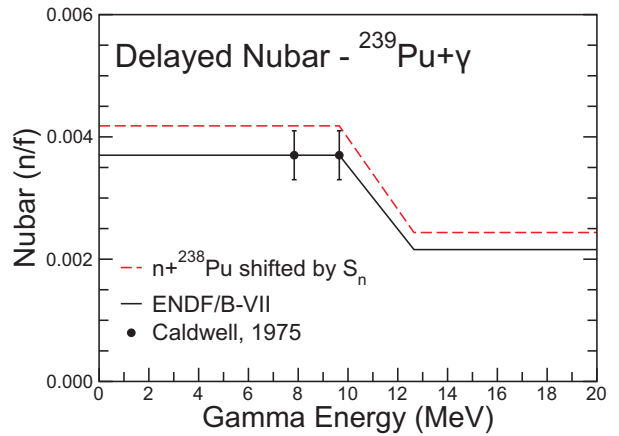
FIG. 81: Delayed nubar for photons incident on ^{239}\text{Pu} . Experimental data are for bremsstrahlung photons, data points refer to the average incident energy.
