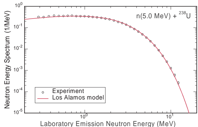
FIG. 22: Prompt fission neutron spectrum for 5.0 MeV neutrons incident on ^{238}\text{U} . The data of Lovchikova [82] are shown together with the least-squares adjustment to the Los Alamos model.
