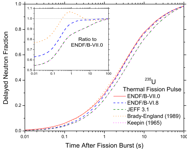
FIG. 47: Delayed neutron fraction as function of time following a ^{235}\text{U} thermal fission pulse for ENDF/B-VII.0, ENDF/B-VI.8, JEFF 3.1, Brady-England [148] and Keepin [149]. The inset shows the ratio of the delayed neutron fractions for the other evaluations to the ENDF/B-VII.0.
