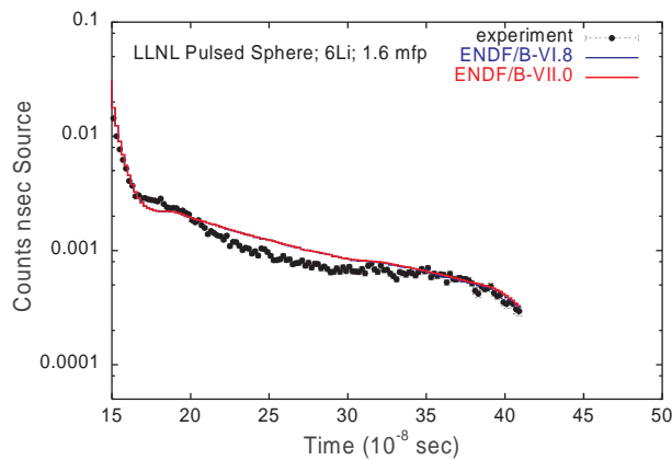
FIG. 112: Simulation of 14 MeV neutron transmission through 1.6 mfp {}^6\text{Li} at 30 degrees [277].
