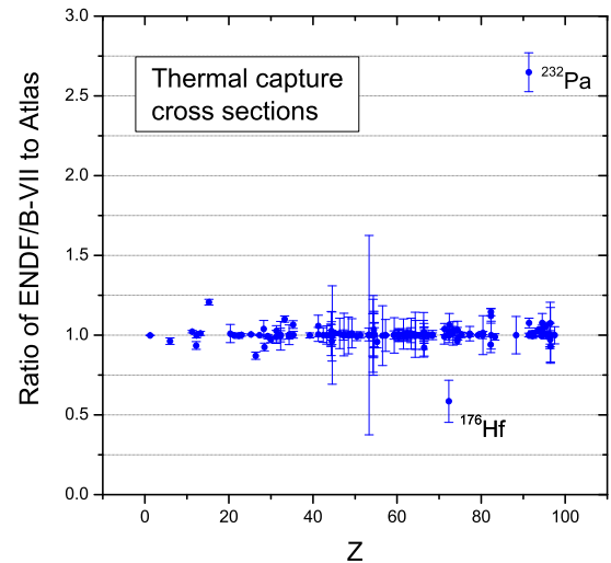
FIG. 117: Thermal neutron capture cross sections in ENDF/B-VII.0 compared to the Atlas of Neutron Resonances [30].
