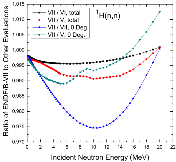
FIG. 67: The ENDF/B-VII.0 \text{H}(n,n) evaluation compared with the ENDF/B-VI and ENDF/B-V evaluations. The zero degree results are ratios of the center-of-mass-system cross sections at 180 degrees (which corresponds to zero degree protons in the laboratory system).
