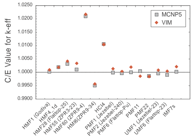
FIG. 104: C/E values for k_{\text{eff}} obtained with MCNP5 and VIM using ENDF/B-VII.0. Excellent agreement is seen between these two independent calculations.
