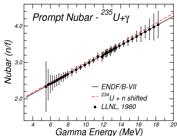
FIG. 76: Prompt nubar for photons incident on ^{235}\text{U} . Our evaluation uses the Caldwell data, LLNL.
