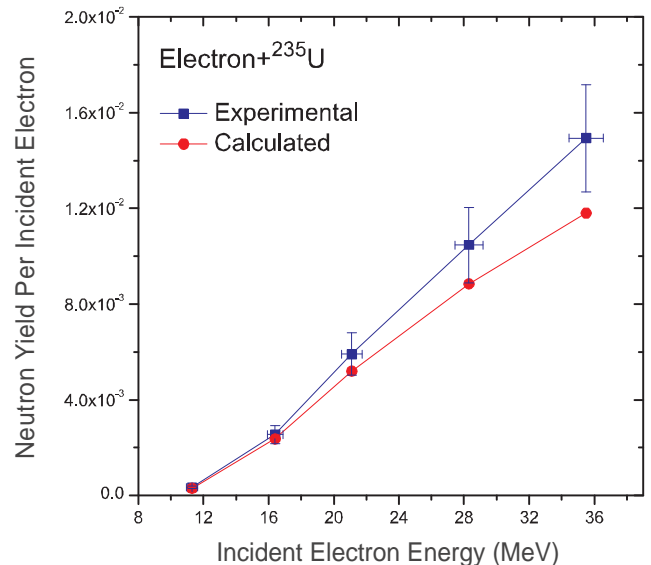
FIG. 83: Neutron yield per incident electron on a ^{235}\text{U} target.
