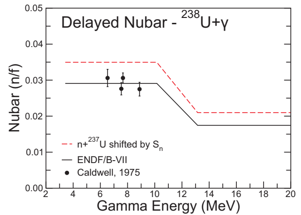
FIG. 80: Delayed nubar for photons incident on ^{238}\text{U} . Experimental data are for bremsstrahlung photons, data points refer to the average incident energy.
