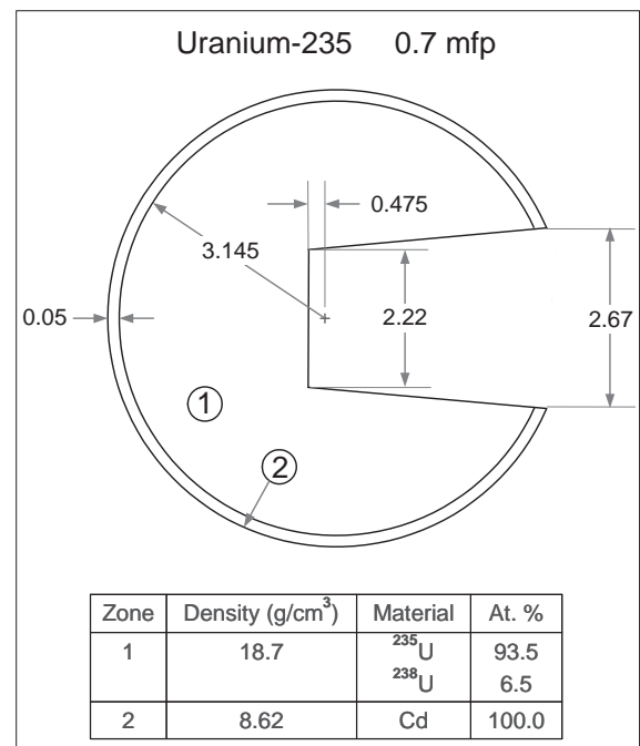
FIG. 113: Example sphere of {}^{235}\text{U} with a radius of 0.7 mean-free-path (mfp).
