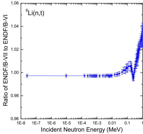
FIG. 68: The ENDF/B-VII.0 {}^6\text{Li}(n,t) evaluation compared with the ENDF/B-VI evaluation. The curve connects the central values of VII.0 to VI.8 ratios.
