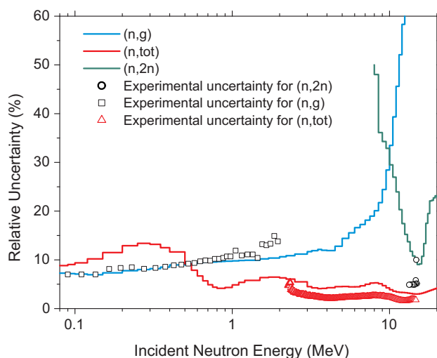
FIG. 65: Relative uncertainties on ^{193}\text{Ir} for the neutron total, (n,2n) and capture cross sections obtained with the EMPIRE-KALMAN method. The experimental uncertainties considered in the analysis are also included.
