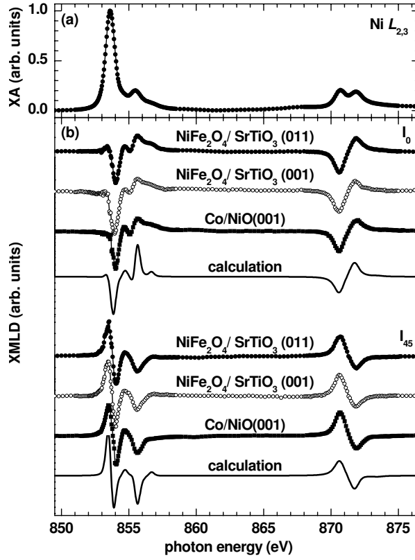
FIG. 2: Comparison of the experimentally obtained fundamental XMLD spectra together with results from atomic multiplet calculations. (a) Measured Ni L_{2,3} XA spectrum for NiFe 2 O 4 /SrTiO 3 . (b) Fundamental XMLD spectra I_0 i.e., \varepsilon=\mu=0^\circ (upper four spectra) and I_{45} i.e., \varepsilon=\mu=45^\circ (lower four spectra). Experimental data from NiFe 2 O 4 /SrTiO 3 (011) (solid circles), NiFe 2 O 4 /SrTiO 3 (001) (open circles) and Co/NiO(001) (solid squares). The multiplet calculations are shown by solid lines.
