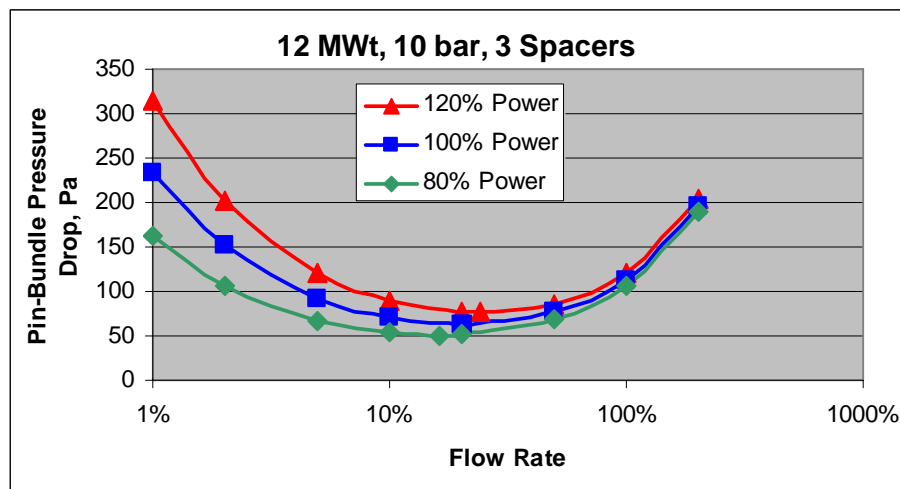
Figure 4.3b 10 bar
