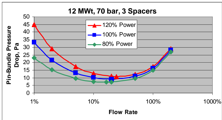
Figure 4.3a 70 bar
