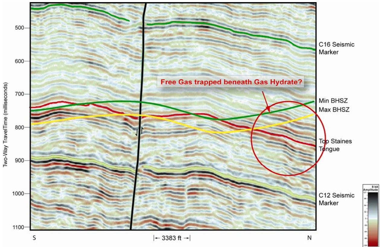
Figure 15. This seismic line is a color variable density display from the amplitude volume. The zone of interest is between the C16 Seismic marker (dark green) and the parallel green and yellow lines which represent the margin of error for the Base Gas Hydrate Stability Zone (BHSZ) horizon. The abrupt terminations of amplitude near the minimum base of the Hydrate Stability Zone (Min BHSZ) are interpreted as gas trapped by the hydrate.
