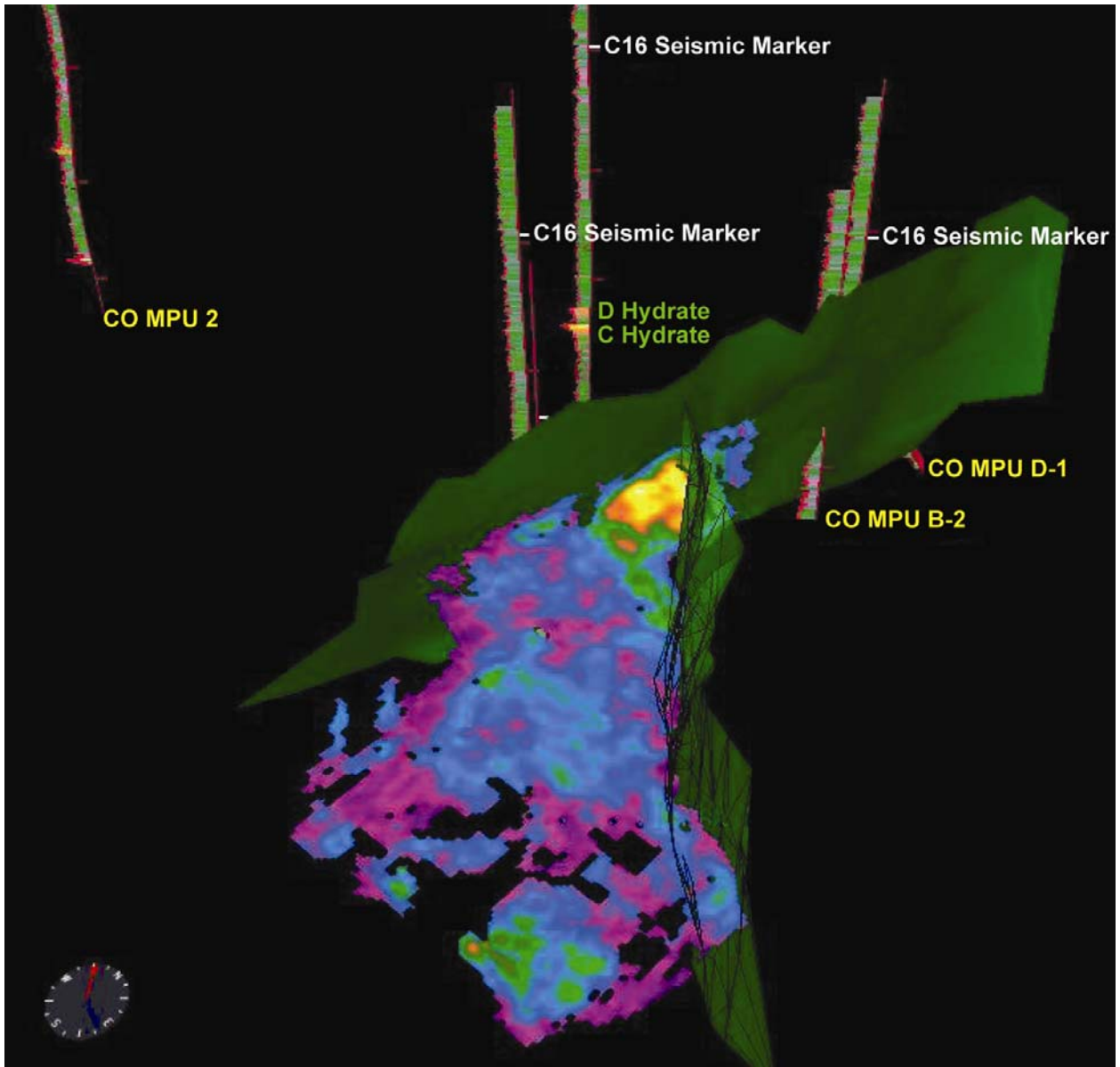
Figure 23. This 3-D display of the fault bounded Mt. Elbert prospect amplitude horizon shows the relationship of the anomaly to bounding faults and wells.
