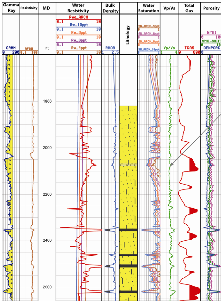
Figure 12. The log suite MPU S-15 well is shown with calculated petrophysical curves for water saturation ( S_w ) and water resistivity ( R_w ) at various salinities. Coals are found only in the interval below the Top Staines Tongue of the Sagavanirktok in this and other Milne Point wells.
