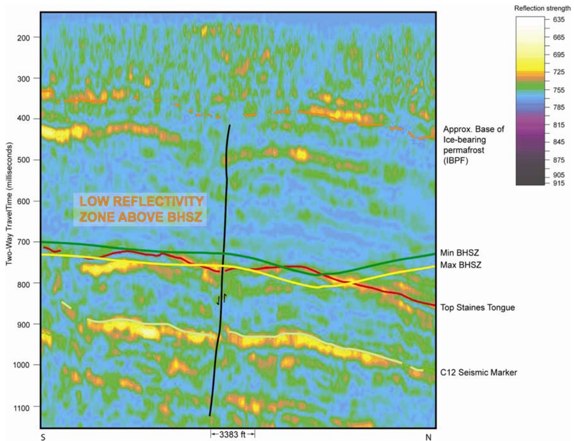
Figure 14. This seismic display is a line from a reflection strength volume. Parallel green and yellow lines depict the margin of error in the calculated Base Hydrate Stability Zone (BHSZ, from log data.).
