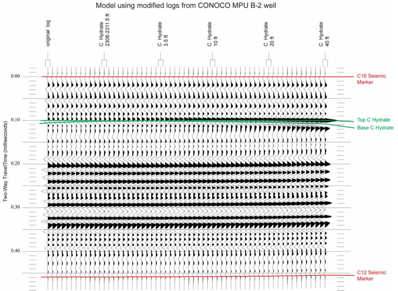
Figure 10. This model shows the seismic response to increasing hydrate thickness. Gas hydrate sections greater than about 20 ft thick show an obvious amplitude increase at the Top C Hydrate and Base C Hydrate with all other events remaining constant.
