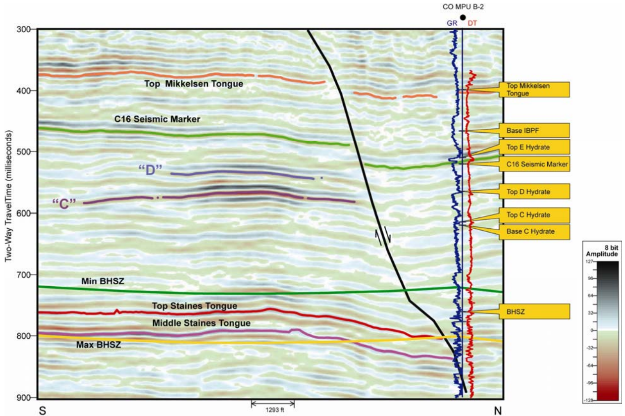
Figure 22. The CO MPU B-2 well tie, down-dip of Mt. Elbert C and D hydrate anomalies show thin hydrates identified on logs. These hydrates are below the detection limits of the seismic (less than 25 ft thick.) Amplitude anomalies in the up-thrown block correlate to these hydrates and are interpreted to be thicker, high saturation hydrates.
