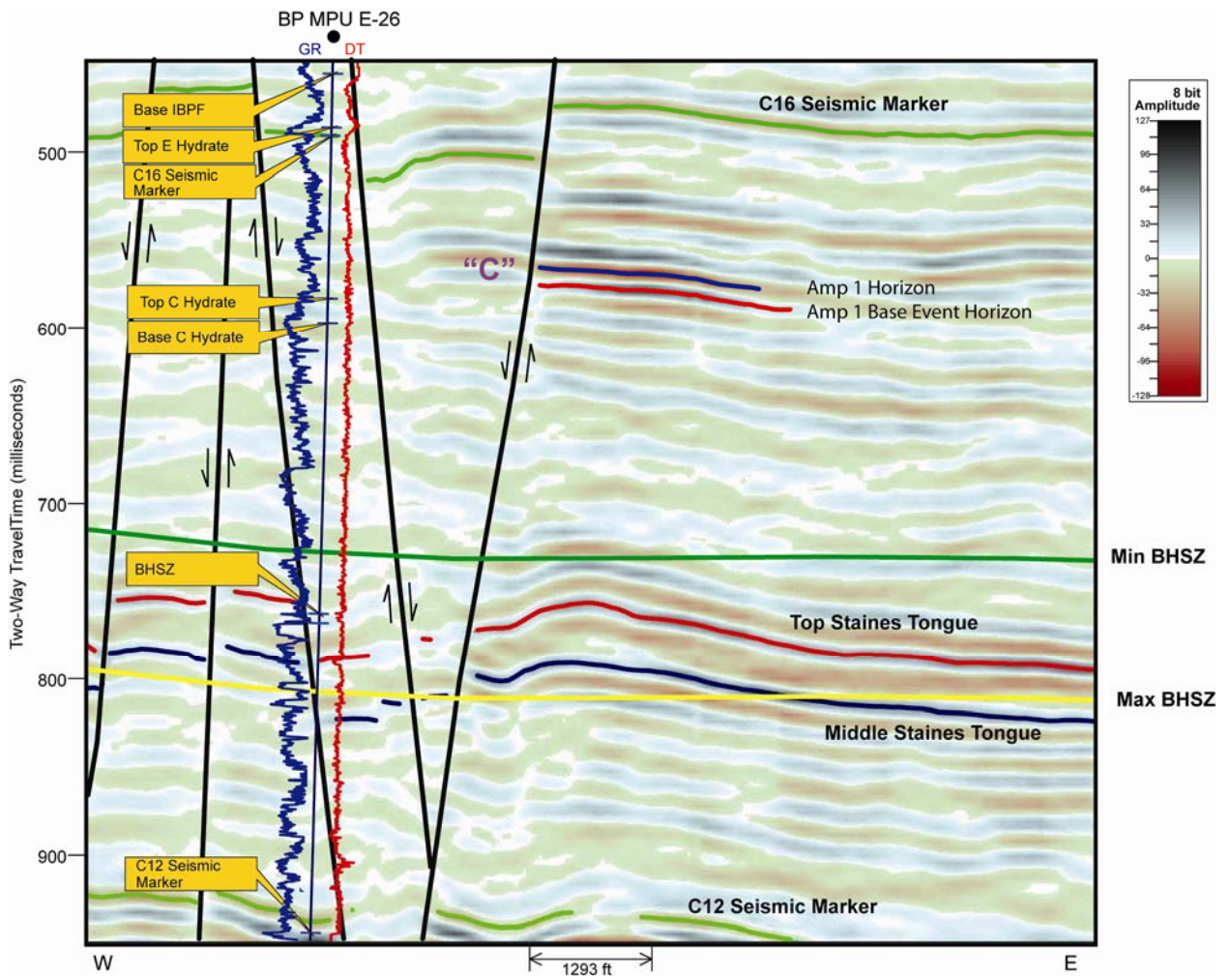
Figure 25. This display shows the Mt. Elbert “C” Hydrate events used in Lee’s saturation calculation. The Seismic line shows the tie across the fault to the BP MPU E-26 well.
