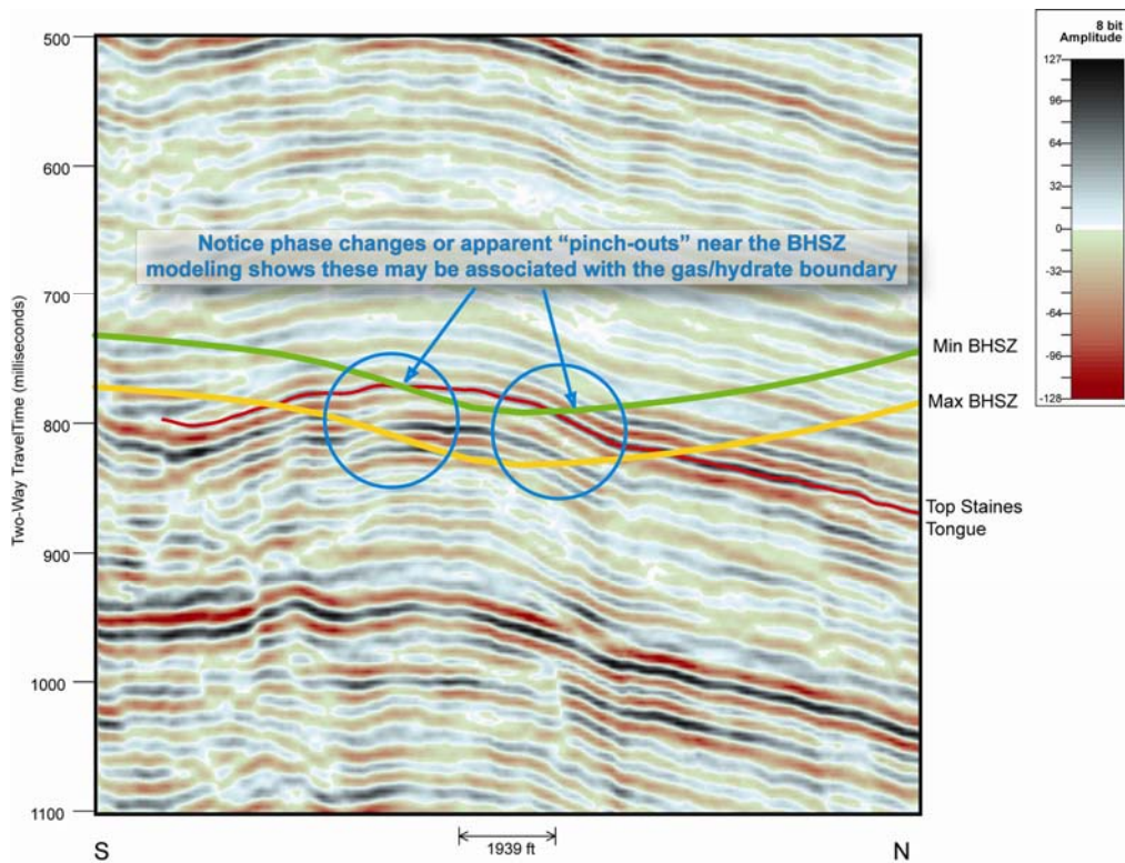
Figure 18. The minimum and maximum Base Hydrate Stability Zone events are shown relative to truncated high amplitude seismic reflections that are interpreted to be sub-hydrate free gas accumulations.
