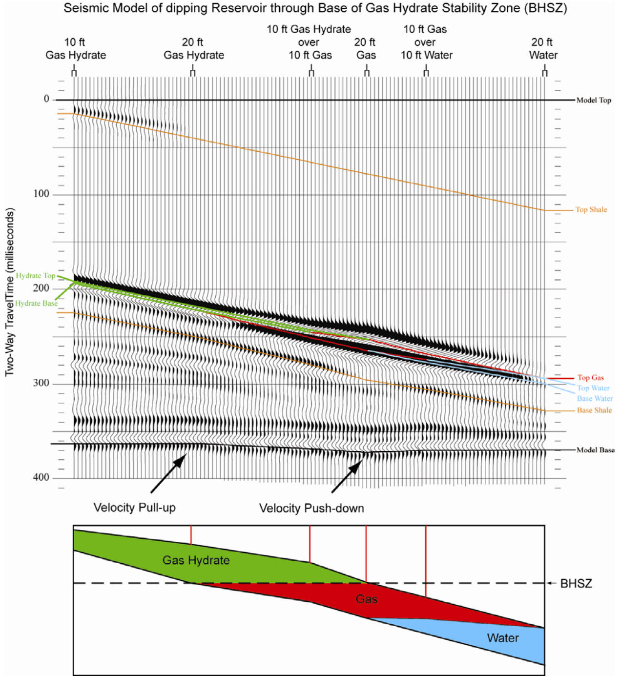
Figure 11. This model shows the trace response to a dipping model, at normal SEG polarity. The thin-bed response shows a phase change and amplitude change that is very similar to the actual seismic events near the Base Hydrate Stability Zone (BHSZ). The thick hydrate shows a pull-up and the gas a push-down on the flat model base related to velocity within the reservoir interval.
