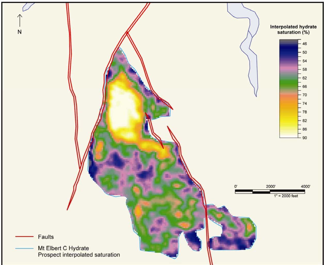
Figure 27. This display is a saturation map for the Mt. Elbert prospect. Saturations were derived using Lee's thin-bed analysis.
