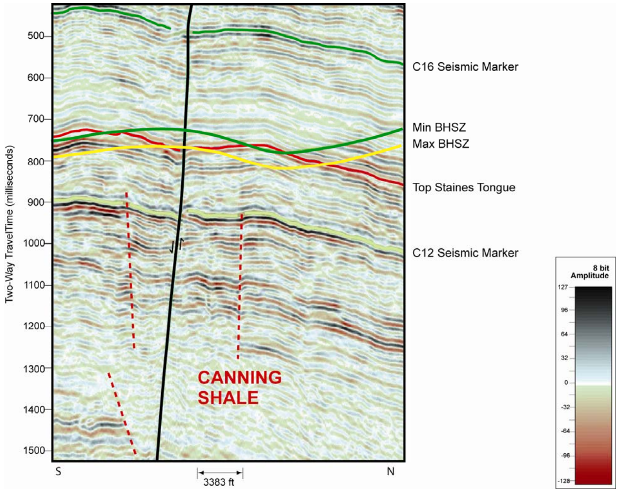
Figure 19. This seismic line shows the thick, nearly reflectionless, Canning Shale zone separating the Hydrate Stability Zone interval from the deeper Ellesmerian section that produces oil and gas in Milne Point, Kuparuk River and Prudhoe Bay fields. Some larger regional faults can be seen cutting this interval.
