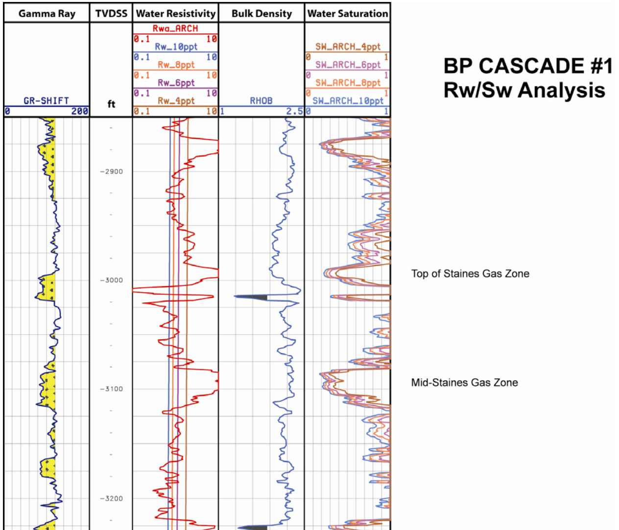
Figure 13. The log suite of the Cascade #1 well is shown with calculated petrophysical curves for water saturation (Sw) and water resistivity (Rw) at various salinities.
