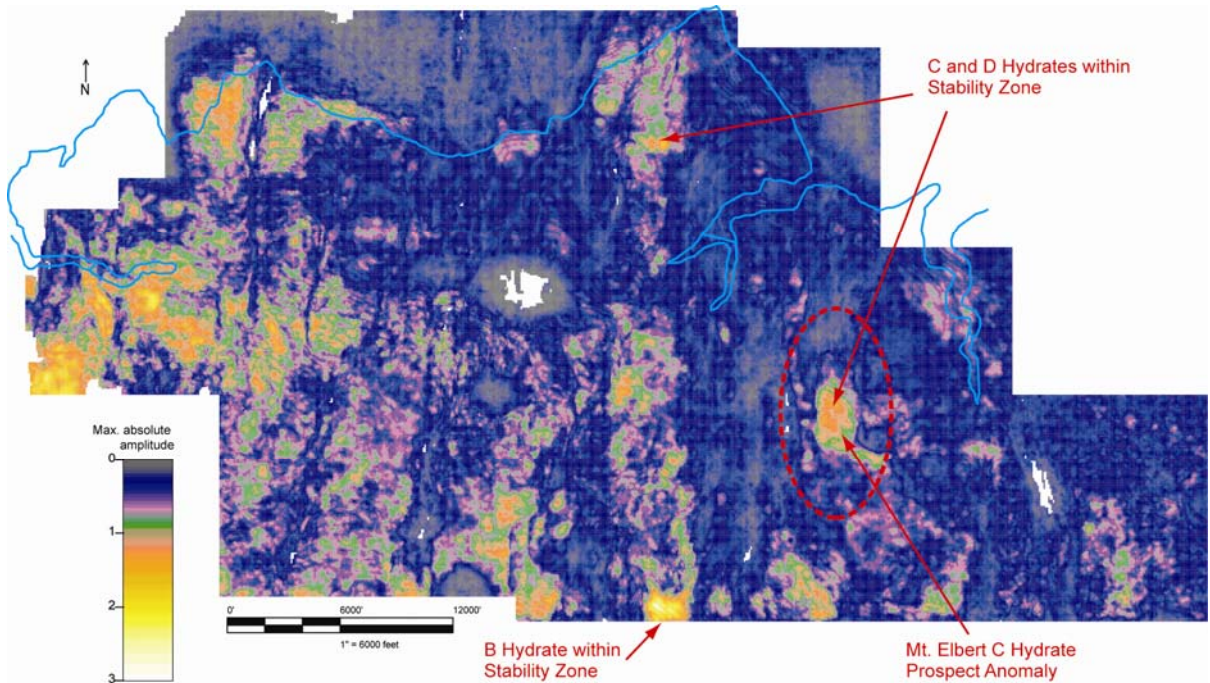
Figure 17. The Intra-Hydrate prospect reconnaissance map within the Gas Hydrate Stability Zone shows the Maximum absolute amplitude from 50 ms below the C16 Seismic Marker to 50 ms. above the Upper Staines Tongue Marker. Several areas of interest were identified, including the Mt. Elbert “C” hydrate anomaly.
