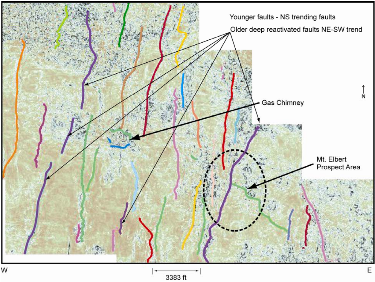
Figure 20. This display shows a shallow coherency timeslice with various fault trends. Older faults, trending more NE to SW, are more likely to be conduits for hydrocarbon migration.
