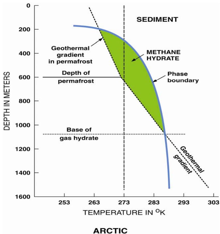
Figure 2. This graph is a phase diagram for the Hydrate Stability Zone in on-shore Arctic regions. Hydrates co-exist with permafrost in the interval between about 200 and 600 m. ( \approx 650-1970 ft) at Milne Point.
