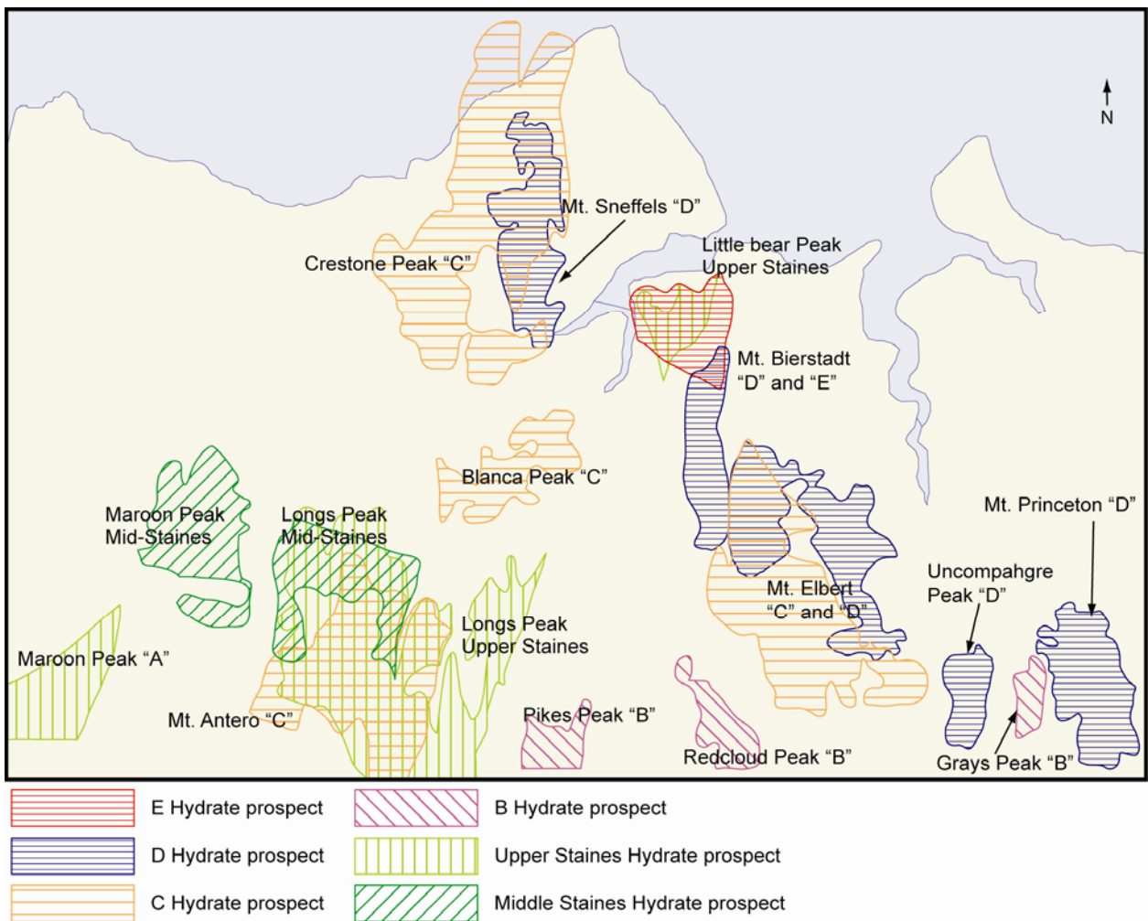
Figure 21. This display shows Milne Point gas hydrate prospects developed by 3D seismic analysis.
