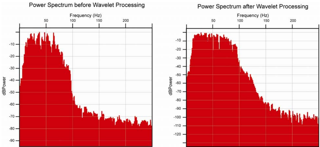
Figure 8. USGS reprocessing improved the power spectrum of the 3D seismic data, increasing the over-all frequency within the zone of interest and whitening the spectrum. This display is a comparison, within the shallow Hydrate Stability Zone, before and after wavelet reprocessing.
