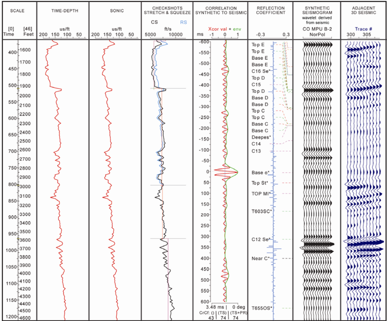
Figure 7. This synthetic seismogram to seismic tie panel for the CO MPU B-2 well shows the excellent tie between the synthetic seismogram and correlative piece of 3-D seismic at the well. Minimal stretch was required for the tie.
