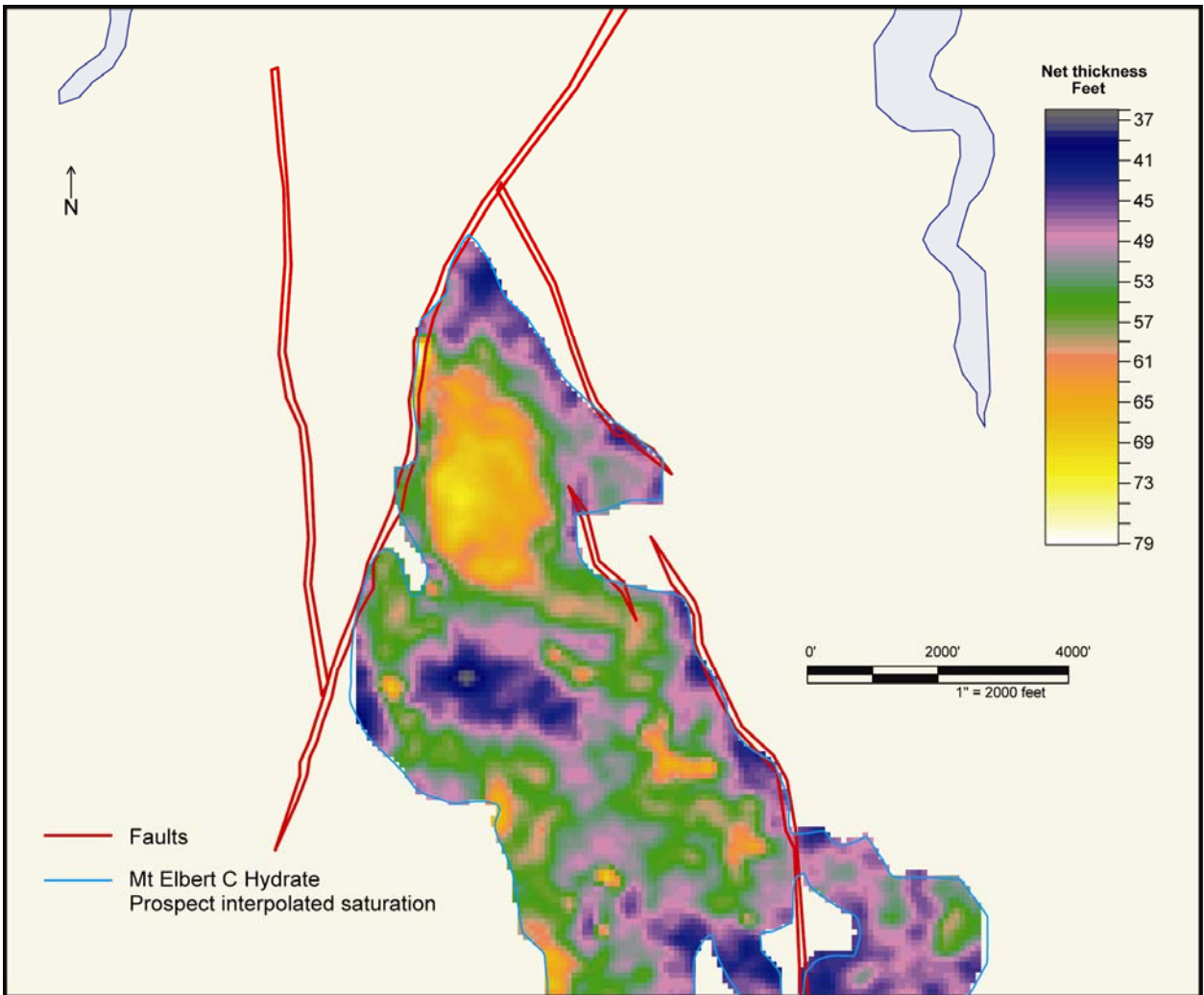
Figure 26. This display is a thickness map for the Mt. Elbert prospect. Thicknesses were derived using Lee's thin-bed analysis.
