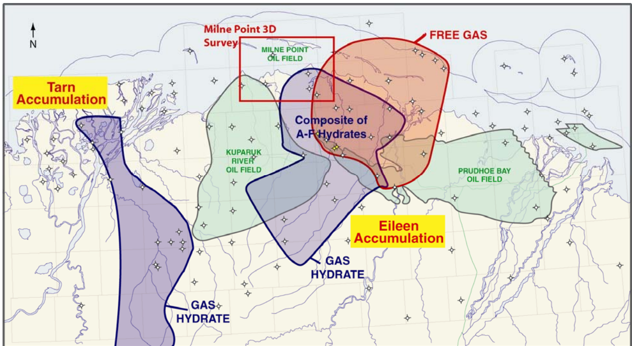
Figure 1. This map shows the Milne Point 3-D study area and identified gas hydrate accumulations. The Milne Point study area is in the northern-most part of the “Eileen Accumulation”. The study area is adjacent to the prolific Kuparuk River and Prudhoe Bay oil fields.
