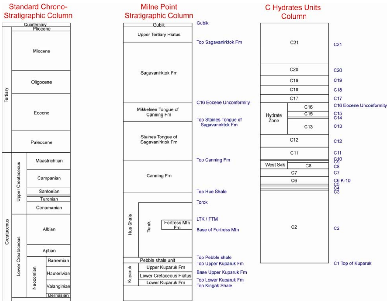
Figure 4. Stratigraphic columns used in the Milne Point study showing regional stratigraphic markers and their relationship to Gas Hydrate “C” picks developed by Collett (1993).
