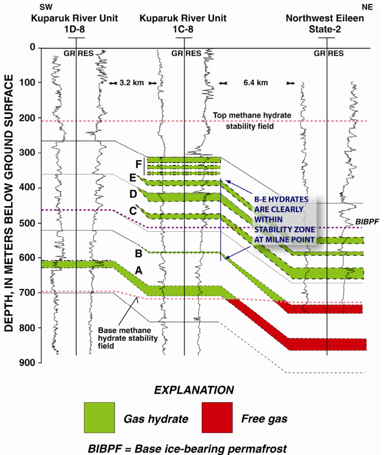
Figure 5. Gamma ray and resistivity logs from the Kuparuk River area showing the Eileen gas hydrate accumulation (Units A-F) (modified from Collett, 1993).
