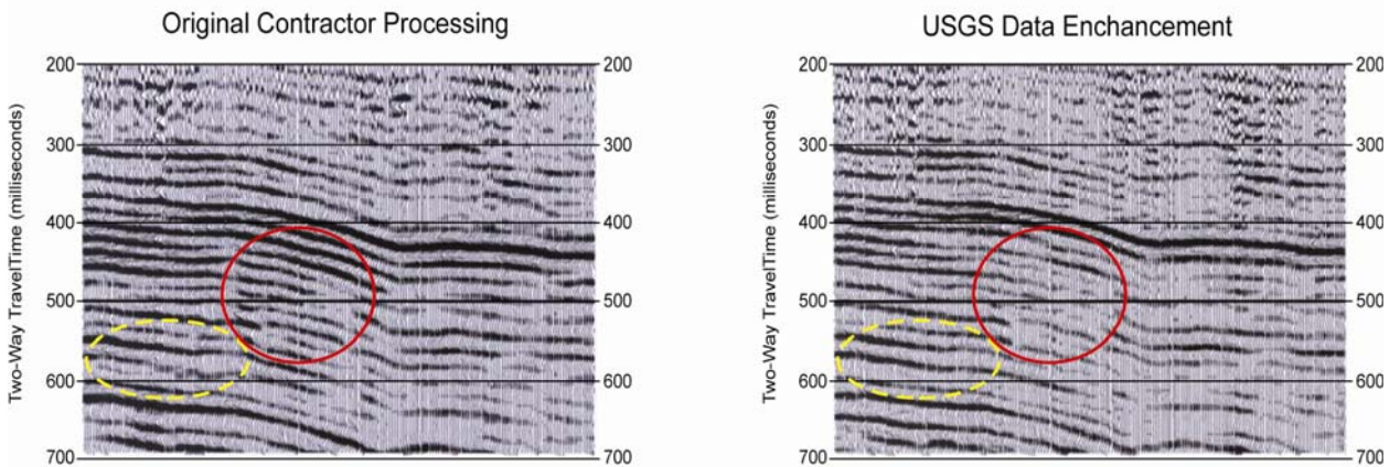
Figure 9. The display shows an example line before and after USGS wavelet reprocessing. The yellow outlined area shows where the USGS signature wavelet deconvolution sharpens the wavelet and broadens the frequency spectrum. The red outlined area show where the USGS predictive deconvolution suppressed interbed multiple reflections.
