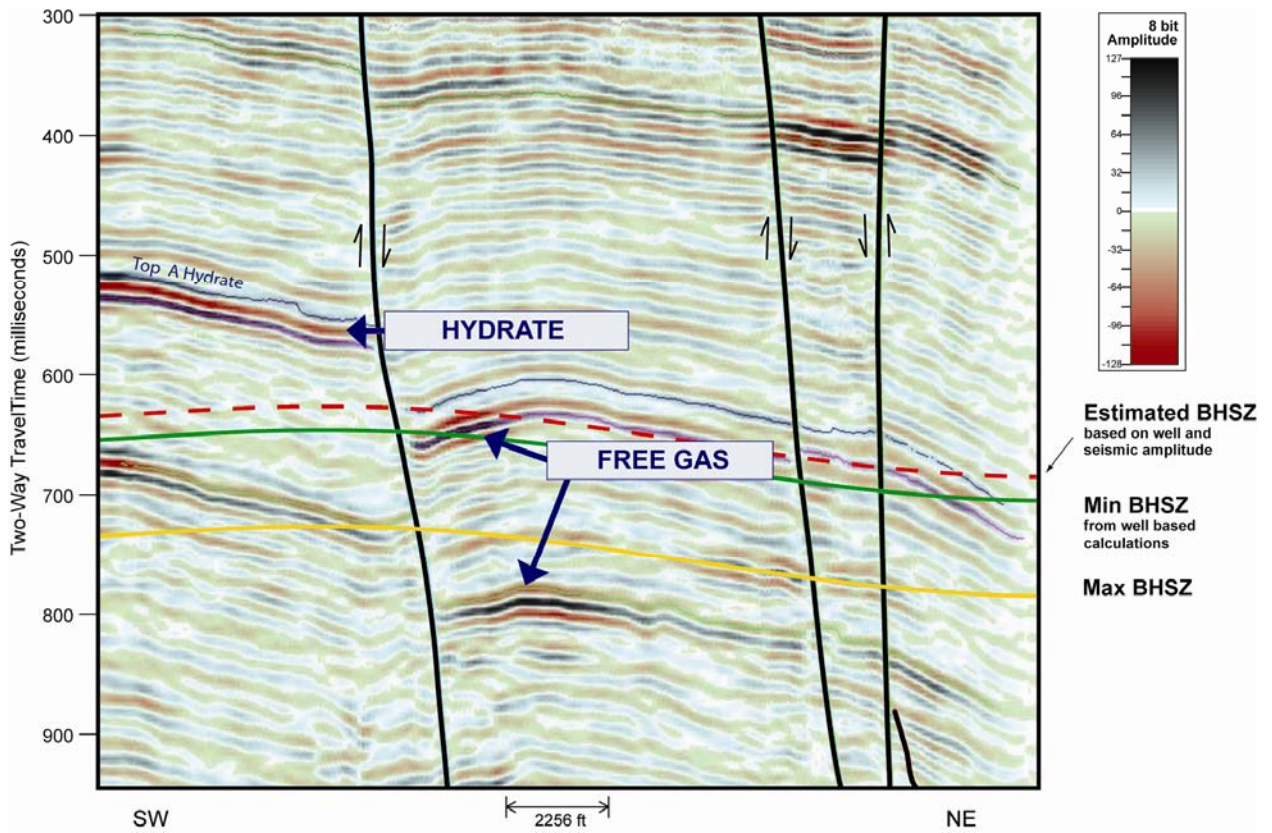
Figure 24. The Maroon Peak free gas and gas hydrate prospects are shown by amplitude and phase variations. The “Free Gas” anomalies are represented by a peak, and the “Hydrate” in the up-thrown block is represented by a trough on this reverse SEG polarity data.
