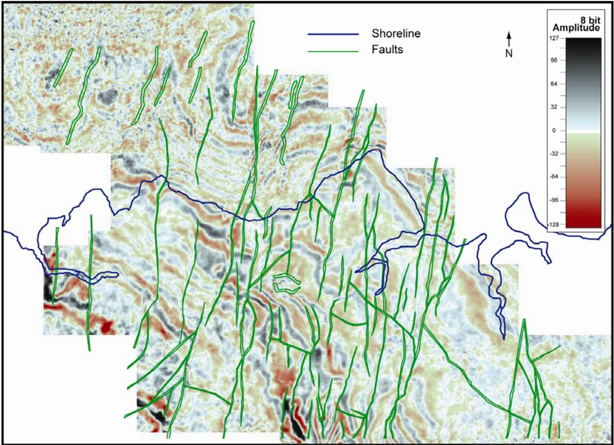
Figure 3. Map shows Milne Point area faulting at approximately the Top of the Staines Tongue of the Sagavanirktok Formation. The Top Staines Tongue is near the Base of the Hydrate Stability Zone over much of the survey. The gas hydrate study was limited to the on-shore portion of the seismic survey.
