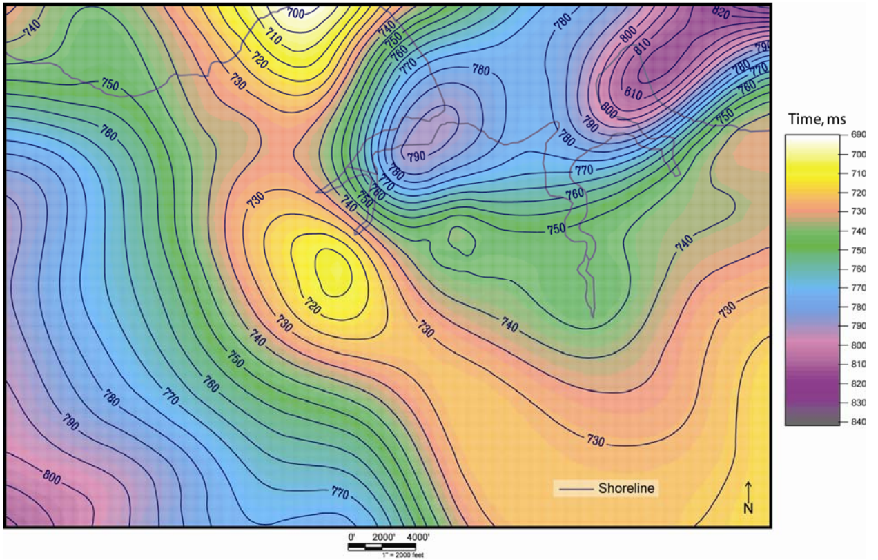
Figure 6. This map shows the BHSZ time structure map for the Milne Point study area generated using well derived temperature data and IBPF picks from well logs data.
