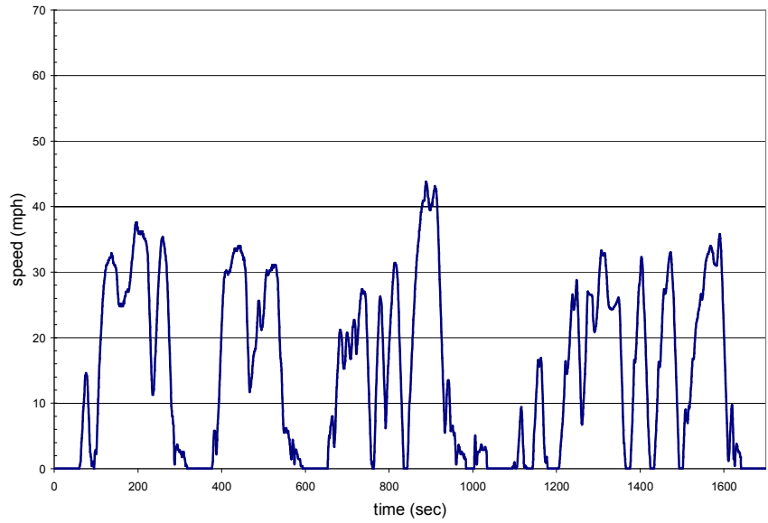
Figure 6. The CSHVC cycle.
