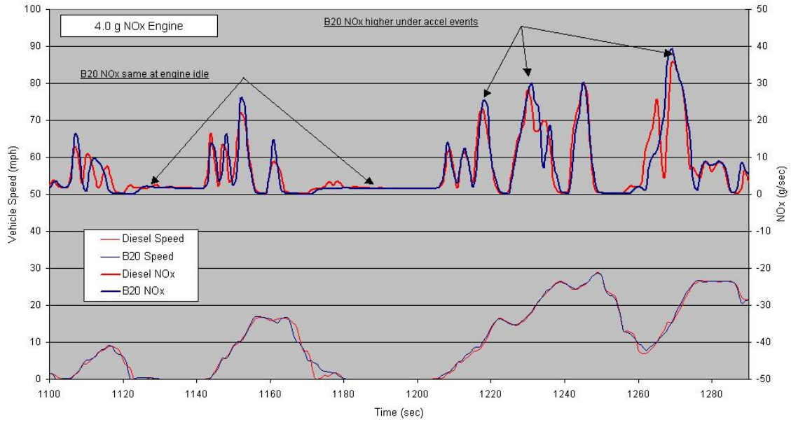
Figure 16. Portions of the CSHVC real-time NO x traces for the Freightliner Class 8 truck.
