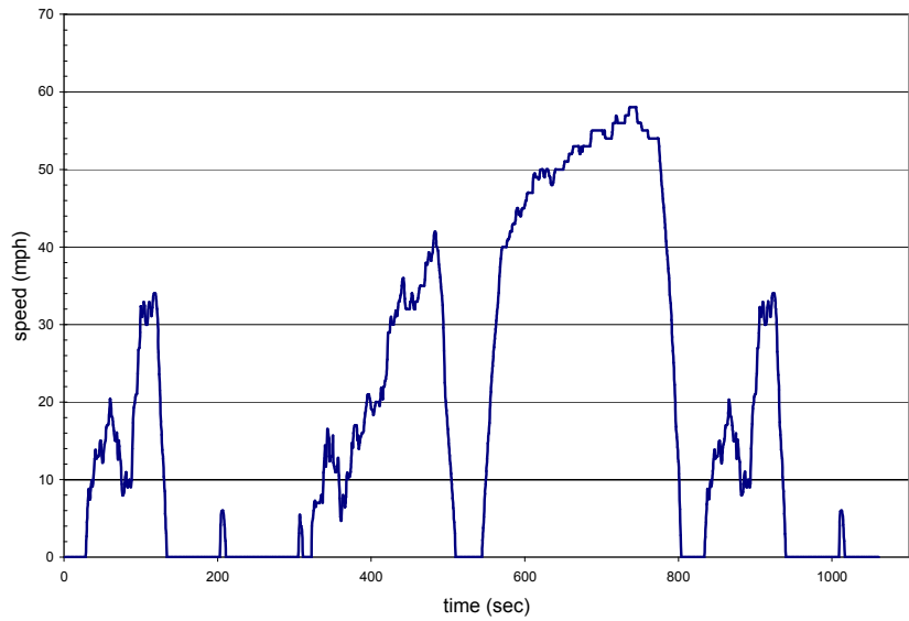
Figure 7. The UDDS cycle.
