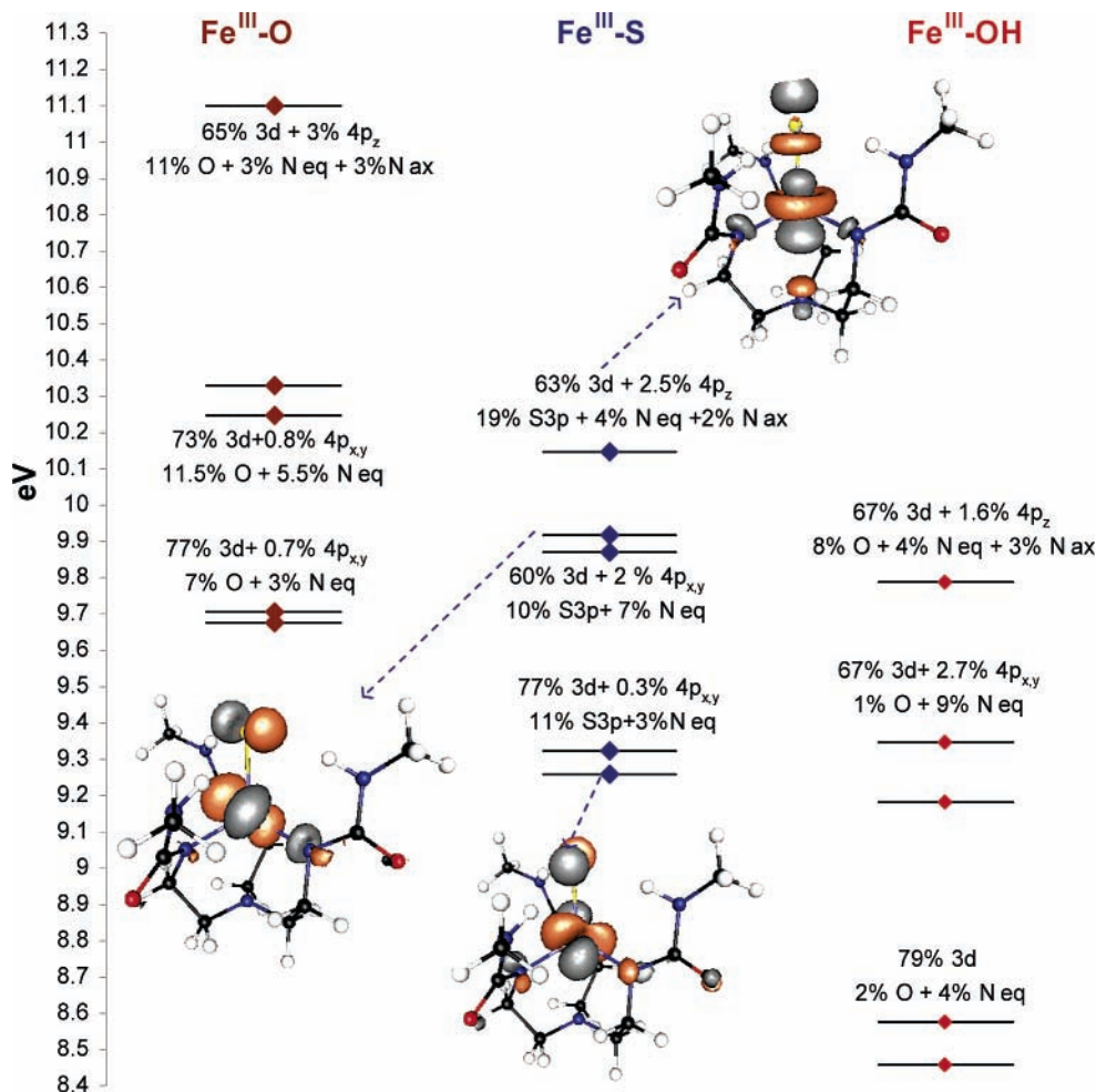
Figure 5. MO diagram of [Fe III H 3 buea(O)] 2- , [Fe III H 3 buea(S)] 2- , and [Fe III H 3 buea(OH)] - showing the \beta -unoccupied orbitals. The coefficients (average values for the E set) of Fe 3d (3d), Fe 4p (4p), X np (np), N ax 2p (N ax ), and N eq 2p (N eq ) and representative contour diagrams for individual sets of d orbitals are given.
