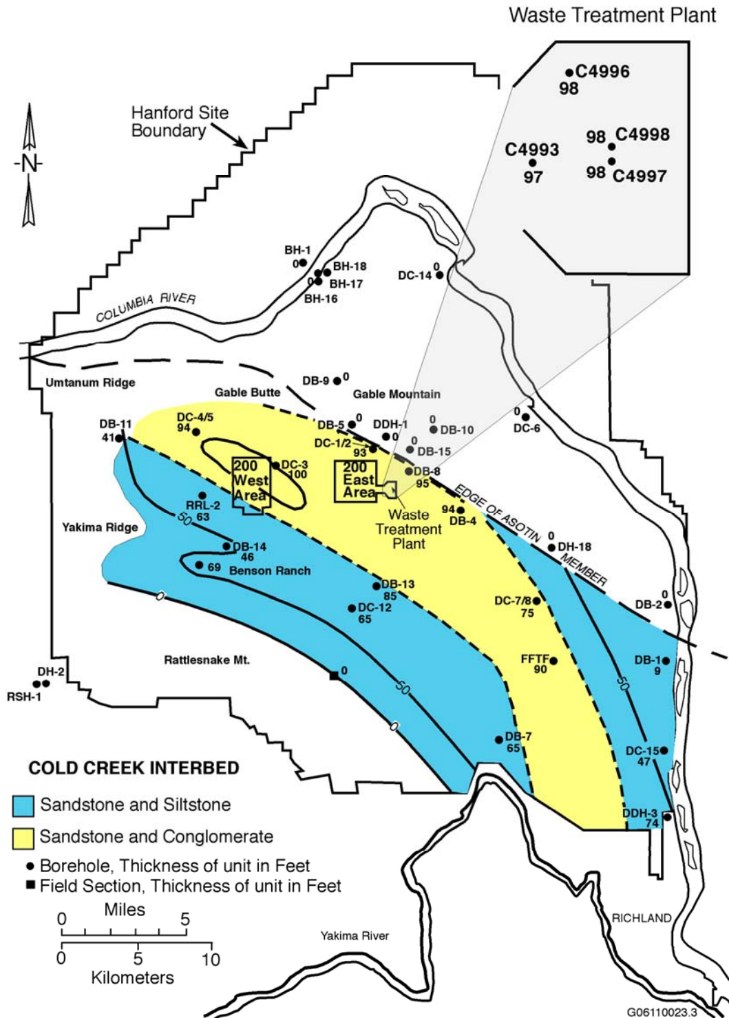
Figure 5.2. Cold Creek Sedimentary Interbed Thickness on the Hanford Site and at the Waste Treatment Plant Site
