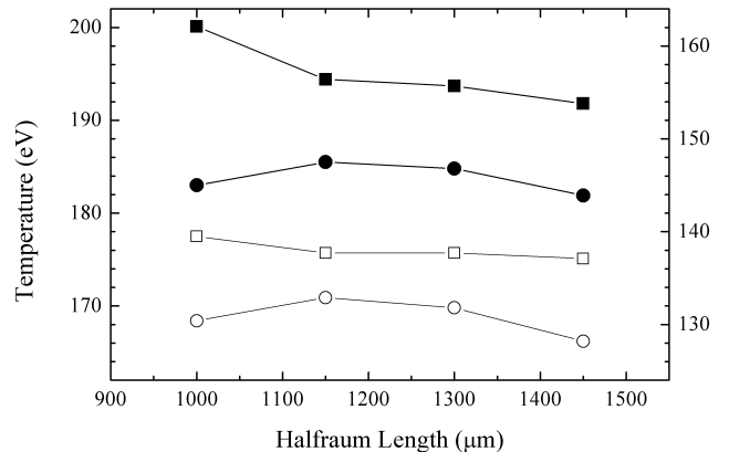
FIG. 18: Temperature as a function of halfraum length for the four simulations shown in Fig. 17, with all simulations having identical beam pointings with respect to the LEH. The solid symbols are from a simulation time of t = 1.0 ns (left-hand axis) while the open symbols are from t = 100 ps (right-hand axis). The squares are DANTE temperatures and the circles are sample radiation temperatures.
