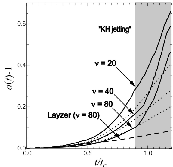
FIG. 8: Comparison of normalized bubble heights in the frame moving with the interface from the HYDRA simulation of Fig. 7 (solid line), the WKB solution of Eq. (9) (dotted line), and the Layzer prediction (dashed line). The shaded region marks the onset of KH vortex generation, jet formation by vortex interference, and subsequent bubble acceleration. Results for modes \nu = 20 and 40 are also shown.
