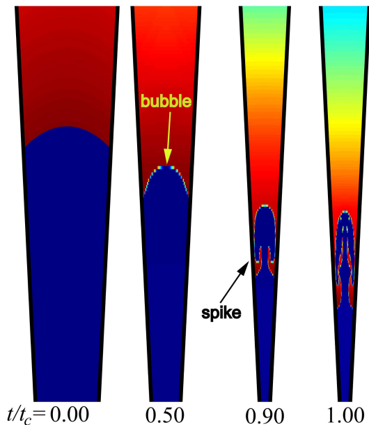
FIG. 7: Snapshots of bubble growth from a HYDRA simulation of RT growth during the deceleration phase with \nu = 80 . Each snapshot is centered approximately about the location of the bubble apex at the corresponding time. The color scale gives the fluid density with red the dense shell and blue the low-density gas.
