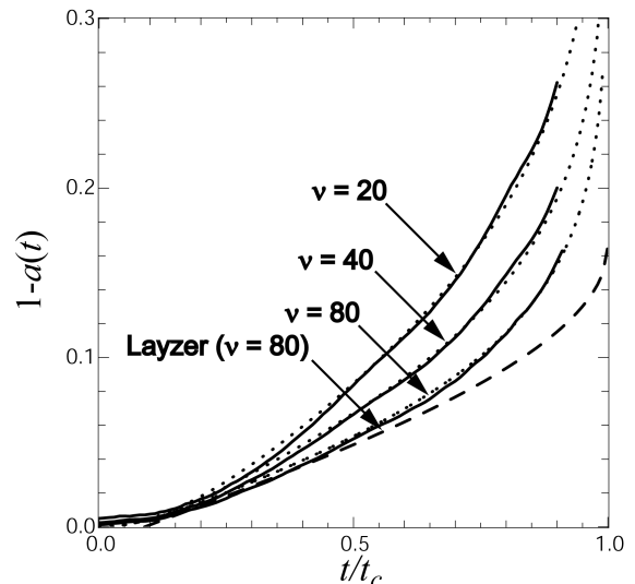
FIG. 4: Comparison of normalized bubble heights in the frame moving with the interface from the HYDRA simulation of Fig. 3 (solid line), the WKB solution of Eq. (9) (dotted line), and the Layzer prediction (dashed line). Results for modes \nu = 20 and 40 are also shown. Here and below the length scale has been normalized to the initial shell radius, i.e. , R_0 \equiv 1 .
