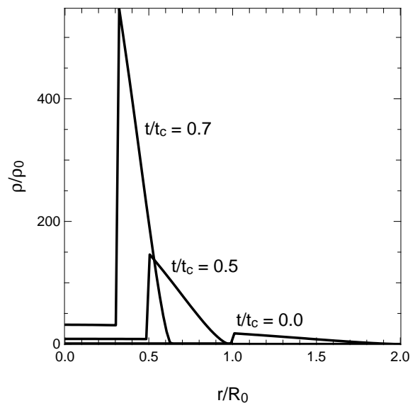
FIG. 6: Sequence of radial density profiles corresponding to a decelerating, Kidder-type implosion. The density scale has been normalized by the density at r = 0 and t = 0 . An initial aspect ratio of R_{\text{out}}/R_0 = 2.0 at t = 0 has been chosen, which corresponds to an Atwood number at the shell-gas interface of \mathcal{A} = 0.90 .
