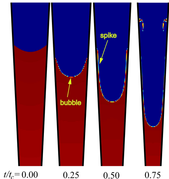
FIG. 3: Snapshots of bubble growth from a HYDRA simulation of RT growth during the acceleration phase with \nu = 80 . Red denotes the dense fluid and blue the low-density pusher. To illustrate the bubble evolution, each snapshot is centered approximately about the location of the bubble apex at the corresponding time.
