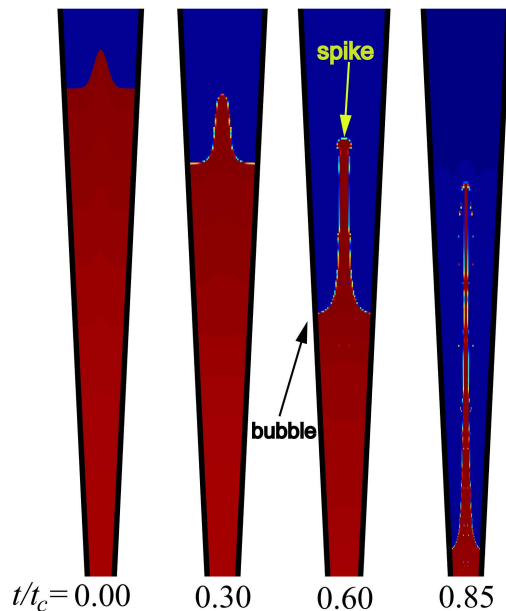
FIG. 9: Snapshots of spike growth from a HYDRA simulation analogous to Fig. 3. The simulation is run identically to Fig. 3 but with a spike-type initial interface shape instead of a bubble-type shape.
