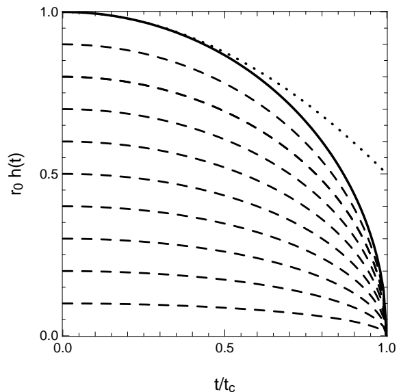
FIG. 1: Implosion diagram of an accelerating, Kidder-type implosion. The interface trajectory is shown as the solid line, and sample fluid particle trajectories as the dashed lines. For comparison, the trajectory of a constant acceleration or “free-falling” implosion is shown by the dotted line.
