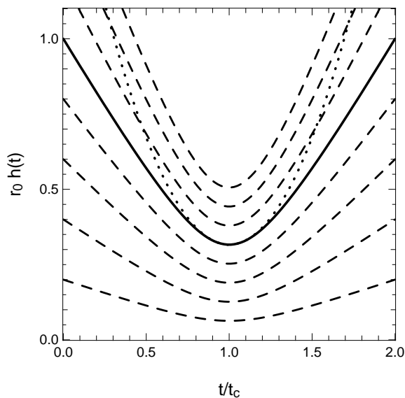
FIG. 5: Implosion diagram of a decelerating, Kidder-type implosion with initial implosion velocity of c = -0.9 . The interface trajectory is shown as the solid line, and sample fluid particle trajectories as the dashed lines. For comparison, the dotted line shows the trajectory of a “free-falling” implosion decelerating at the peak deceleration of the self-similar case.
