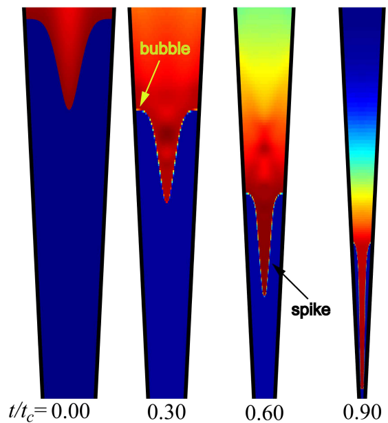
FIG. 11: Snapshots of spike growth from a HYDRA simulation analogous to Fig. 7 but with c = -0.95 , \mathcal{A} = 0.95 , and a spike-type initial interface shape. Each snapshot is centered approximately about the location of the spike tip at the corresponding time.
