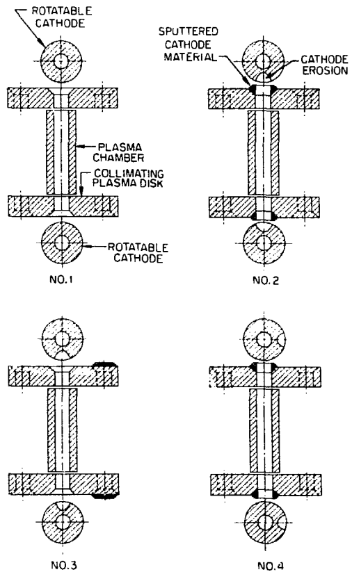
Fig. 4. Views of the rotatable cathodes, the plasma chamber, and the collimating plasma discs during an experiment to find the cause of beam increase as the source ages are shown. (1) The cathodes and collimating discs at the beginning of an ion source burn. (2) The eroded cathodes and the collimating discs with sputtered tantalum when the beam intensity has increased. (3) Rotation of the plasma collimators produced the same beam intensity as obtained in view 2. (4) Rotation of the cathodes resulted in operating at the initial beam intensity as obtained in view 1.
