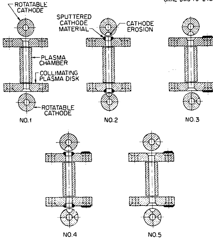
Fig. 5. Five views are shown of the rotatable cathodes, collimator discs, and plasma chamber for a proposed mode of operation to increase the cyclotron beam intensity. (1) The cathodes and collimating discs at the beginning of an ion source burn. (2) The eroded cathodes and the collimating discs with sputtered tantalum near the end of an ion source burn. (3) The collimators and only one cathode are rotated for the next burn. This cathode arrangement allows the arc to be struck easily and also results in increased beam near the end of the source life. (4) The cathodes and collimator discs near the end of the second burn. (5) The cathodes and collimator discs positioned for the beginning of the third burn.
