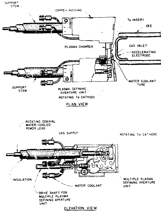
Fig. 1. A schematic drawing of the source head of the rotatable cathode ion source. The cathodes can be rotated and the plasma collimator has multiple apertures which can be changed remotely.
