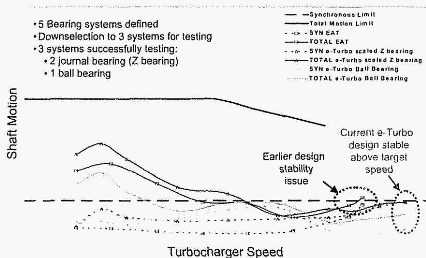
Figure 10: Bearing system selection to resolve shaft motion issue with e-Turbo™
