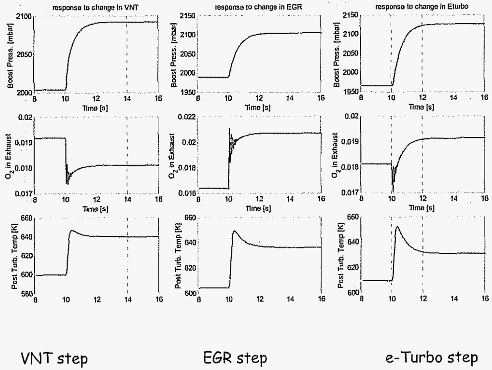
Figure 47: Step changes in VNT, EGR, and e-Turbo power from left to right and resulting O 2 and engine turbine out temperature below each. Shows potential to control O 2 and temperature into DPF and that it may be possible to light-off DPF without burning additional fuel.
