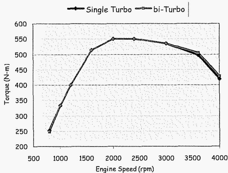
Figure 32: Simulated baseline (no e-Turbo™) torque characteristics of a 4.0 liter diesel engine equipped with bi-turbo and single turbo configurations
