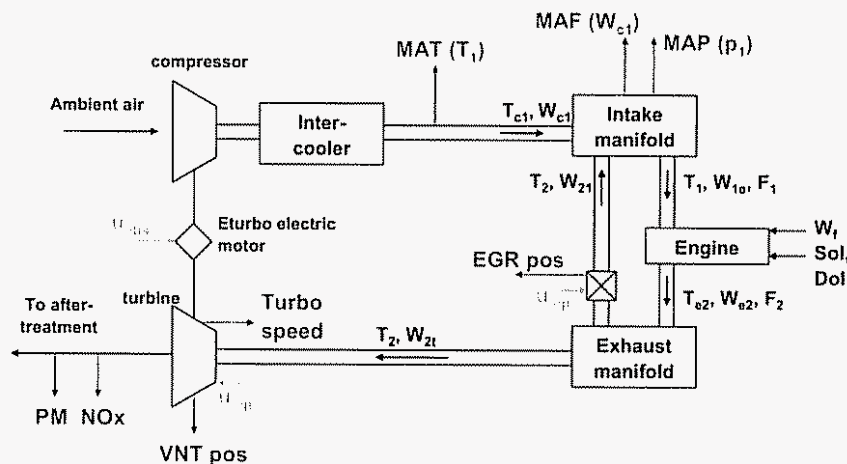
Figure 42: Sensing and control architecture for e-Turbo™
