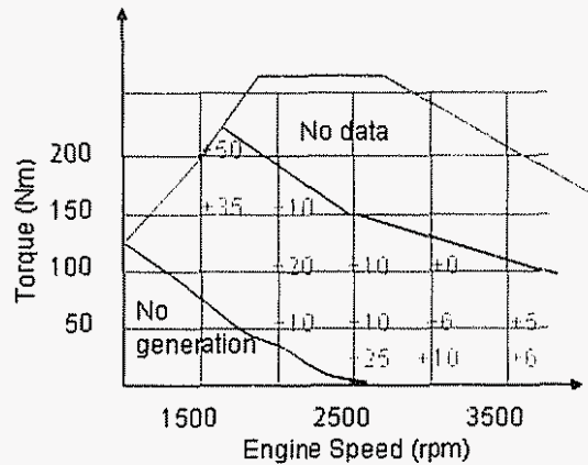
Figure 48: Possible exhaust temperature increase with 250 W of power generation with e-Turbo™ under various load-speed conditions
