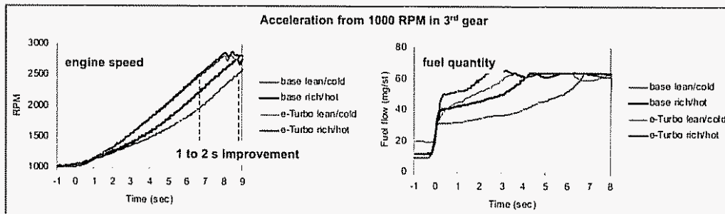
Figure 25: Transient response of e-Turbo™ diesel engine powered passenger vehicle in third gear
