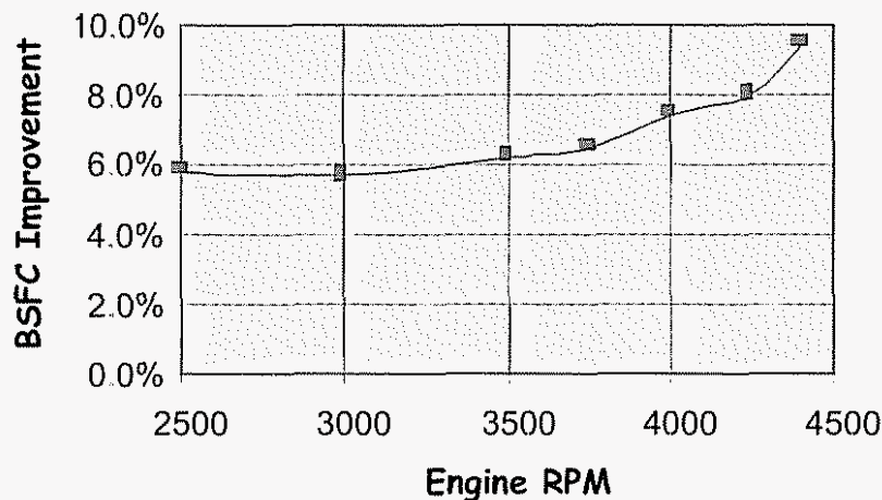
Figure 11: Simulated brake specific fuel consumption (BSFC) improvement with electrical power generation
