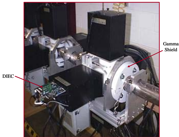
Fig. 7. The FMFM detector assembly showing the DIEC and the gamma shield.
