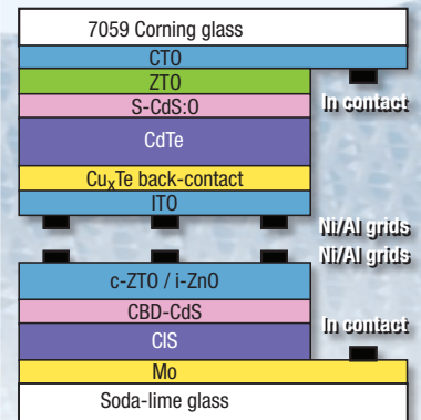
This CdTe-CIS multijunction cell developed under the EM&D project demonstrated a record 15.3% sunlight-to-electricity conversion efficiency.
