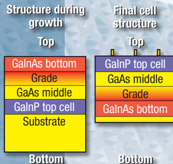
In the inverted cell configuration, the top layer is grown on a substrate at the bottom of a stack of additional layers (left). After growth, the original substrate is removed, the layers are turned upside down, and the electrical contacts are applied to what is now the top layer (right).
