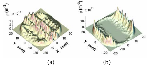
Figure 4: Clearing effect in a dipole magnet of ILC positron damping ring with (a) 0V and (b) -100V. Bunch intensity is 2\times 10^{10} and bunch spacing is 6 ns.
