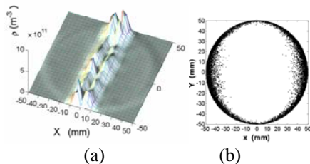
Figure 1: Electron distribution in a dipole magnet of KEKB LER with 0 (a) and -400 V (b) clearing field.
