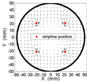
Figure 5: Configuration of electrodes and clearing field in a quadrupole magnet.
