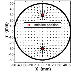
Figure 2: Configuration of electrodes and a clearing field in a dipole magnet.
