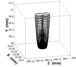
Figure 3: Electron's orbit in a dipole magnet with a clearing field .
