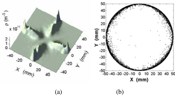
Figure 6: Effects of a 4 electrodes clearing system in a quadrupole magnet with clearing potential 0V (a) and -100V (b).
