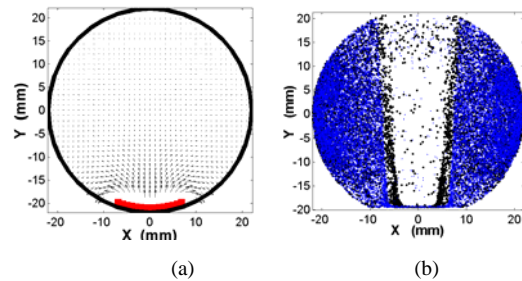
Figure 7: Clearing field (a) and effect (b) of a traditional stripline electrode. The red color in (a) shows the electrode. The blue and black dots in Fig. 7(b) show the electrons with different size of the electrode.
