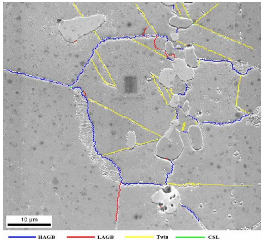
Fig. 4.115: Different boundary types overlaid on the SEM figure indicate the GB migration associated with discontinuous precipitation in Alloy 230. \epsilon_{tot} = 1.0\%
