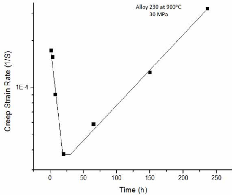
Fig. 4.122: (c) Creep strain rate for Alloy 230 with an applied stress of 30 MPa at 900°C
