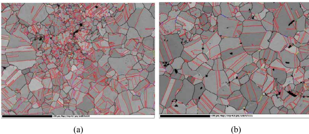
Fig. 3.28: EBSD and CSL boundary analysis of the materials in the as-received condition: (a) Alloy 617; (b) Alloy 230
