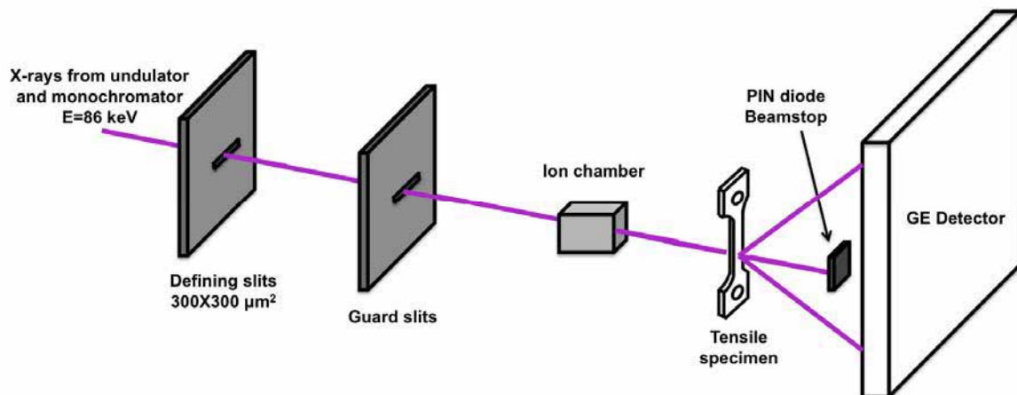
Fig. 3.4: Schematic of the experimental diffraction setup
