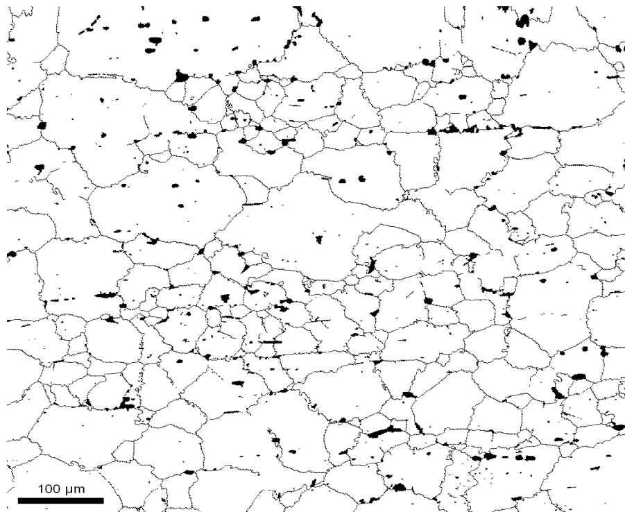
Fig. 4.108: Grain boundary character distribution of aged Alloy 230. (a) Dark lines are HAGBs, and light grey lines are CSL boundaries; (b) HAGB network after removal of CSL boundaries
