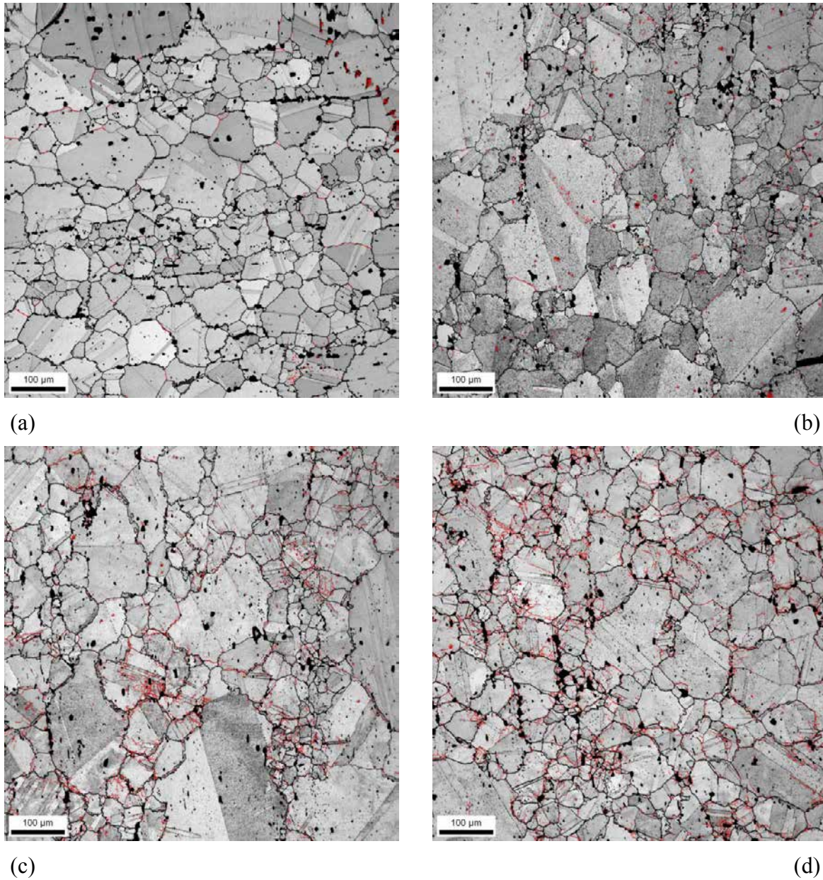
Fig. 4.109: LAGB distribution highlighted by red lines for different Alloy 230 samples. Test conditions: (a) aged; (b) \epsilon_{tot} = 1.0\% ; (c) \epsilon_{tot} = 1.5\% ; (d) \epsilon_{tot} = 1.0\% , dwell time = 3 minutes; (e) \epsilon_{tot} = 1.5\% , dwell time = 3 minutes; (f) \epsilon_{tot} = 1.0\% , dwell time = 30 minutes
