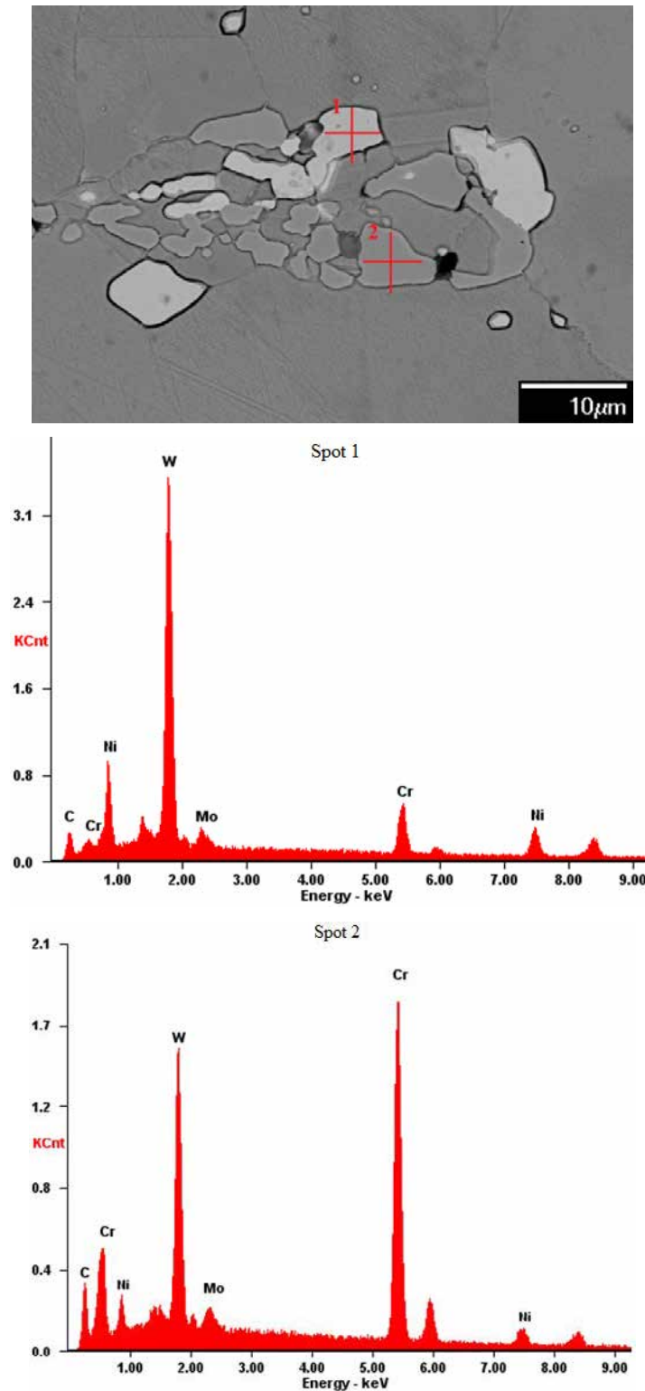
Fig. 4.78: The morphology and composition of precipitates in the as-received Alloy 230. The EDS spectrum was taken from the highlighted point in the SEM figure. (a) spot 1: W-rich M_6C and spot 2: Cr-rich M_{23}C_6 ; (b) GB Cr-rich M_{23}C_6 precipitate
