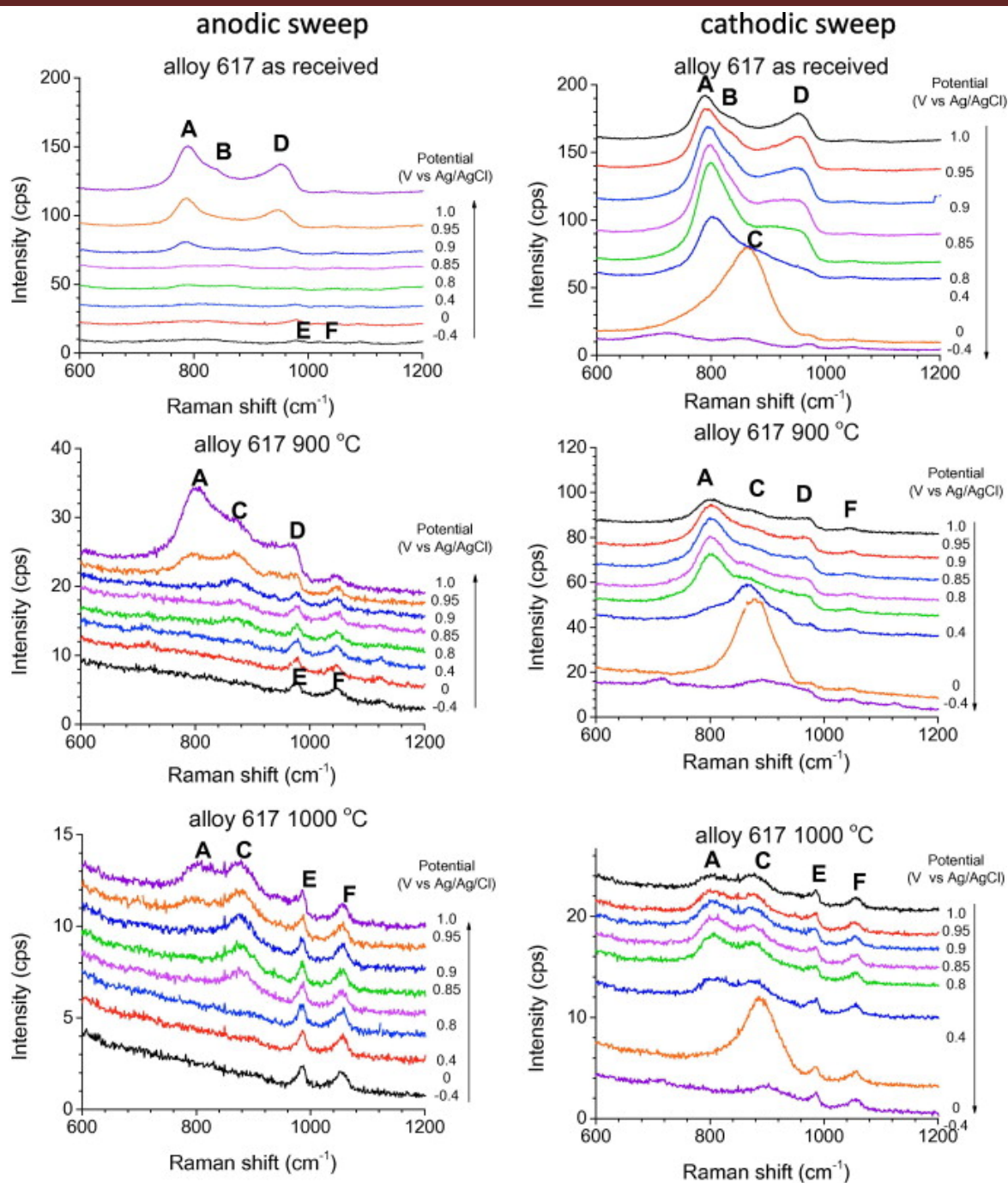
Fig. 4.139: Potential dependent spectra of Ni alloys in 0.1 M H 2 SO 4 . Spectra offset for clarity.
