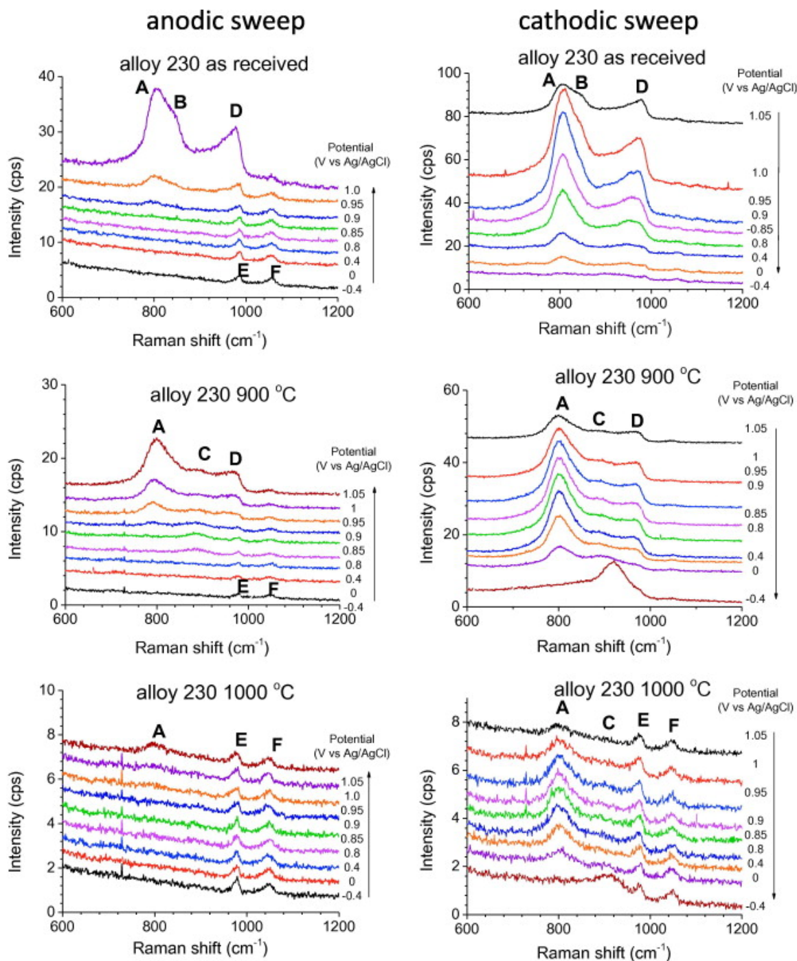
Fig. 4.141: Potential dependent spectra of Alloy 230 in 0.1 M H 2 SO 4 . Spectra offset for clarity.
