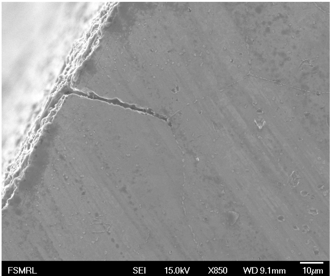
Fig. 4.123: (a) Cross-sectional view of pressurized creep tubes near the fracture surface under the applied stress of 35 MPa at 900°C for Alloy 230
