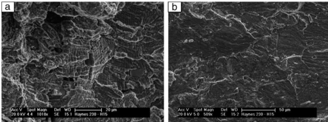
Fig. 4.135: (a) High-magnification SEM micrograph showing the fatigue striations on the 900°C specimen; (b) post-fracture surface of the 900°C specimen showing a low level of oxidation and a smooth surface indicative of intragranular fatigue crack growth
