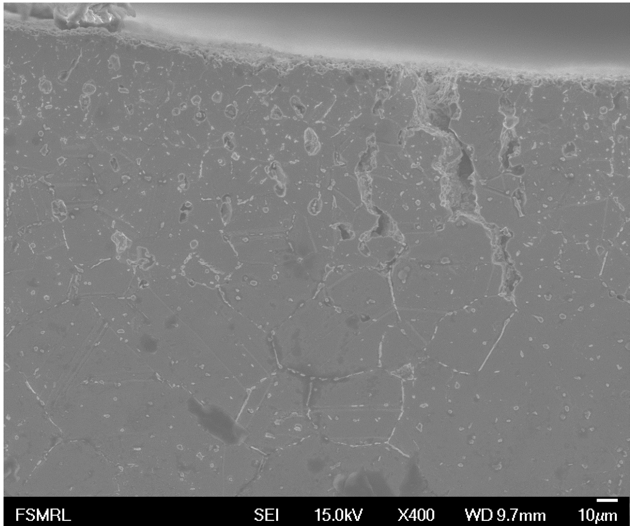
Fig. 4.120: (a) Cross-sectional view of pressurized creep tubes near the fracture surface under the applied stress of 30 MPa at 900°C for Alloy 617
