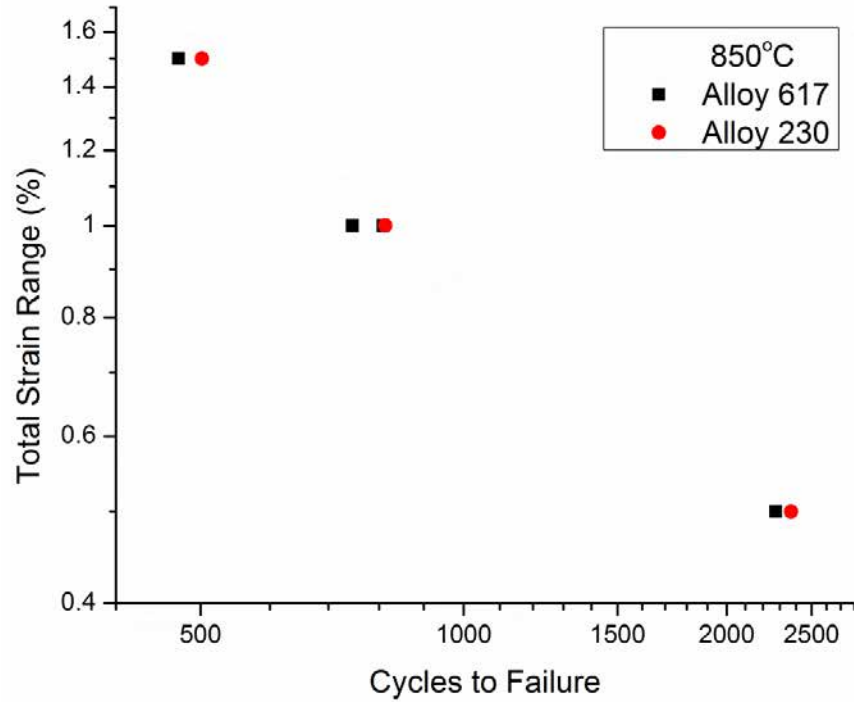
Fig. 4.65: LCF life of Alloy 617 and Alloy 230 tested at 850°C. The failure criterion was based on a 40% maximum tensile stress decrease in (a), and on a 20% stress ratio drop in (b).
