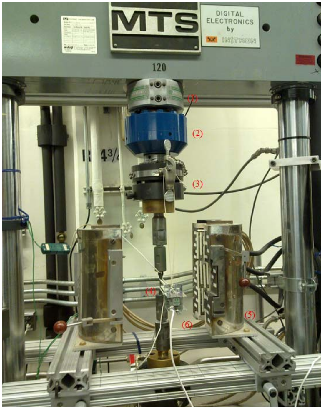
Fig. 3.13: First set of creep-fatigue test frames. Detailed item description: (1) alignment fixture; (2) load cell; (3) specimen grips; (4) specimen; (5) furnace; (6) high temperature extensometer
