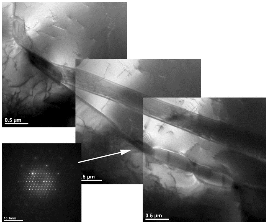
Fig. 4.33: TEM analysis of Alloy 617 aged at 1000°C for 300 hours; an intergranular precipitate (P) with an orientation relation with the matrix (M): [-114]_M // [011]_P
