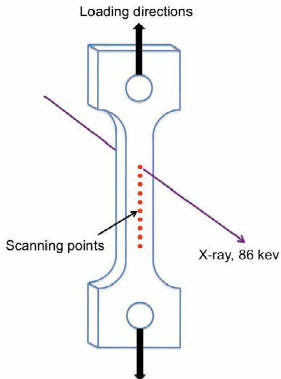
Fig. 4.51: Schematic of axial-scanning measurements
