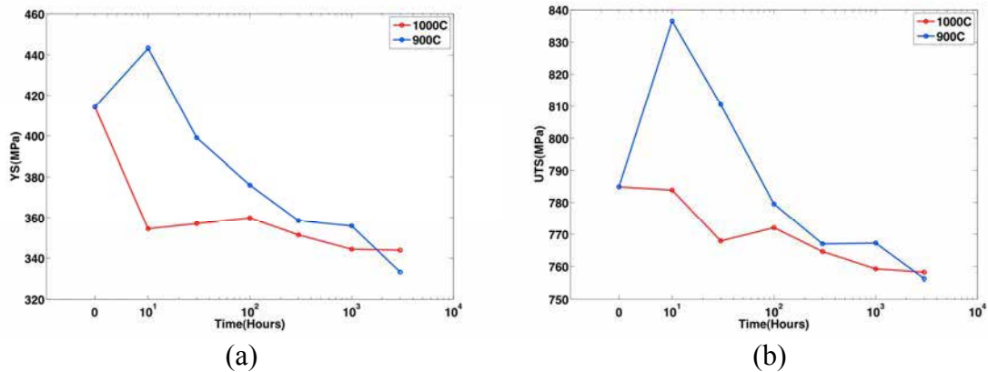
Fig. 4.46: Tensile properties for the as-received and aged Alloy 617: (a) Y.S.; (b) U.T.S.
