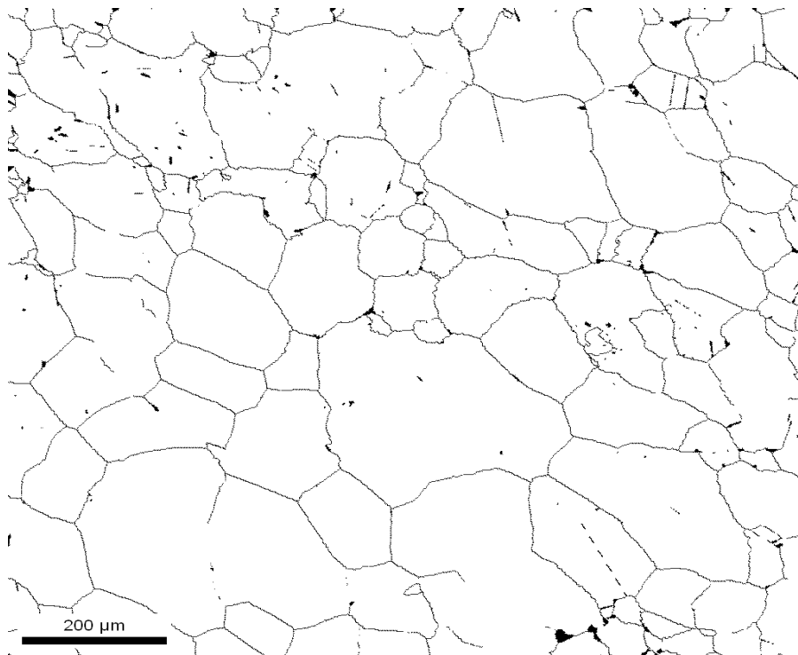
Fig. 4.102: Grain boundary character distribution of aged Alloy 617. (a) Dark lines are HAGBs and light grey lines are CSL boundaries; (b) HAGB network after removal of CSL boundaries
