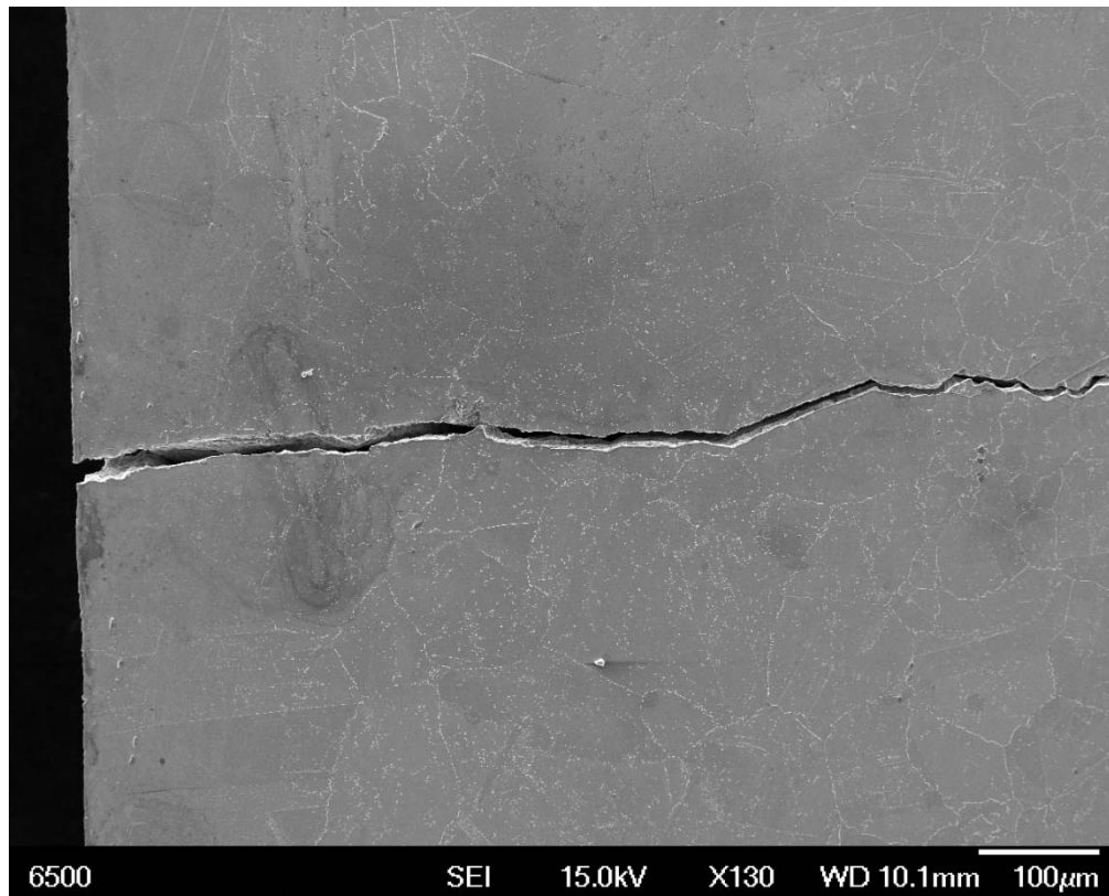
Fig. 4.86: Transgranular crack initiation and propagation in Alloy 617 during LCF tests. \epsilon_{tot} = 0.5\%
