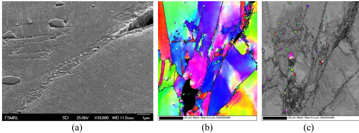
Fig. 4.6: DRX in the tensile test at 800°C: (a) SEM image of a grain boundary with a crack; (b) EBSD mapping showing the crystal orientations; (c) EBSD sampling of the inclusion particles ( M_{23}C_6 )
