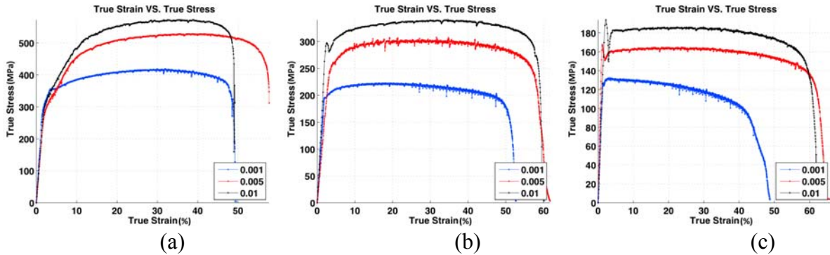
Fig. 4.22: True strain-stress curves for Alloy 617 at temperature: (a) 800°C; (b) 900°C; (c) 1000°C
