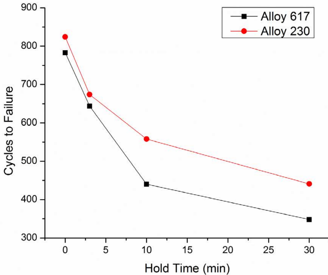
Fig. 4.71: Influence of hold time at peak tensile strain on the creep-fatigue life. \epsilon_{tot}=1.0\%
