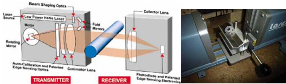
Fig. 3.20: Laser instrument used to measure the diameter change of the tube specimen. The resolution is 0.5\mu\text{m} [3.10]
