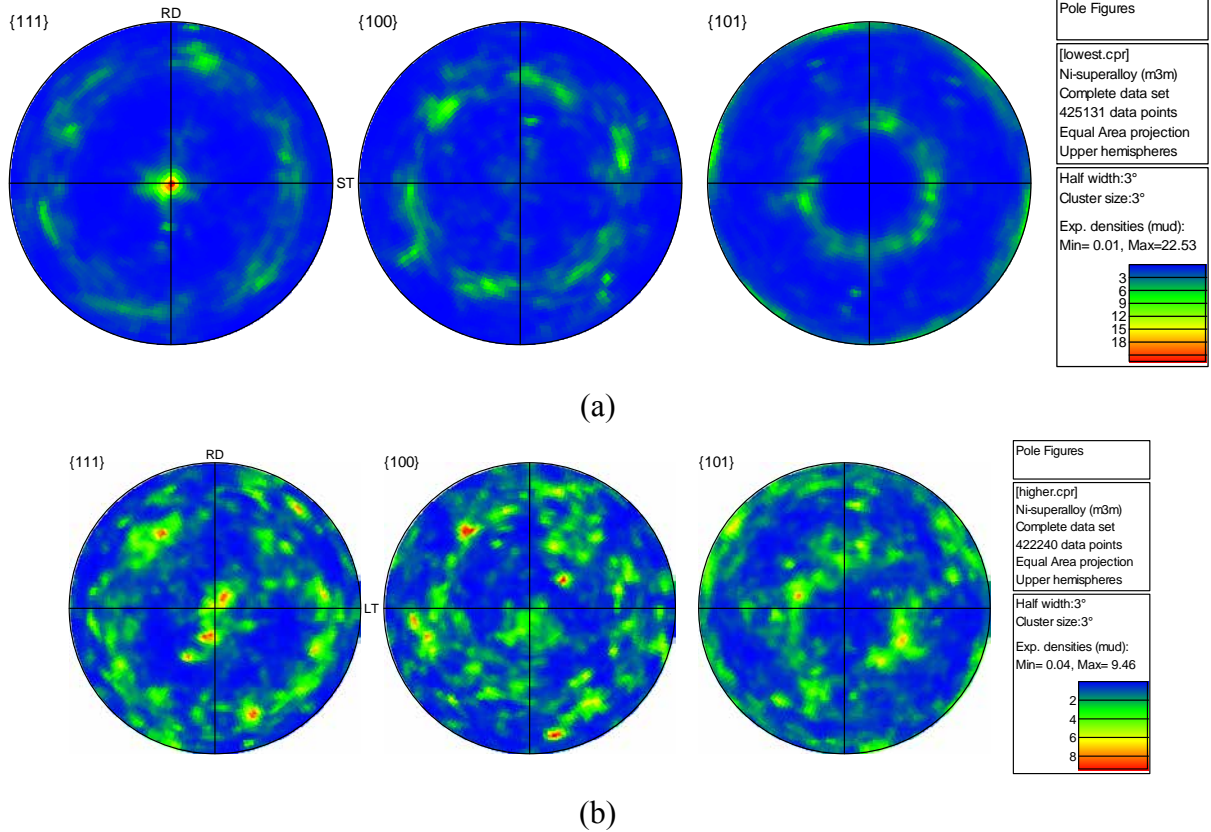
Fig. 4.16: Texture development after tensile testing at room temperature: (a) long-transverse direction; (b) short-transverse direction
