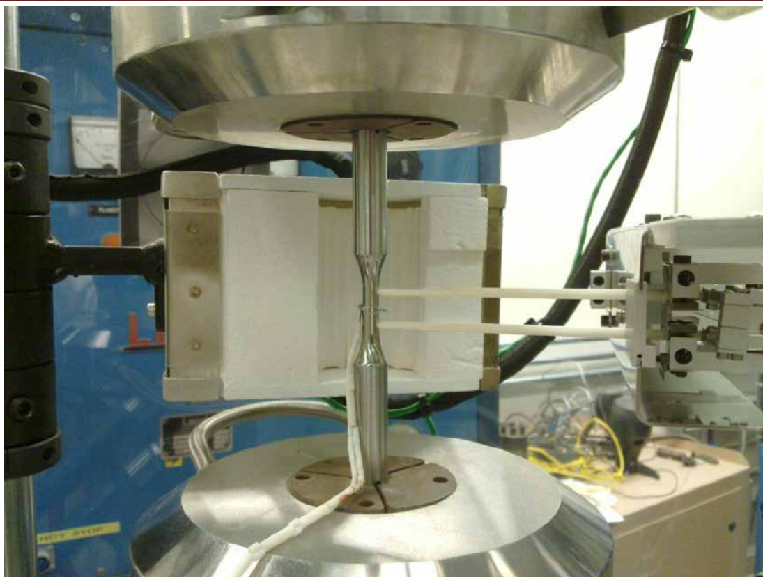
Fig. 3.17: A straight-sided specimen installed in the hydraulic grips with one S-type thermal couple and the high temperature extensometer installed
