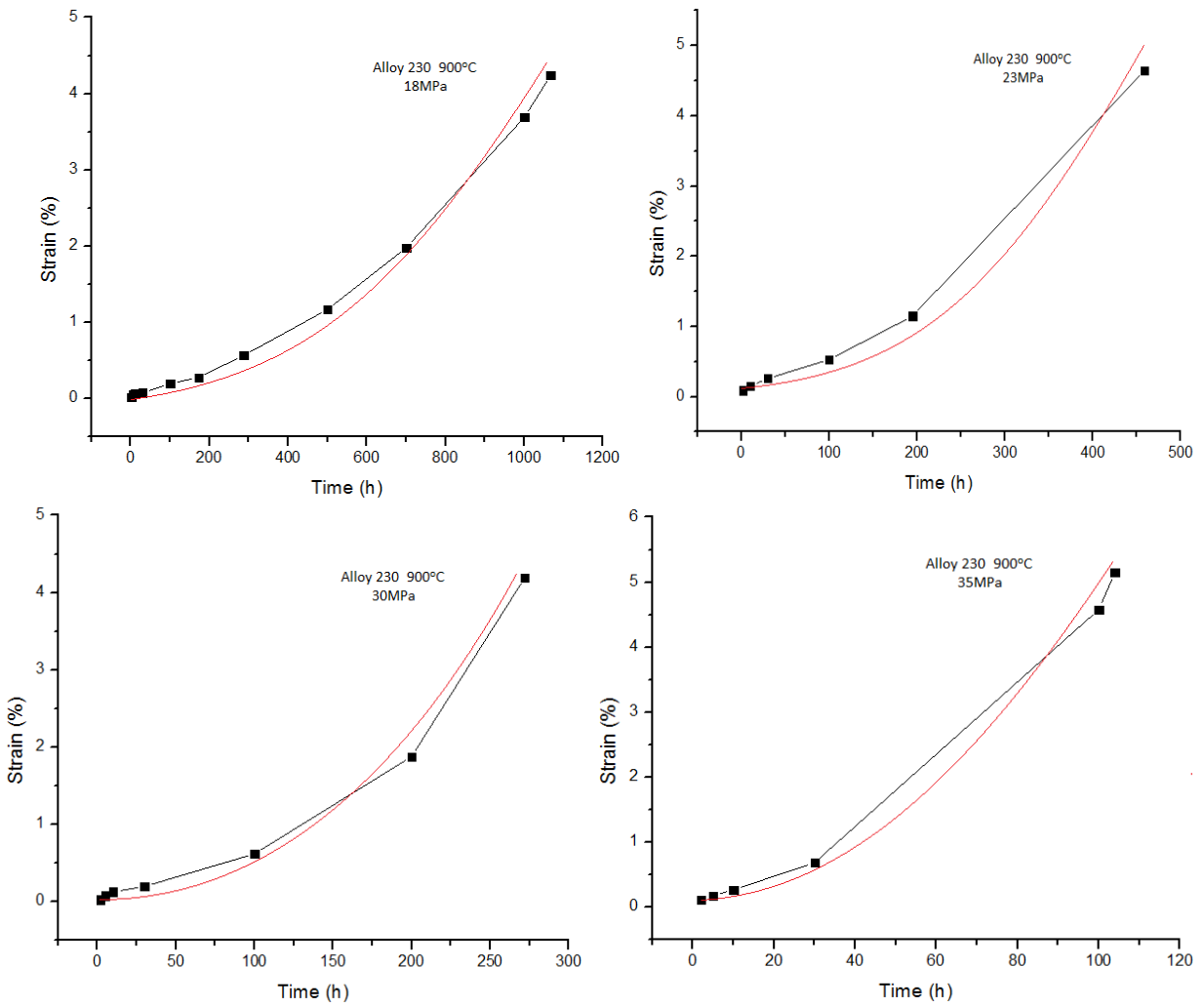
Fig. 4.129: (e) FEM simulation results for Alloy 230 at 900°C
