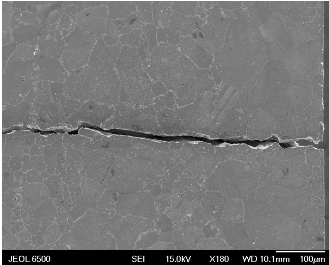
Fig. 4.90: Transgranular crack initiation and propagation in Alloy 230 during LCF tests. \epsilon_{tot} = 0.5\%
