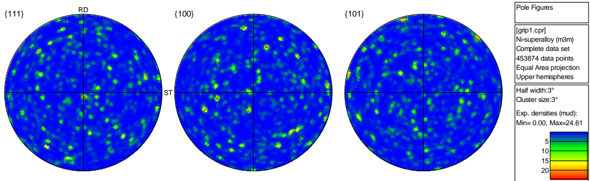
Fig. 4.13: Texture analysis for Alloy 617 in the as-received condition
