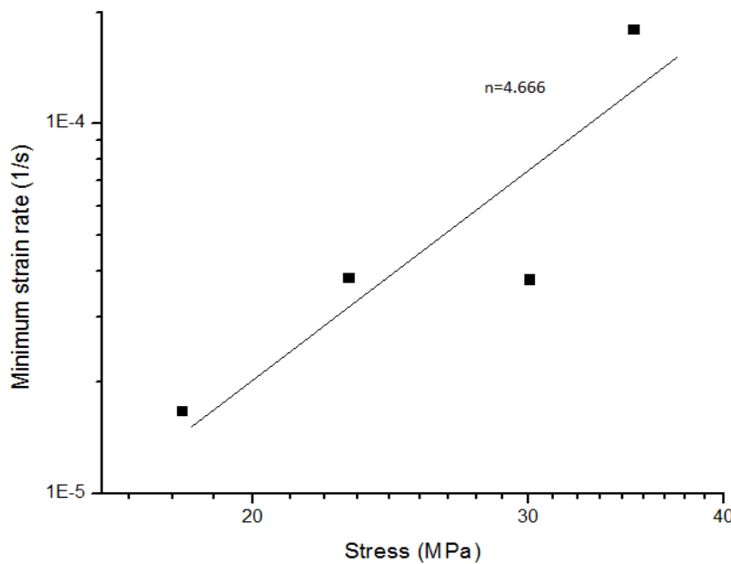
Fig. 5.13: Stress exponent analysis for Alloy 230 at 900°C
