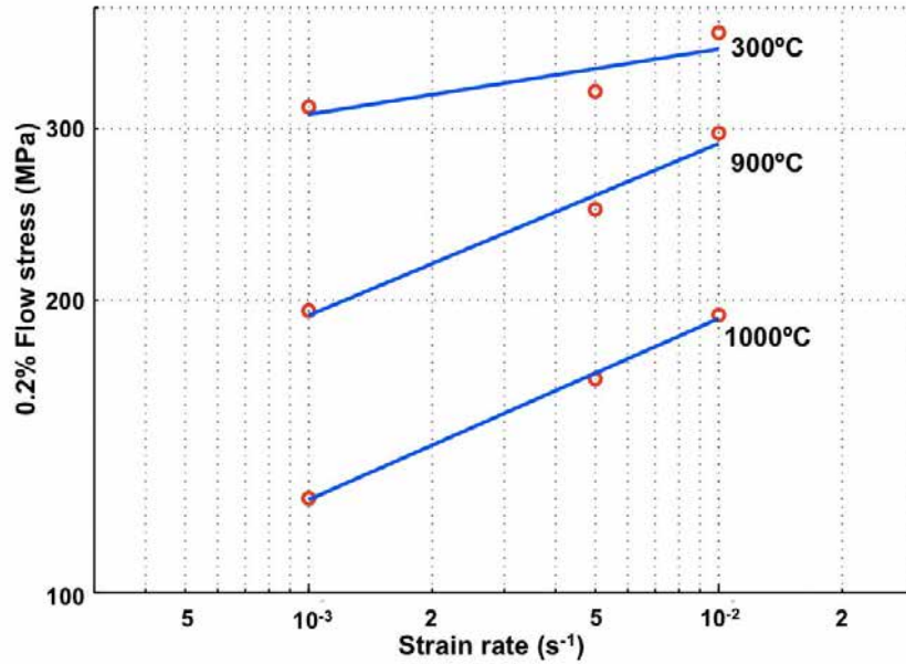
Fig. 4.21: 0.2% flow stress versus strain rate for Alloy 617.
