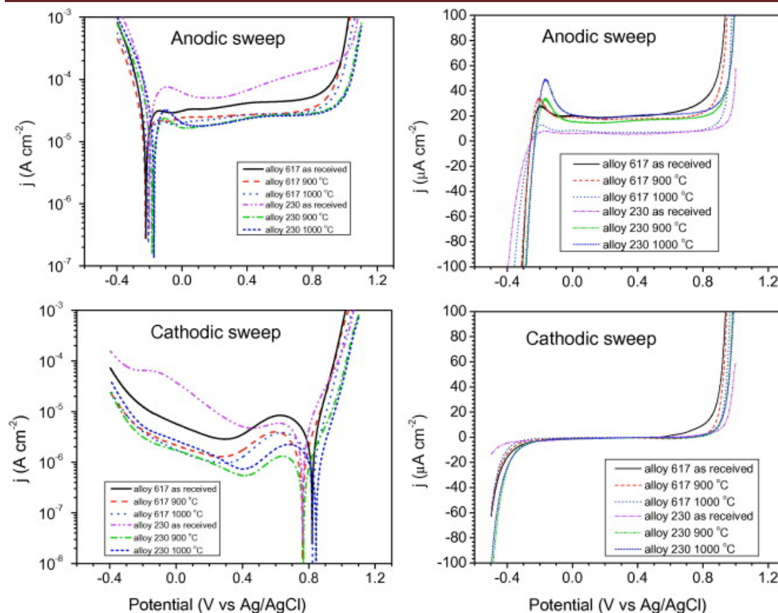
Fig. 4.138: Polarization curves of alloys in 0.1 M \text{H}_2\text{SO}_4 with 10 mV/s scan rate and 1000 rpm rotation rate. Current is in logarithmic scale on the left and linear scale on the right.
