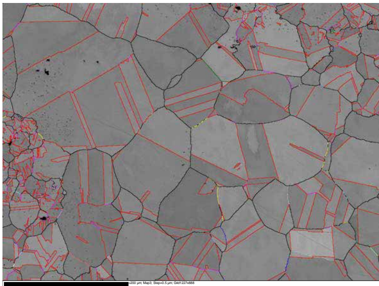
Fig. 4.39: EBSD and CSL boundary analysis for Alloy 617 aged at 900°C for 1000 hours
