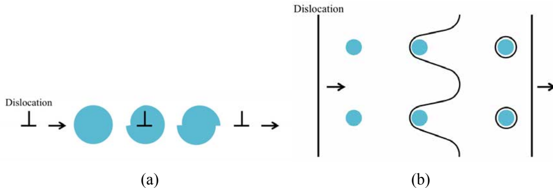
Fig. 4.27: Schematic representation of two strengthening mechanisms by dislocation-particle interaction: (a) particle cutting; (b) Orowan looping
