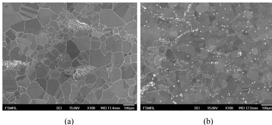
Fig. 3.25: Microstructure of the materials in the as-received condition: (a) Alloy 617; (b) Alloy 230
