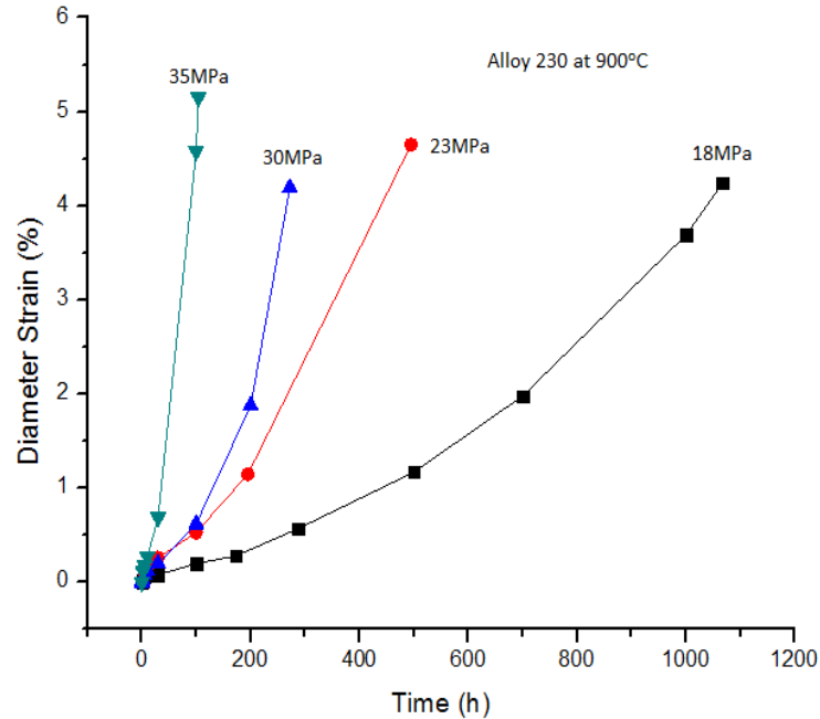
Fig. 4.121: Diameter strain vs. creep exposure time for Alloy 230 at 900°C
