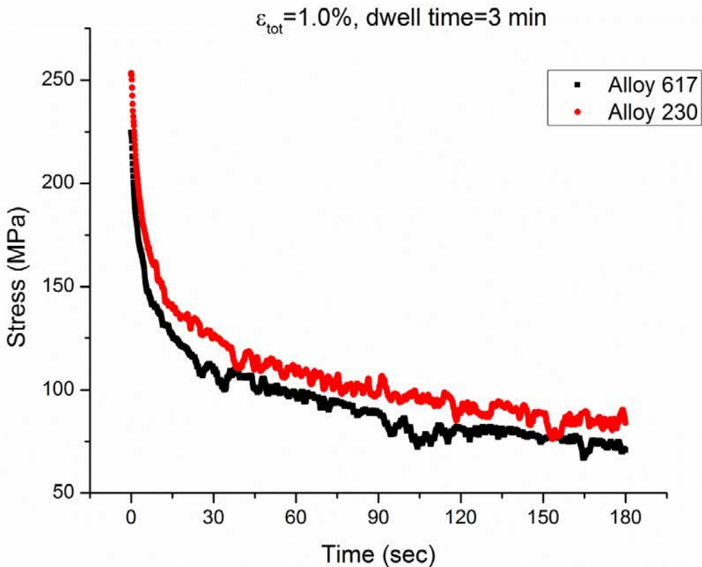
Fig. 4.74: Stress relaxation behavior during peak tensile strain hold period
