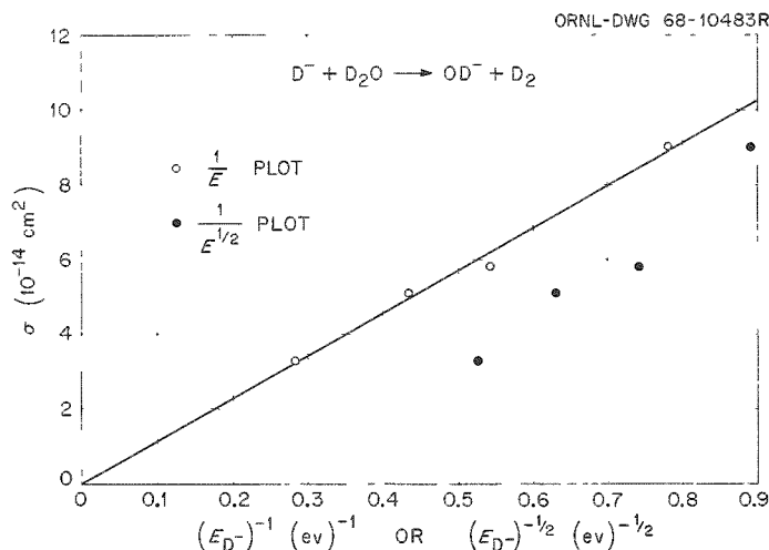
Fig. 17.11. Cross Section vs 1/E and (1/E)^{1/2} for the Reaction D^- + D_2O \rightarrow OD^- + D_2 .
