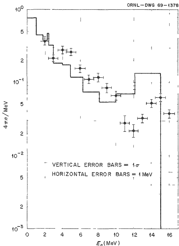
Fig. 21.1. Neutron Spectrum in Air at a Range of 215 m. Source height 500 ft, lateral distance 500 ft. Data normalized to 4\pi neutrons per Mev per source neutron. Compared with calculations at the same range (source height of 1125 ft).
