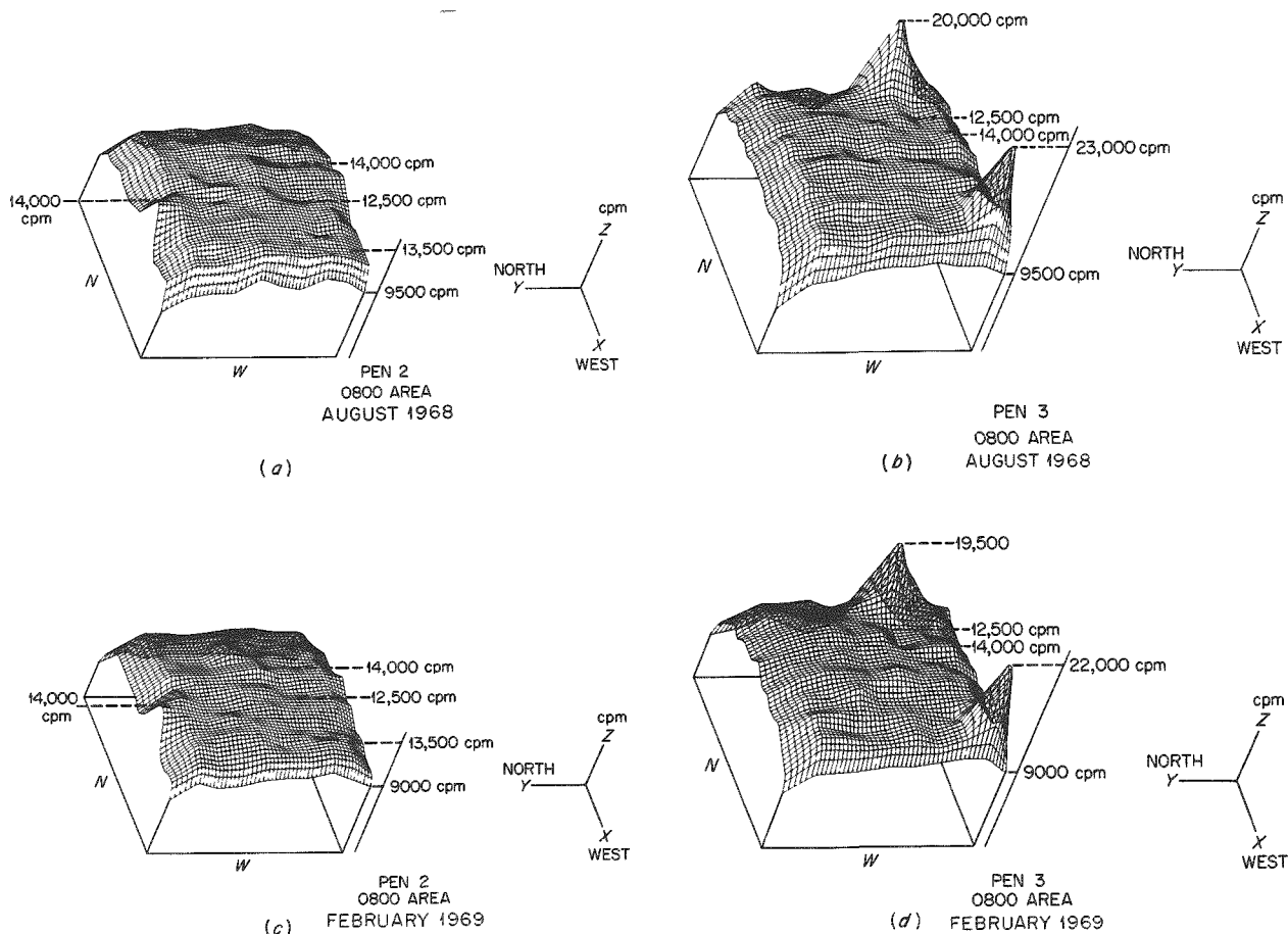
Fig. 8.2. Scans of Two of the Four Pens in the OCD Experimental Area (Ecology Area 0800) Contaminated with \sim 2 curies Each of ^{137}\text{Cs} -Tagged Fallout Simulant in August 1968. Pen 2 ( a,c ) shows the plane dose field typical of three of the four pens. Pen 3 ( b,d ) had two stoppages of the simulant spreader during tagging, resulting in the additional simulant represented by the two peaks shown. Scans made in August 1968 are shown in a and b ; scans of the same pens made during February 1969 are shown in c and d .
