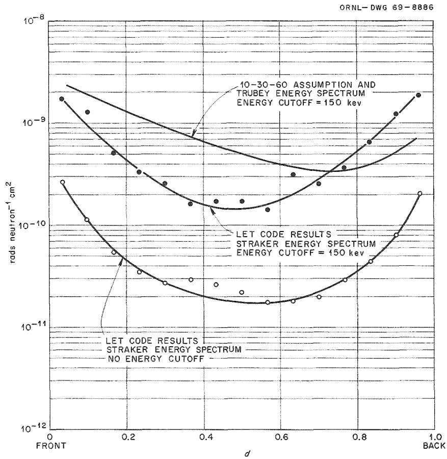
Fig. 20.20. Dose from Recoil Ions in a Cylindrical Phantom Filled with H 2 O (Height = 46 cm; Radius = 40 cm).
