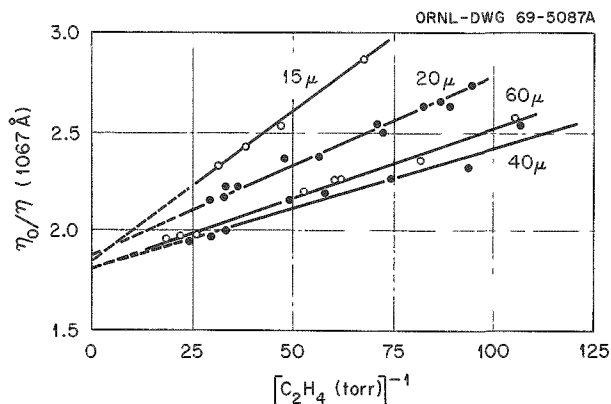
Fig. 16.12. Stern-Volmer Plot of Sensitized Ionization Efficiencies in Argon-Ethylene.
