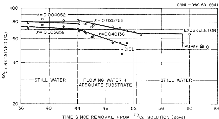
Fig. 11.17. Rates of Excretion of ^{60}\text{Co} by Two Hydropsychids as Affected by a Change in Environmental Conditions from Still Water with Inadequate Substrate to Flowing Water with Adequate Substrate.
