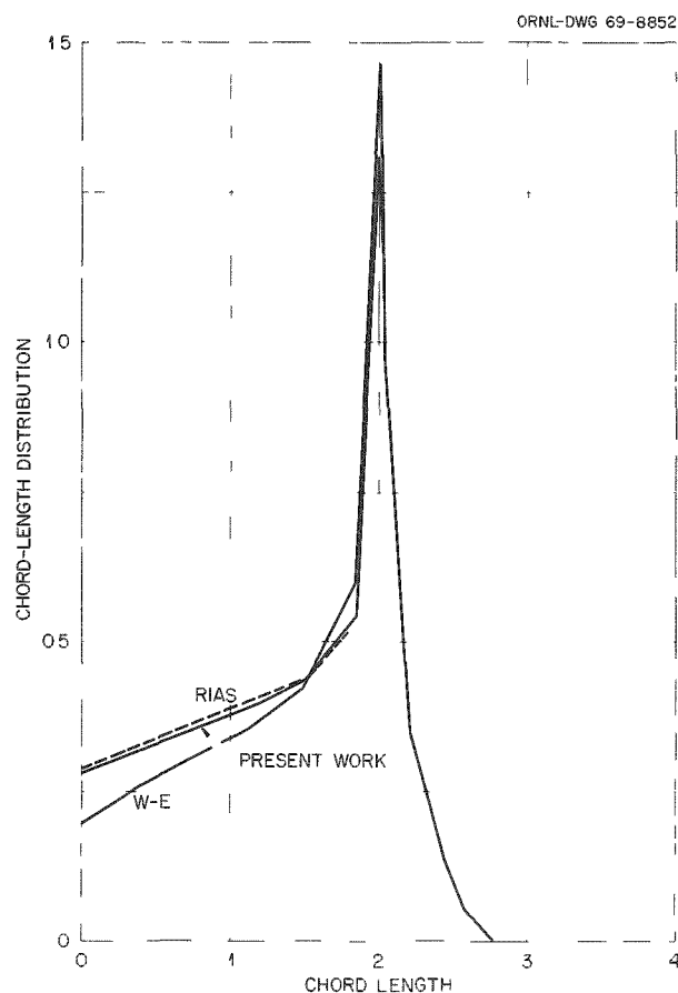
Fig. 14.4. Comparison of Chord-Length Distributions Obtained by Schwed and Ray (RIAS) and Wilson and Emery (W-E) with Present Work.
