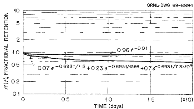
Fig. 24.6. A Plot of Maletskos et al. 's Power Function, 0.96t^{-0.01} , Together with a Sum of Three Exponential Terms for Approximating Total Body Retention of Thorium in Man.
