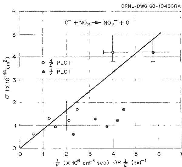
Fig. 17.12. Cross Section vs 1/E and 1/v for the Reaction O^- + NO_2 \rightarrow NO_2^- + O .
