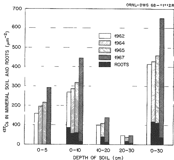
Fig. 10.6. Soil and Root Radiocesium Inside Tagged Plot of Tulip Poplar ( Liriodendron ) Forest from October 1962 to June 1967.
