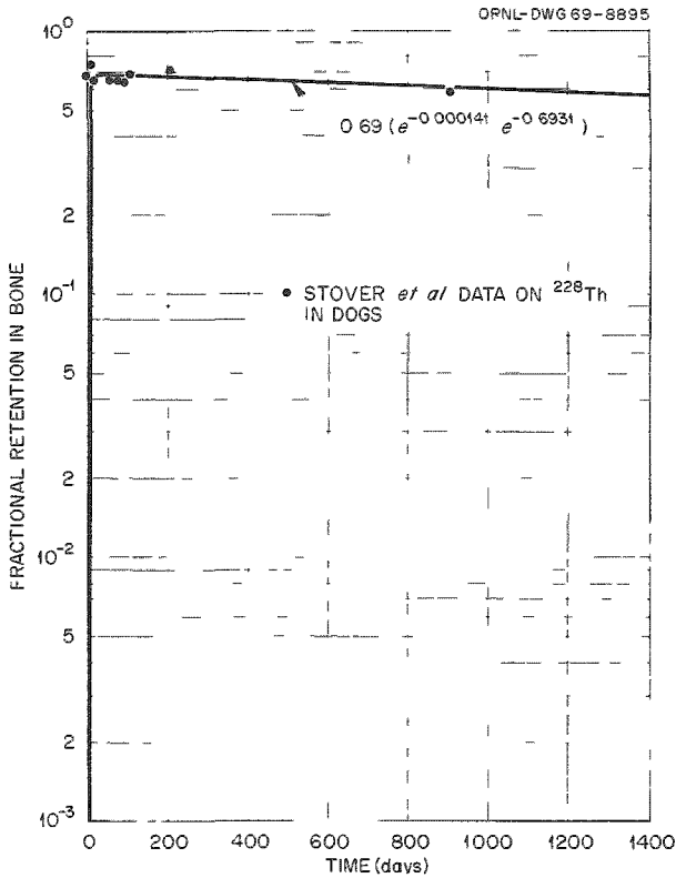
Fig. 24.7. Comparison of 228 Th Retention in Bone of Dogs with Estimate from a Lumped Four-Compartment Mammillary Model of Distribution of Thorium in the Dog Body.
