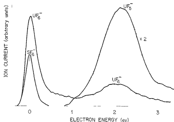
Fig. 17.8. Negative Ion Yields from a Mixture of UF_6 and SF_6 (~2:1) as a Function of Electron Energy.
