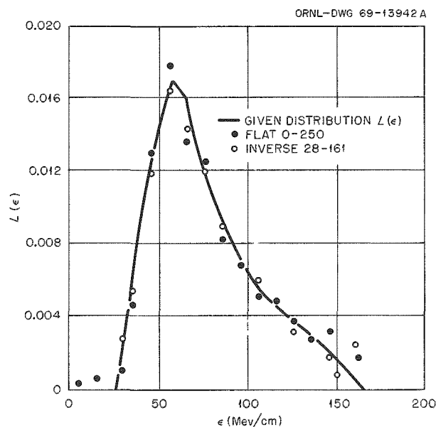
Fig. 14.7. Known Proton LET Spectrum (Solid Line) (Proton Energies 2 to 18 Mev). Unfolded spectra described in text (open and closed circles). The abscissa gives \epsilon in units of Mev/cm in a material of unit density (10 Mev/cm = 1 kev/ \mu ).
