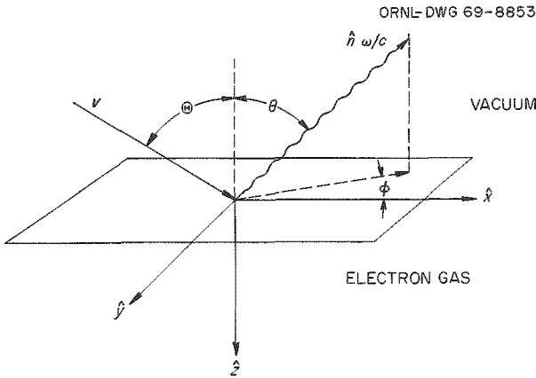
Fig. 14.8. Geometry of the BDFS Experiment. The velocity of the incident electron is v , and the propagation vector of the emitted photon is \hat{h}\omega/c , where \hat{h} is a unit vector and \omega is the angular frequency of the photon. The photon may be polarized either in the \hat{h}\hat{z} plane ( p polarization) or perpendicular to the \hat{h}\hat{z} plane ( s polarization). The region z > 0 is occupied by an electron gas, and the region z < 0 is a vacuum. The velocity v lies in the \hat{x}\hat{z} plane.
