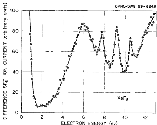
Fig. 17.4. Threshold Electron Impact Excitation Spectrum of Xenon Hexafluoride.
