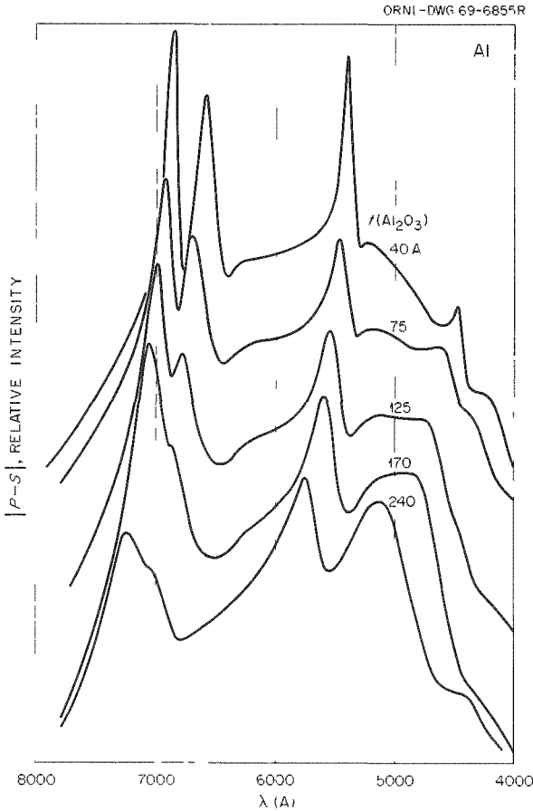
Fig. 15.20. Anomalous Peaks for Aluminized Grating Covered with Varying Thicknesses of \text{Al}_2\text{O}_3 , \theta = 25.7^\circ .
