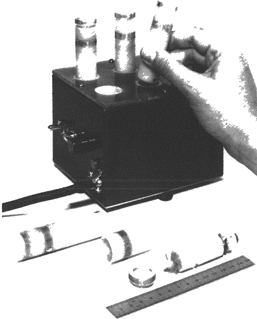
Fig. 22.33. Prototype of Personnel Dosimeters for Uranium Miners, Closed and Disassembled; Charging Unit in Background.
