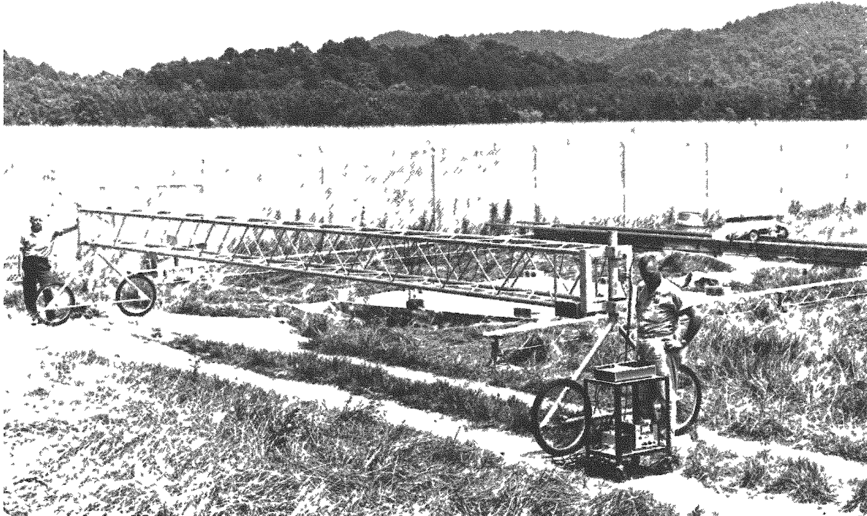
Fig. 8.1. View of OCD Plot Scanning Device. Scanner detector consists of a G-M tube mounted in a collimator so that signals are received from an area 1 m 2 at 1 m height. The G-M tube traverses the pen at a rate of 1 cm/sec, sending its signals to a modified rate meter and X-Y plotter.
