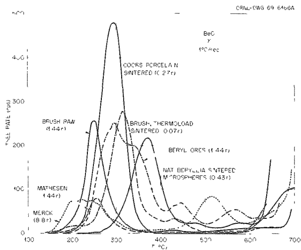
Fig. 22.16. TSEE Curves of Unsintered and Sintered BeO from Different Sources and with Different Impurity Content.
