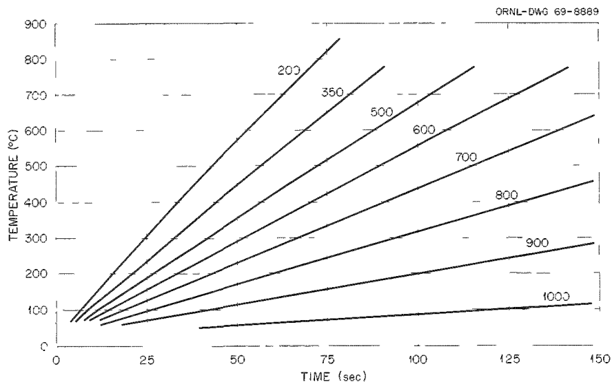
Fig. 21.11. Temperature as a Function of Time as Produced by the Linear Temperature Controller.
