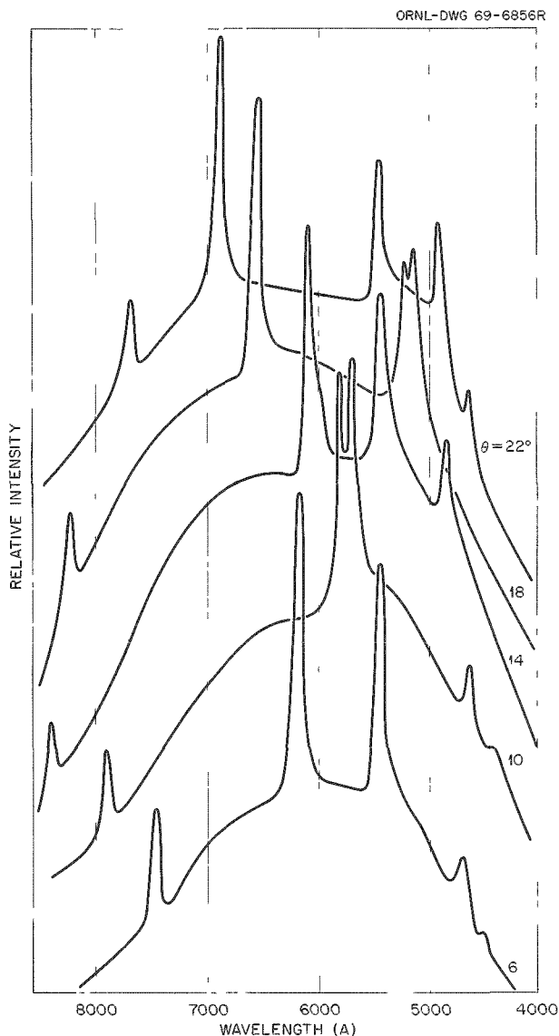
Fig. 15.17. Tungsten Emission Spectra Showing Anomalies in the p -Polarized Component from a Silver-Coated Diffraction Grating. The half-angle between source and detector is denoted by \theta .
