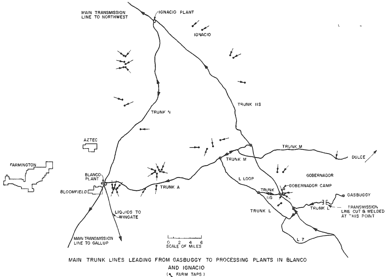
Fig. 6.2 Simplified Schematic of the Gas Collection System in the San Juan Division of El Paso Natural Gas Company.
