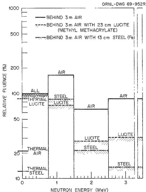
Fig. 23.1. Health Physics Research Reactor (HPRR) Neutron Fluence Spectra.
