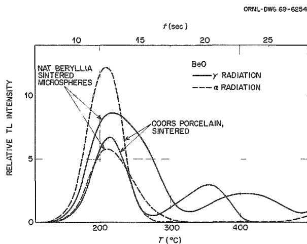
Fig. 22.21. TL Glow-Curves of Two Sintered BeO Samples After Exposure to Alpha and Gamma Radiation.
