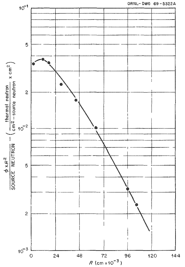
Fig. 20.22. Thermal-Neutron Distribution Along the Air-Ground Interface for Distances to 3500 ft from a Point 14-Mev Neutron Source Operating 54 ft Above Ground.
