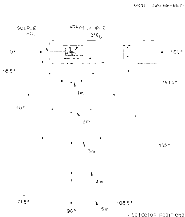
Fig. 20.2. Location of Detectors Used in the Measurement of Radiations from the Small Boy Viewed Looking Down on a Horizontal Plane 1 m from the Floor.
