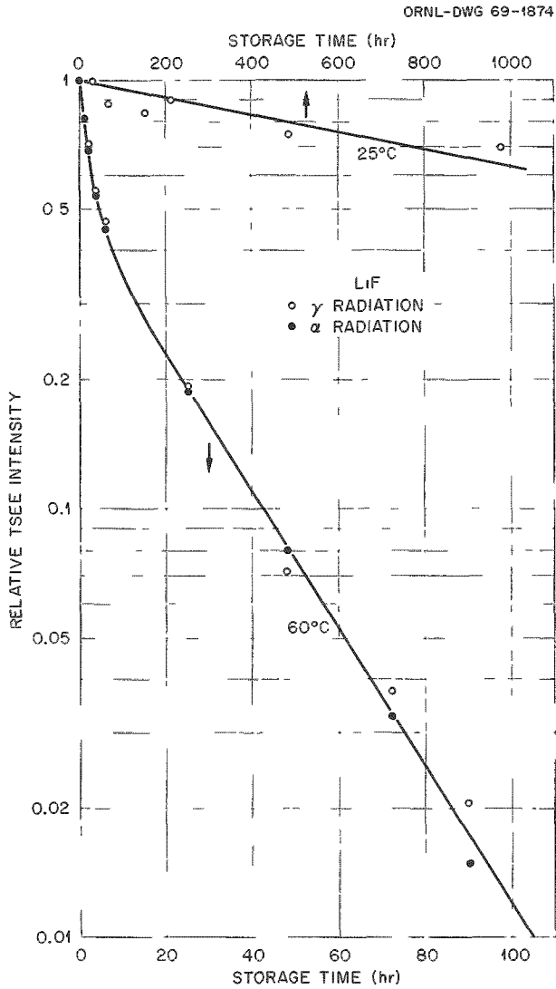
Fig. 22.6. Fading of the \sim 150^\circ\text{C} TSEE Peak in LiF (Baker) After Alpha and Gamma Irradiation at Different Storage Temperatures in Unmodified Laboratory Atmosphere.
