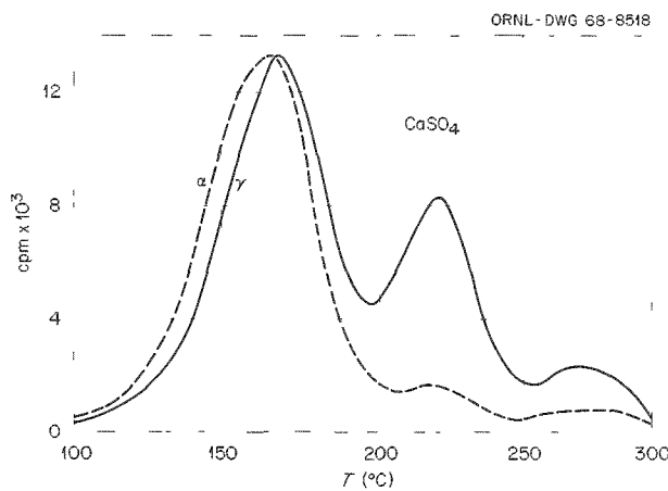
Fig. 22.3. TSEE Curve During Nonlinear Heating of \text{CaSO}_4 (Baker, Prefired 1 hr at 950^\circ\text{C} ) After Exposure to ^{239}\text{Pu} Alpha and ^{60}\text{Co} Gamma Radiation.
