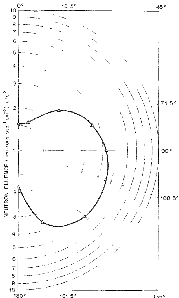
Fig. 20.9. Small Boy Neutron Fluence at 2 m (Determined by the Long Counter) as a Function of Angle.
