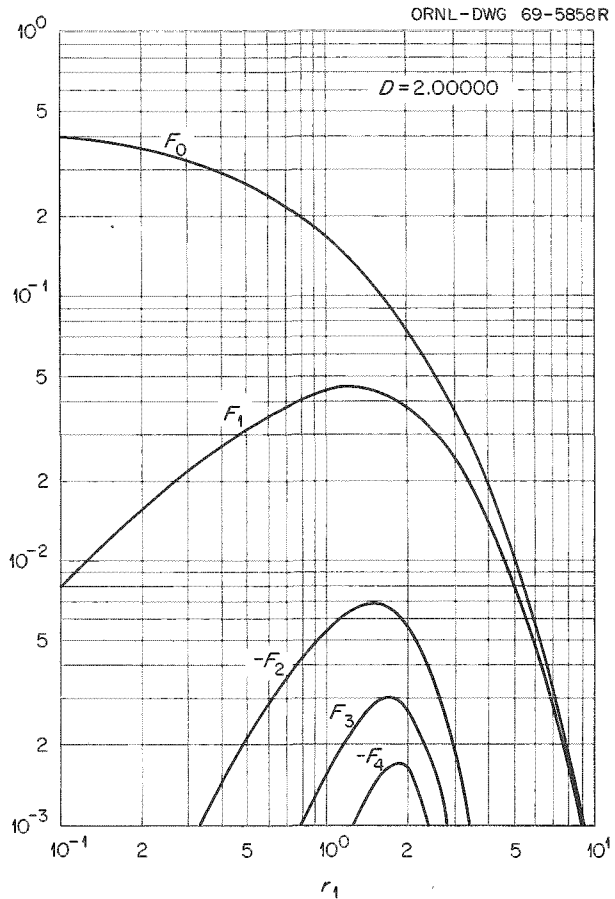
Fig. 14.14. Radial Functions F_l(r_1) for D = 2 .
