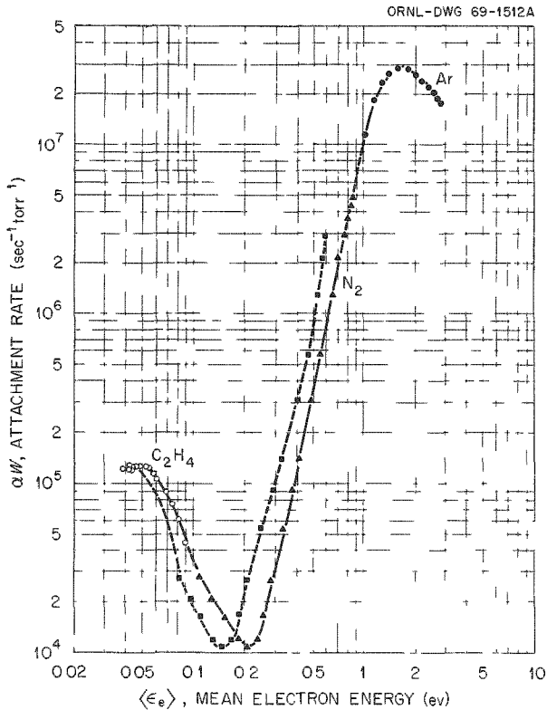
Fig. 16.2. Attachment Rate \alpha_w as a Function of Mean Electron Energy \langle \epsilon_e \rangle for p -Benzoquinone: Comparison of Carrier Gases. ■, Carleton and Megill, 12 ▲, Engelhardt et al 13
