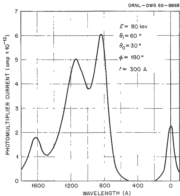
Fig. 15.16. Emission Spectrum from Aluminum Film 300 A in Thickness Bombarded by 1.0 \mu of 80-kev Electrons.
