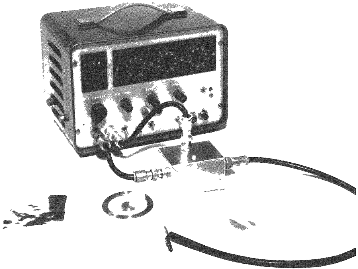
Fig. 22.29. Automatic Flying-Spark Alpha-Particle Track Counter with Portable High-Voltage Supply and Scaler.
