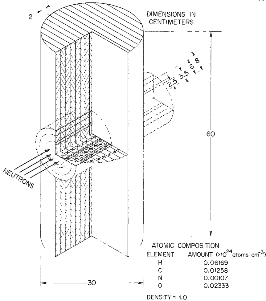
Fig. 20.11. Phantom for Study of D and DE Due to a Collimated Beam of Neutrons.
