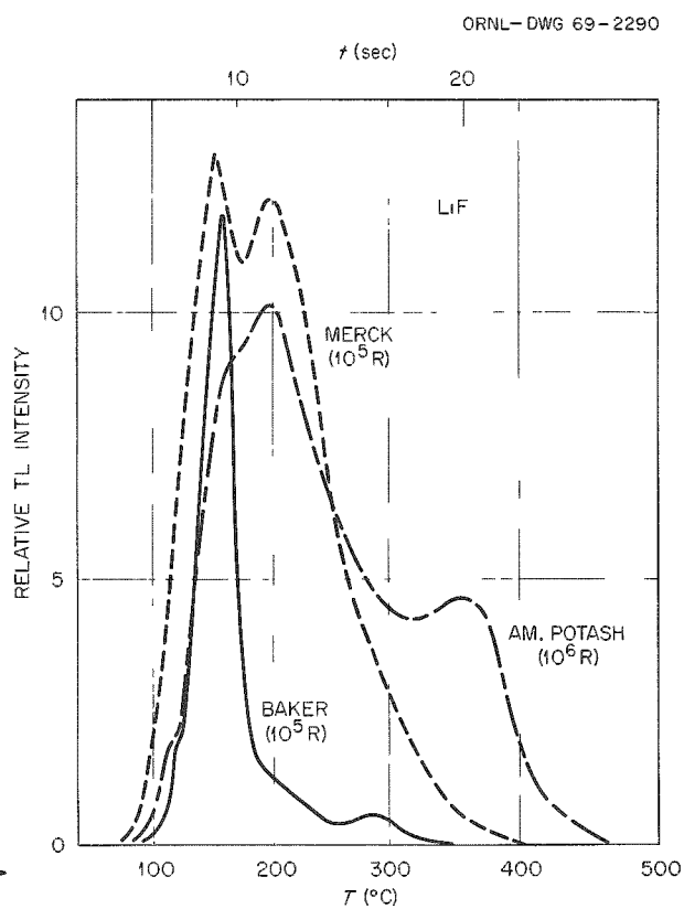
Fig. 22.15. Thermoluminescence (TL) Glow Curves of Different Analytical-Grade (Unactivated) Lithium Fluorides After Exposure to Gamma Radiation.
