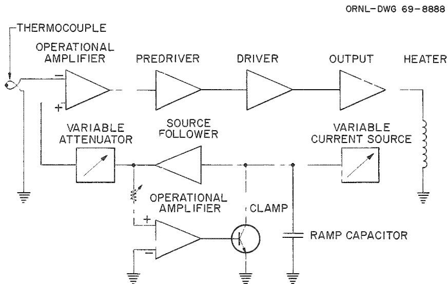
Fig. 21.10. Temperature Controller Block Diagram.
