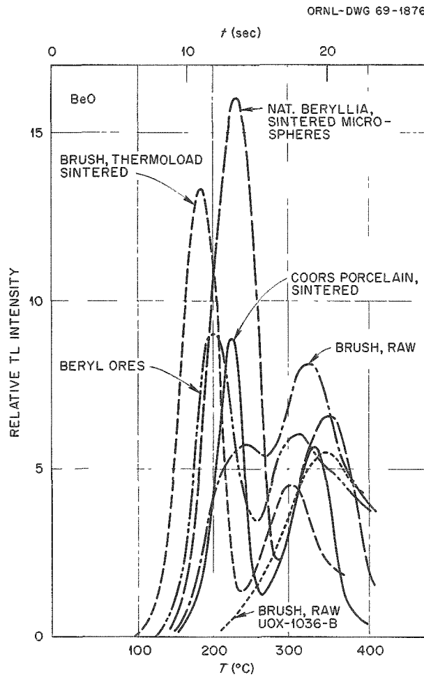
Fig. 22.17. TL Glow-Curves of Different Gamma-Irradiated BeO Samples.
