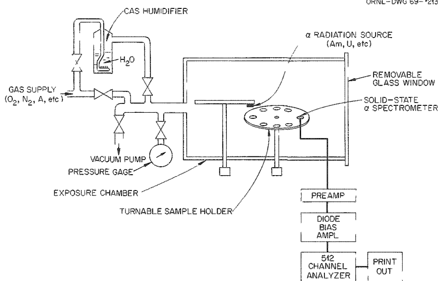
Fig. 22.25. Schematic Diagram of Exposure Chamber for Studies of the Environmental Effect on Foil Sensitivities.
