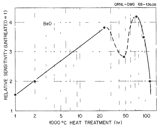
Fig. 22.10. TSEE Sensitivity of the Low-Temperature ( \sim 250^\circ\text{C} ) Peak in a Sintered \text{BeO} (Brush) as a Function of Storage Time at 1000^\circ\text{C} .
