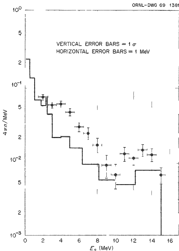
Fig. 21.2. Neutron Spectrum in Air at a Range of 766 m. Source height 1125 ft lateral distance 2250 ft Data normalized to 4\pi neutrons per Mev per source neutron Compared with calculations for the same conditions
