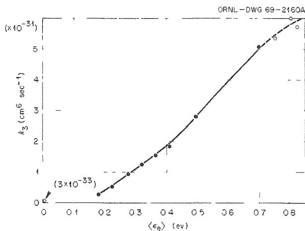
Fig. 16.9. Three-Body Electron Attachment Rate Coefficient for \text{N}_2\text{O}-\text{N}_2 Mixtures vs \langle \epsilon_e \rangle .
