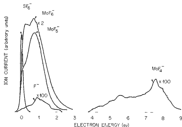
Fig. 17.7. Negative Ion Yields from Molybdenum Hexafluoride as a Function of Electron Energy.
