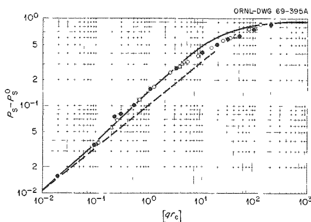
Fig. 16.11. Geminate Scavenging Probabilities as a Function of Scavenger Concentration. Experimental points: closed circles, CH_3Br ; open circles, C_2H_5Br ; triangles, CH_3Cl ; solid line, present theory.
