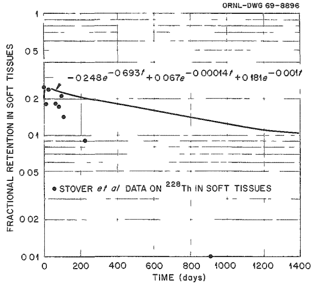
Fig. 24.8. Comparison of 228 Th Retention in Soft Tissues of Dogs with Estimate from a Four-Compartment Mammillary Model of Distribution of Thorium in Dog Body.
