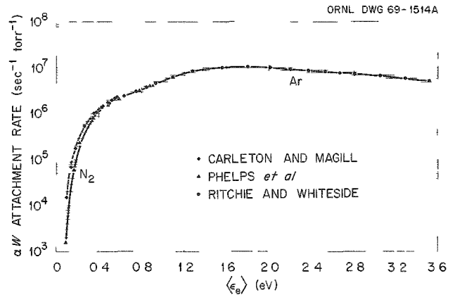
Fig. 16.3. Variation of the Attachment Rate for the Formation of O^- from N_2O with \langle \epsilon_e \rangle .
