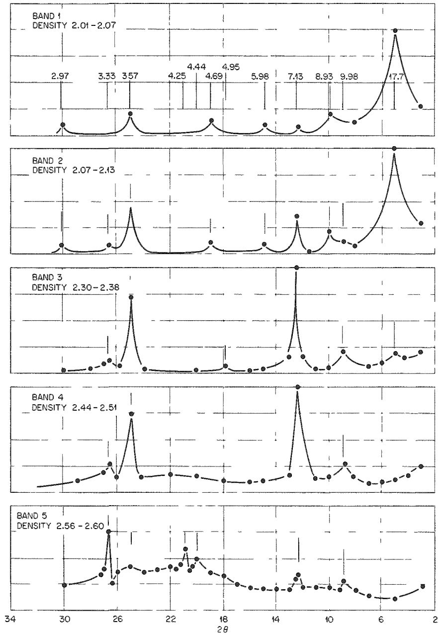
Fig. 1.3. Smoothed X-Ray Diffraction Tracings of Magnesium-Saturated Glycerol-Solvated Clays (Less than 2 \mu ) from Recovered Bands.
