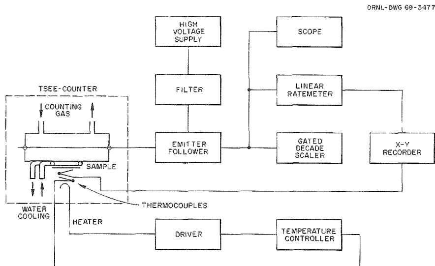
Fig. 22.2. Block Diagram of TSEE Reader.
